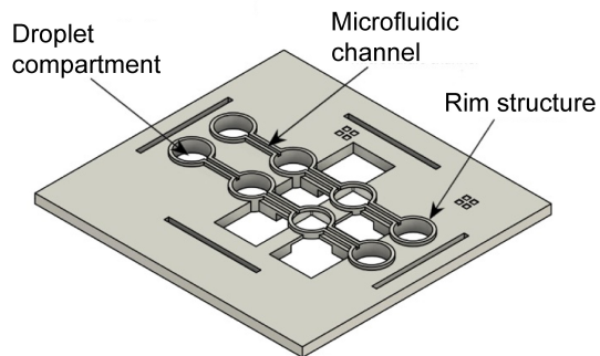
Isometric projected view:
