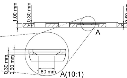
Side view of section BB':
