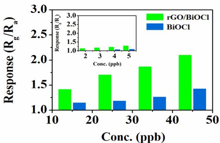
Fig.S2 Effect of \text{NO}_2 concentration on response of BiOCl and rGO/BiOCl based fabricated sensor.
