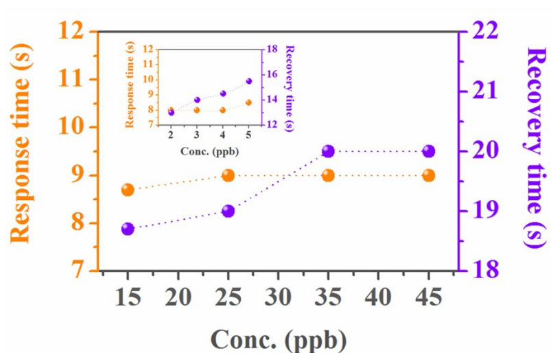
Fig.S1 Response/recovery times of each concentration stages.
