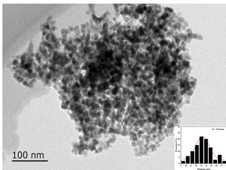
Fig.S4 Co/C-500 Particle Size Distribution Map
