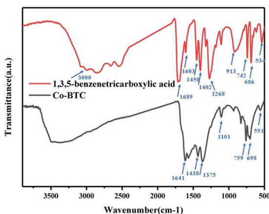
Fig. S1 FT-IR spectra of Co-BTC and 1,3,5-H 3 BTC.
