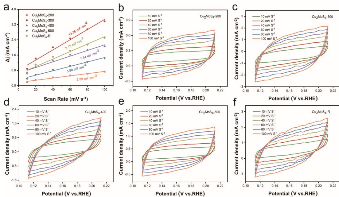
Fig. S12 (a) Double layer capacitance curves of catalysts in 1 M PBS; (b-f) Cyclic voltammetry curves of different catalysts at different scan rates.
