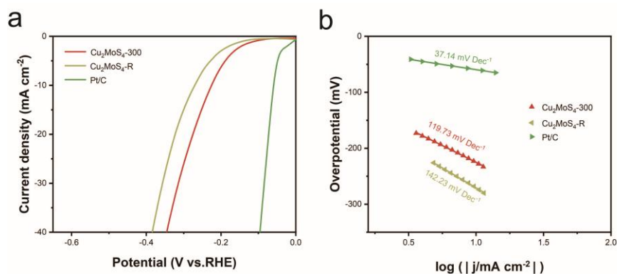
Fig. S13 (a) HER polarization curves of \text{Cu}_2\text{MoS}_4 -300, \text{Cu}_2\text{MoS}_4 -R and Pt/C in 1 M KOH; (b) Corresponding Tafel curves of the samples in 1 M KOH.
