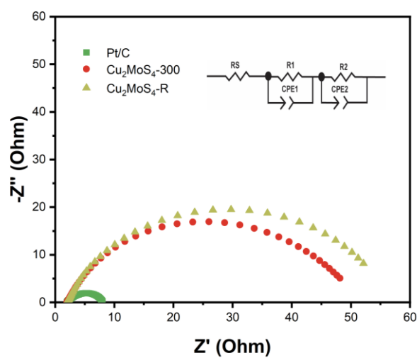
Fig. S8 EIS spectrum of \text{Cu}_2\text{MoS}_4 -300 in 0.5 M \text{H}_2\text{SO}_4 .
