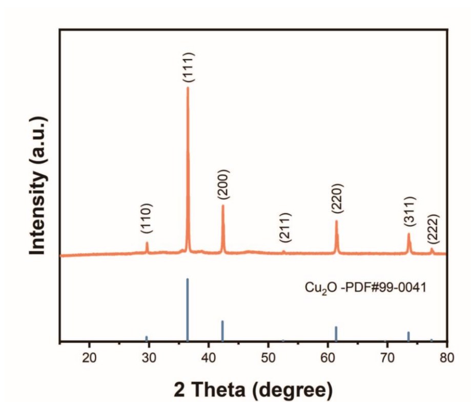
Fig. S5 XRD pattern of the resulting sample without EBI irradiation.
