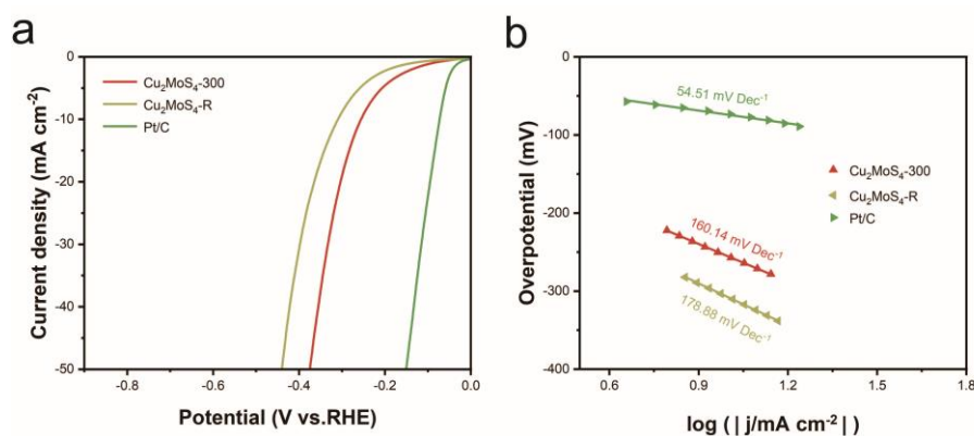
Fig. S10 (a) HER polarization curves of \text{Cu}_2\text{MoS}_4 -300, \text{Cu}_2\text{MoS}_4 -R and Pt/C in 1 M PBS; (b) Corresponding Tafel curves of samples in 1 M PBS.
