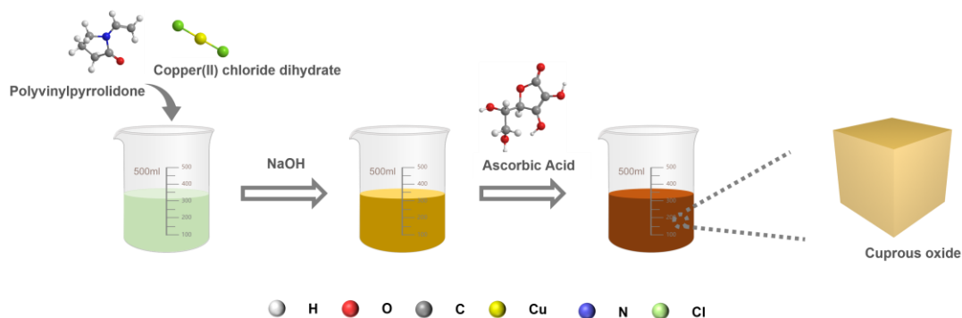
Fig. S1 Schematic diagram of hydrothermal synthesis of Cu 2 O nanocubes.
