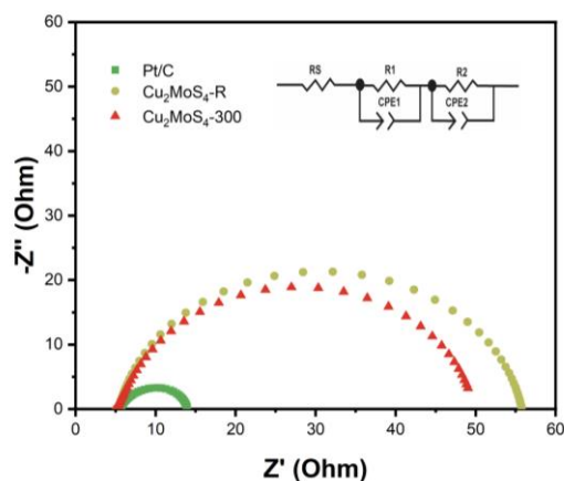
Fig. S14 EIS spectrum of the as-synthesized \text{Cu}_2\text{MoS}_4 -300 nanocubes in 1 M KOH.
