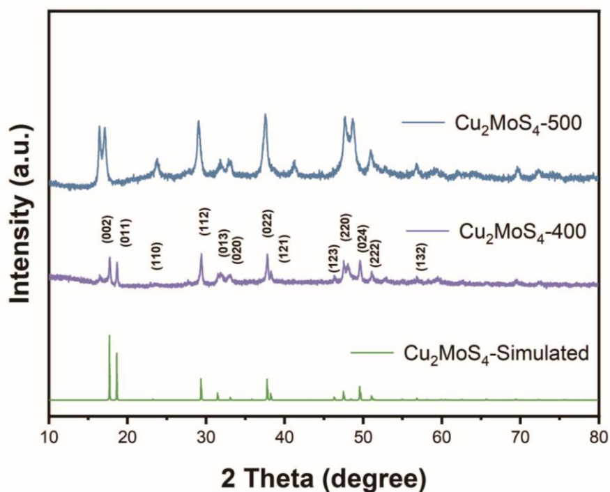
Fig. S3 XRD patterns of the \text{Cu}_2\text{MoS}_4\text{-400} and \text{Cu}_2\text{MoS}_4\text{-500} samples.
