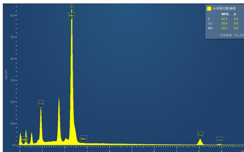
Fig. S6 Energy dispersive X-ray spectrum of the \text{Cu}_2\text{MoS}_4 -300 nanocubes.
