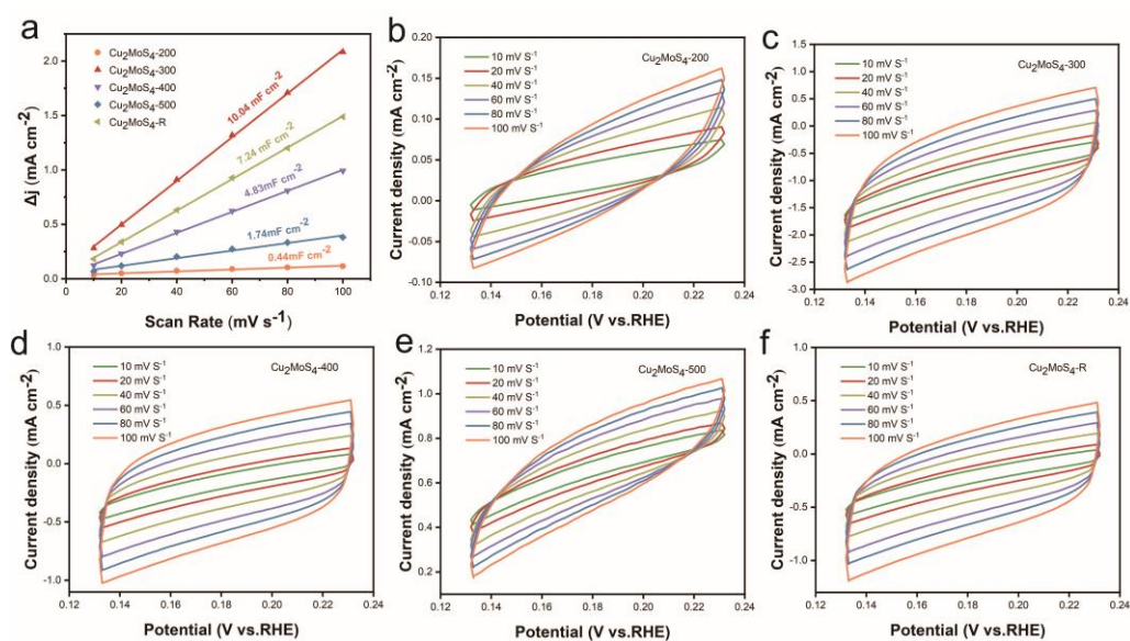
Fig. S15 (a) Double layer capacitance curves of \text{Cu}_2\text{MoS}_4 -related catalysts in 1 M KOH; (b-f) Cyclic voltammetry curves at different scan rates.
