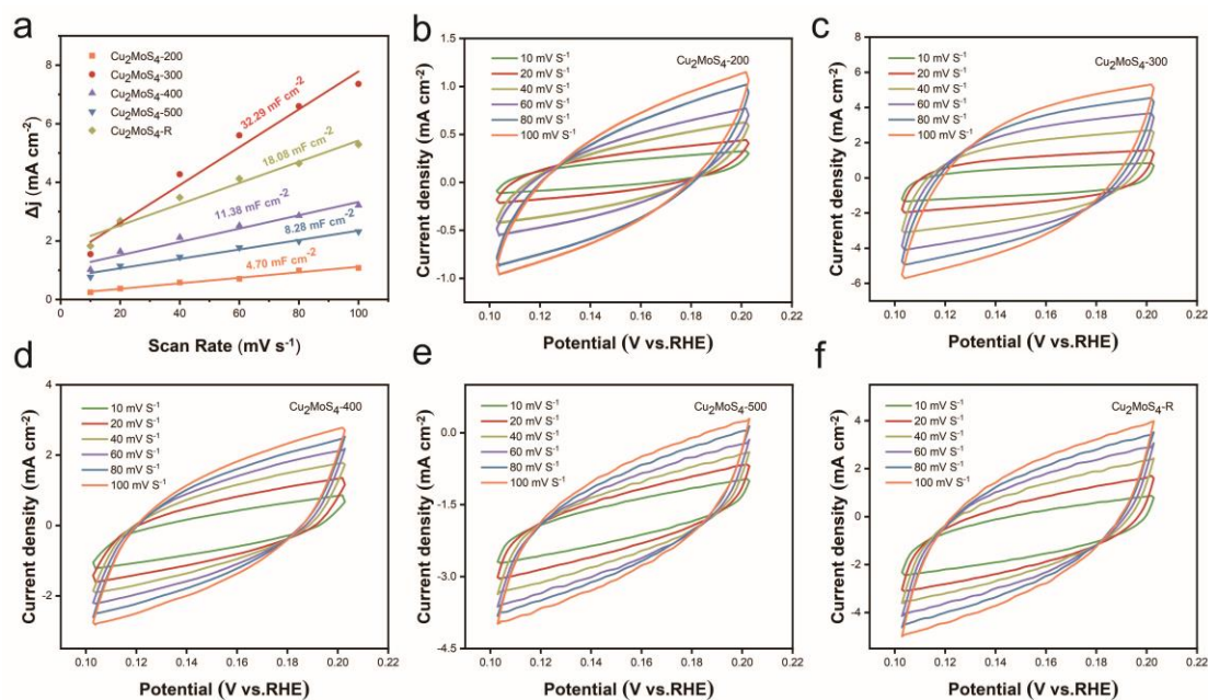
Fig. S9 (a) Double layer capacitance curves of different catalysts in 0.5 M \text{H}_2\text{SO}_4 ; (b-f) Cyclic voltammograms of the catalysts at different scan rates.
