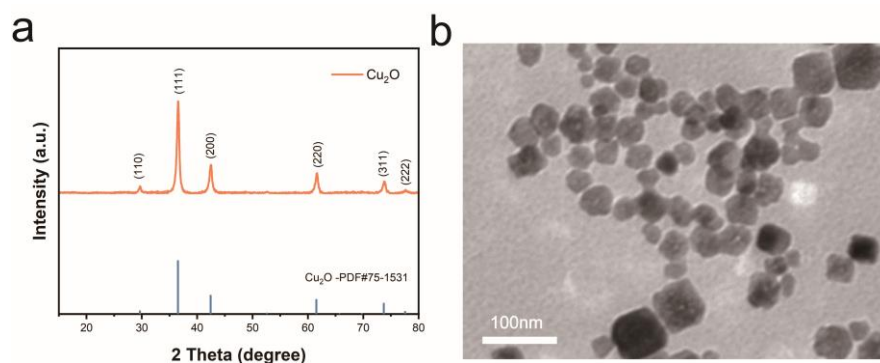
Fig. S2 XRD pattern (a) and TEM image (b) of the Cu 2 O nanocubes.
