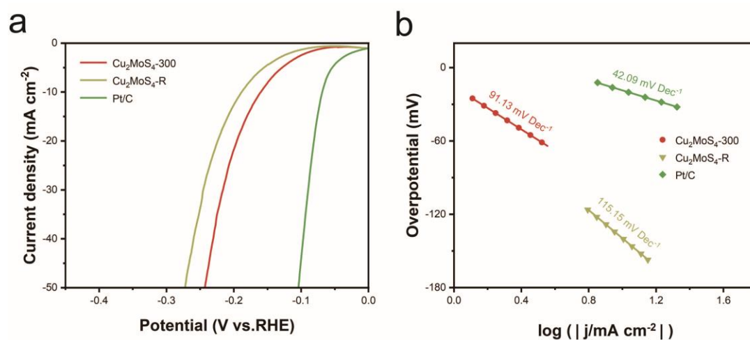
Fig. S7 (a) HER polarization curves of \text{Cu}_2\text{MoS}_4 -300, \text{Cu}_2\text{MoS}_4 -R and Pt/C in 0.5 M \text{H}_2\text{SO}_4 ; (b) Corresponding Tafel curves.
