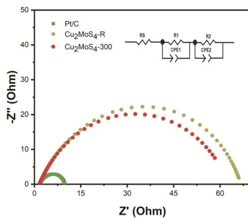
Fig. S11 EIS spectra of \text{Cu}_2\text{MoS}_4 -300 in 1 M PBS.
