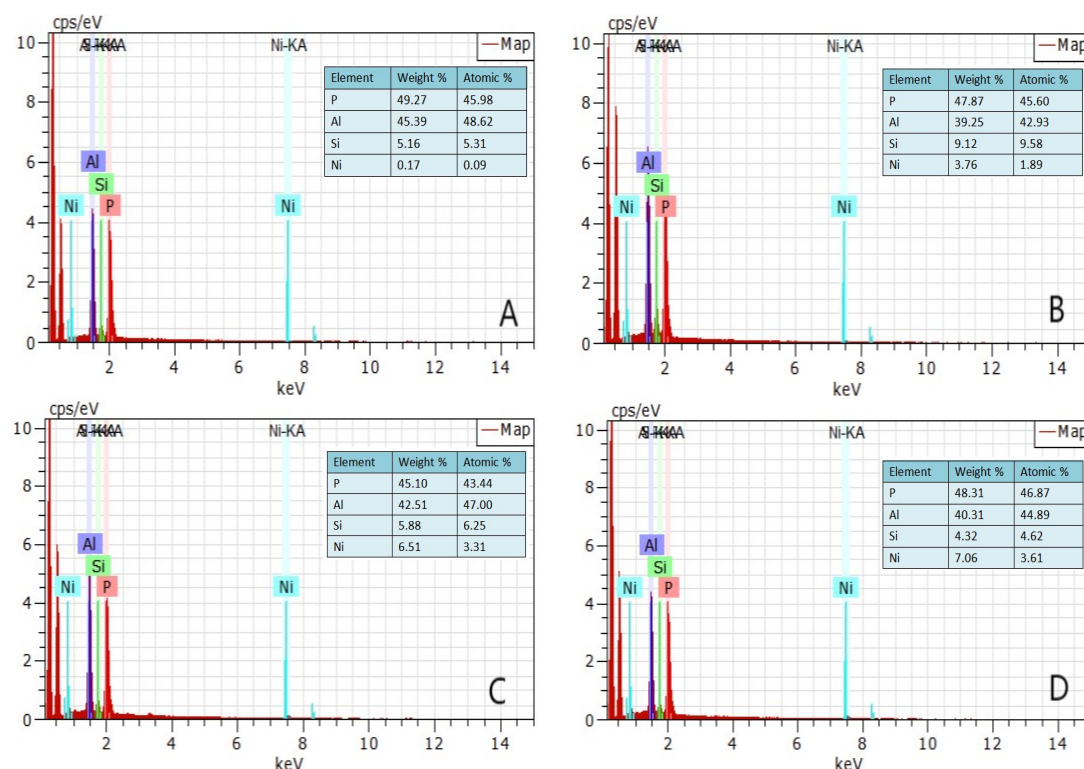
Fig. S1 Mapping and EDS of Ni/SAPO-11 catalysts (A: NiS11-N1; B: NiS11; C: NiS11-N3; D: NiS11-N4) with different Ni/Al ratios.
