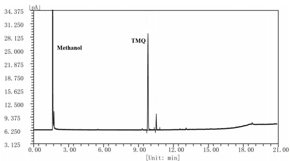
Figure 3. Chromatogram under optimal conditions
