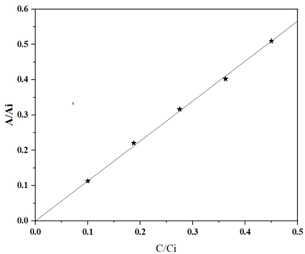
Figure 1. Calibration curve of TMP.
