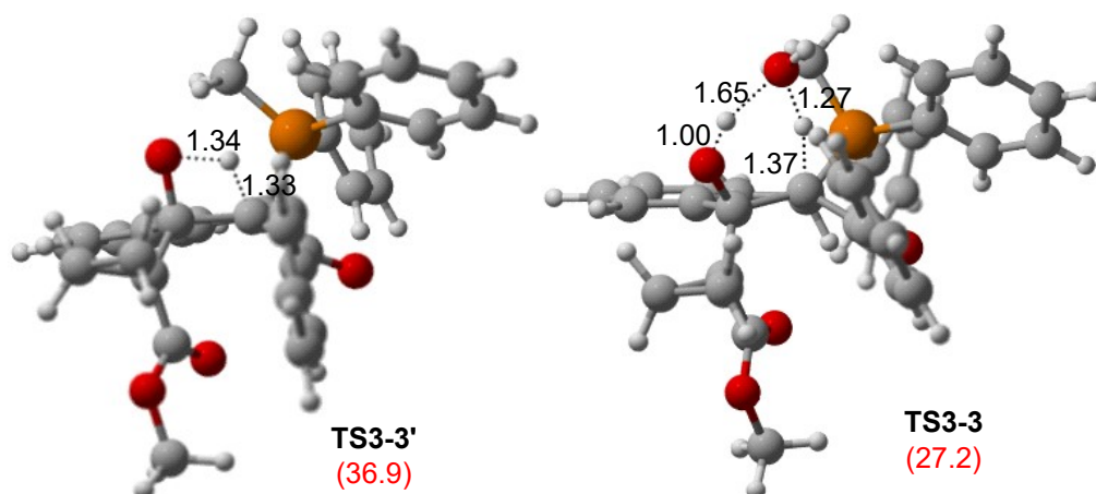
Fig. S1 Structures and energy barriers for the [1,3]-proton transfer
