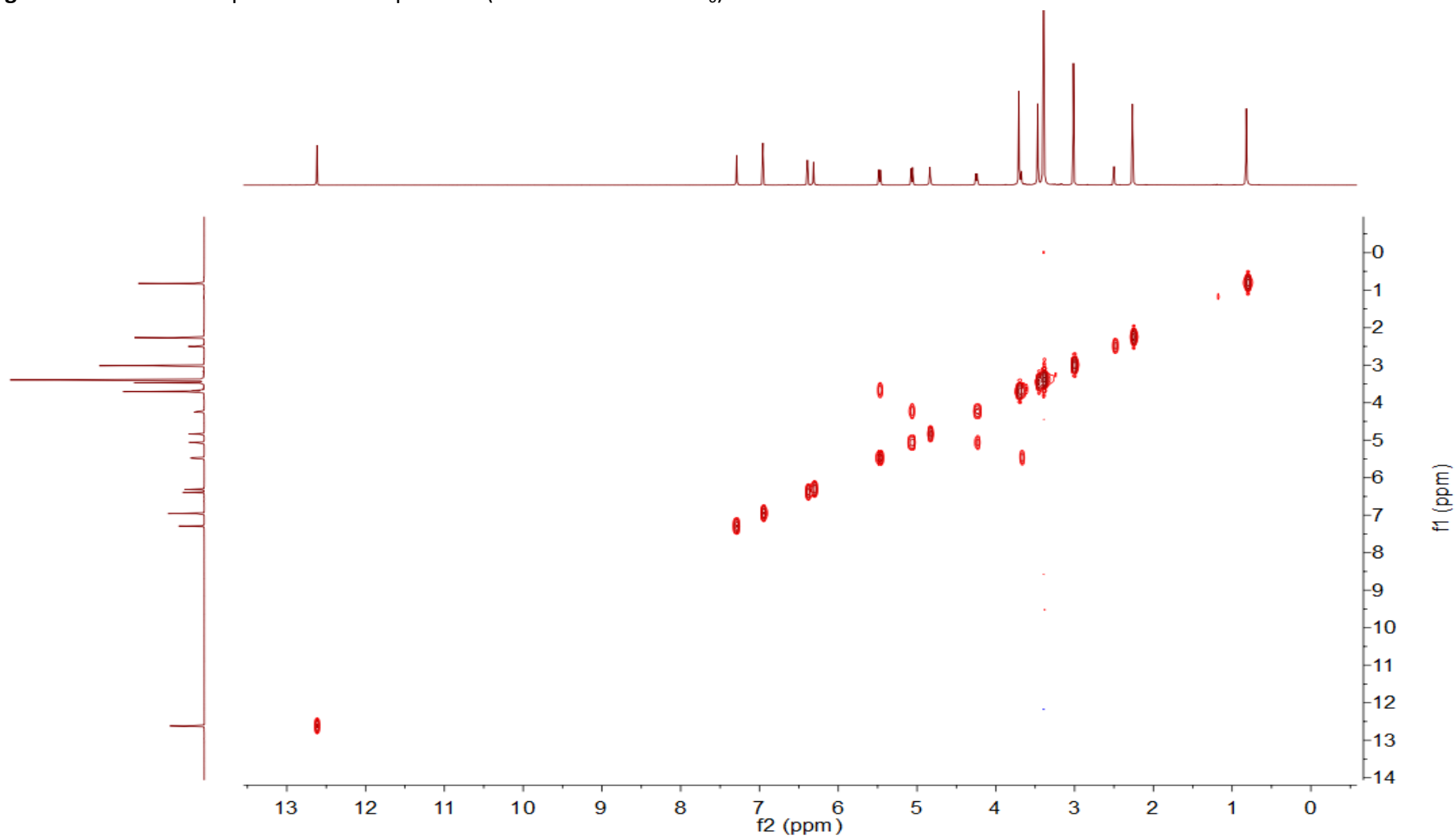
Figure S4. ^1\text{H} - ^1\text{H} COSY spectrum of compound 1 (Recorded in \text{DMSO}-d_6 )
