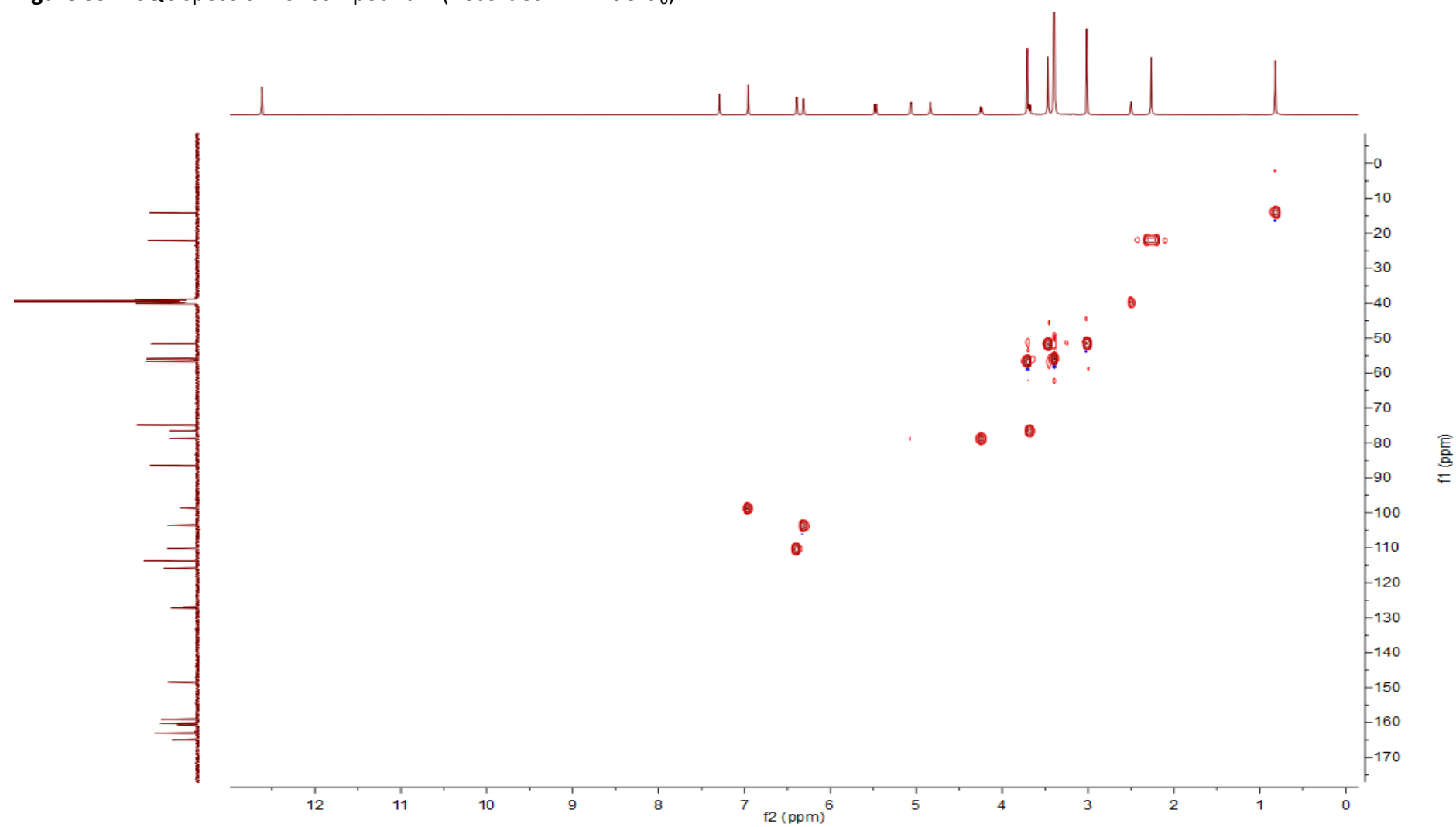
Figure S3. HSQC spectrum of compound 1 (Recorded in DMSO- d_6 )
