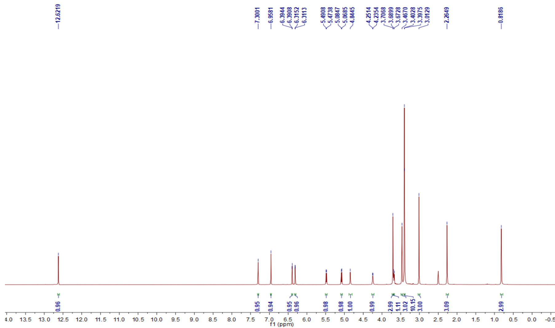
Figure S1. ^1\text{H} NMR spectrum of compound 1 (Recorded in \text{DMSO}-d_6 )
