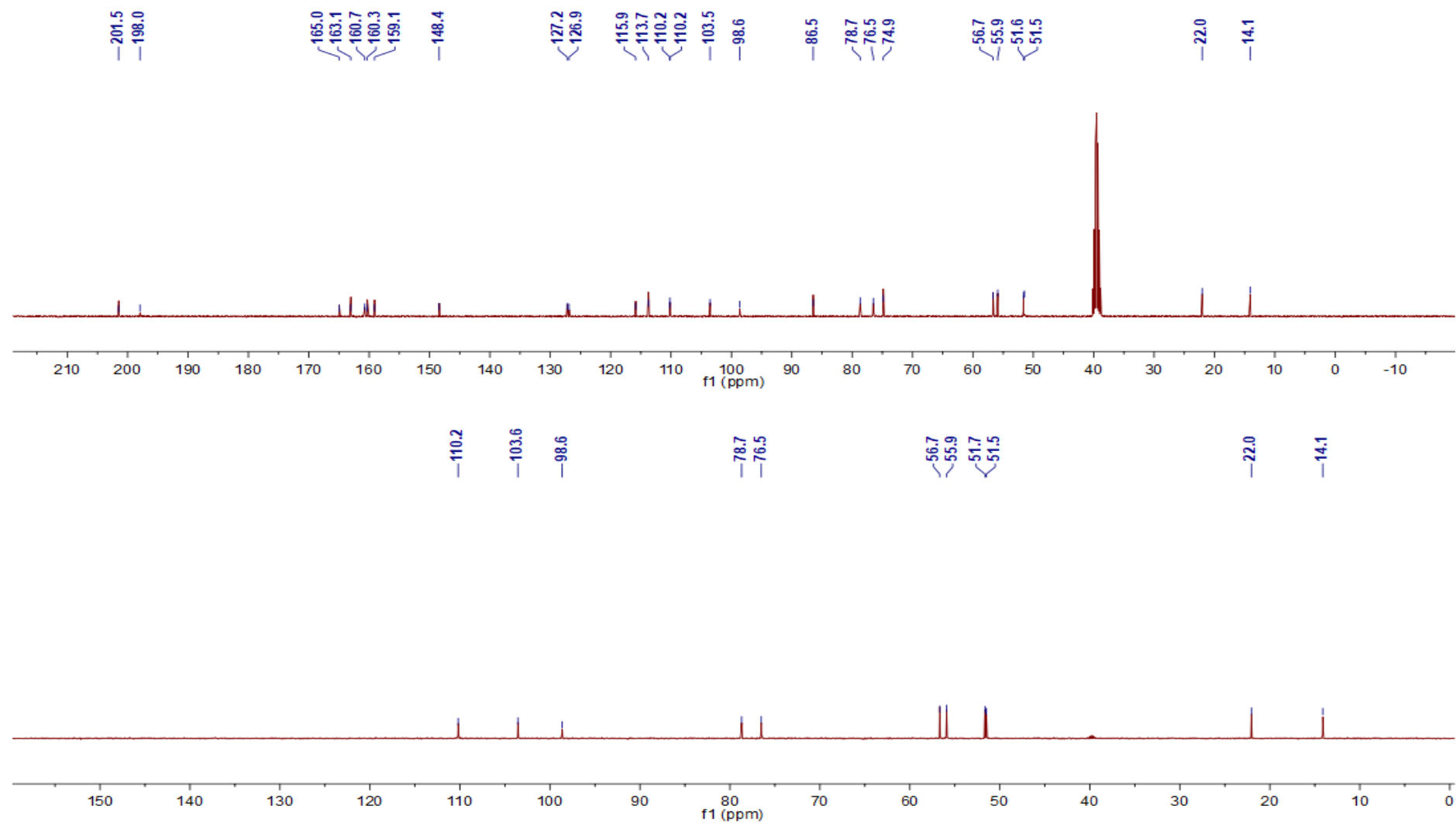
Figure S2. ^{13}\text{C} NMR and DEPT spectra of compound 1 (Recorded in \text{DMSO-}d_6 )
