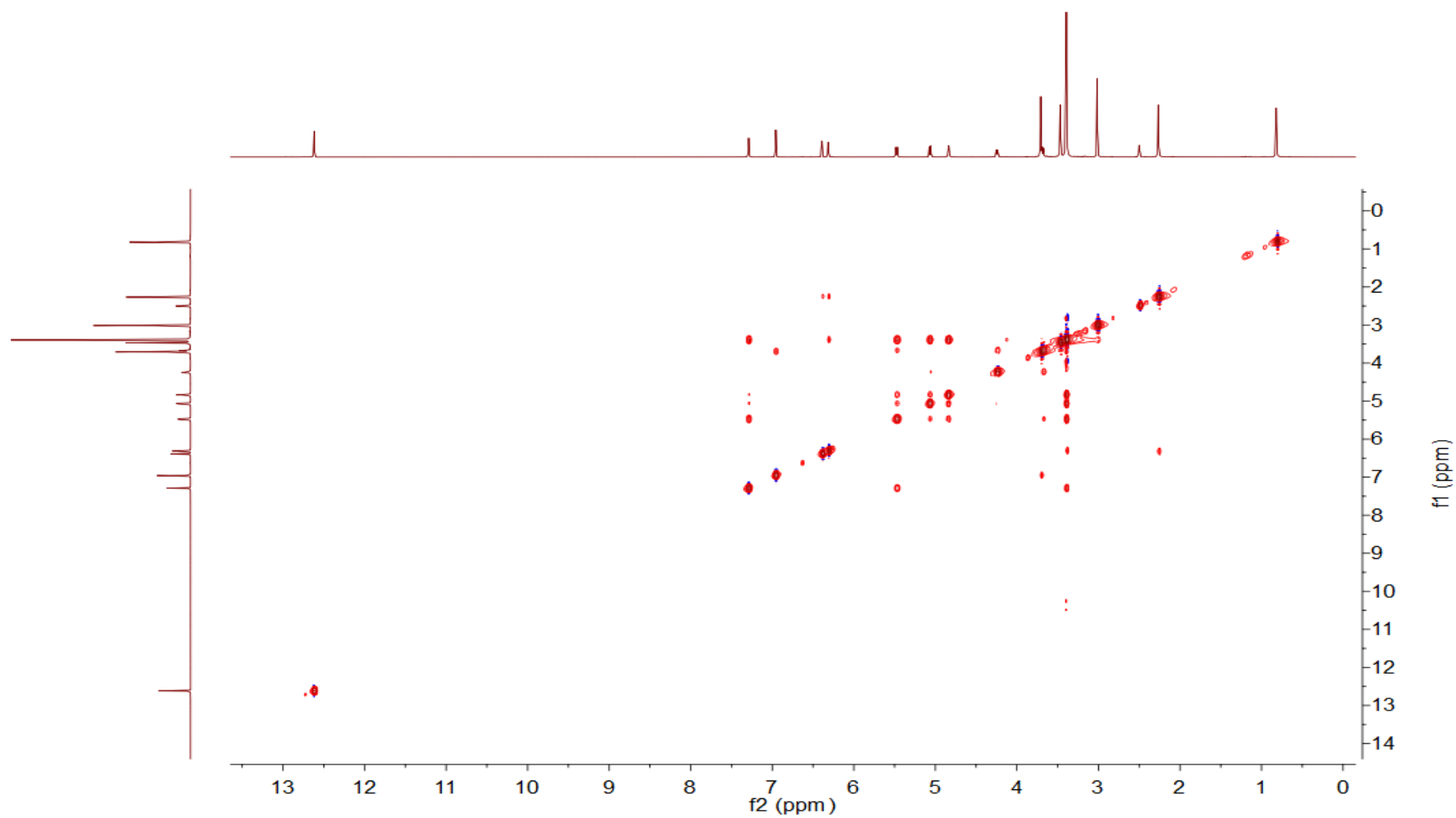
Figure S6. NOESY spectrum of compound 1 (Recorded in DMSO- d_6 )
