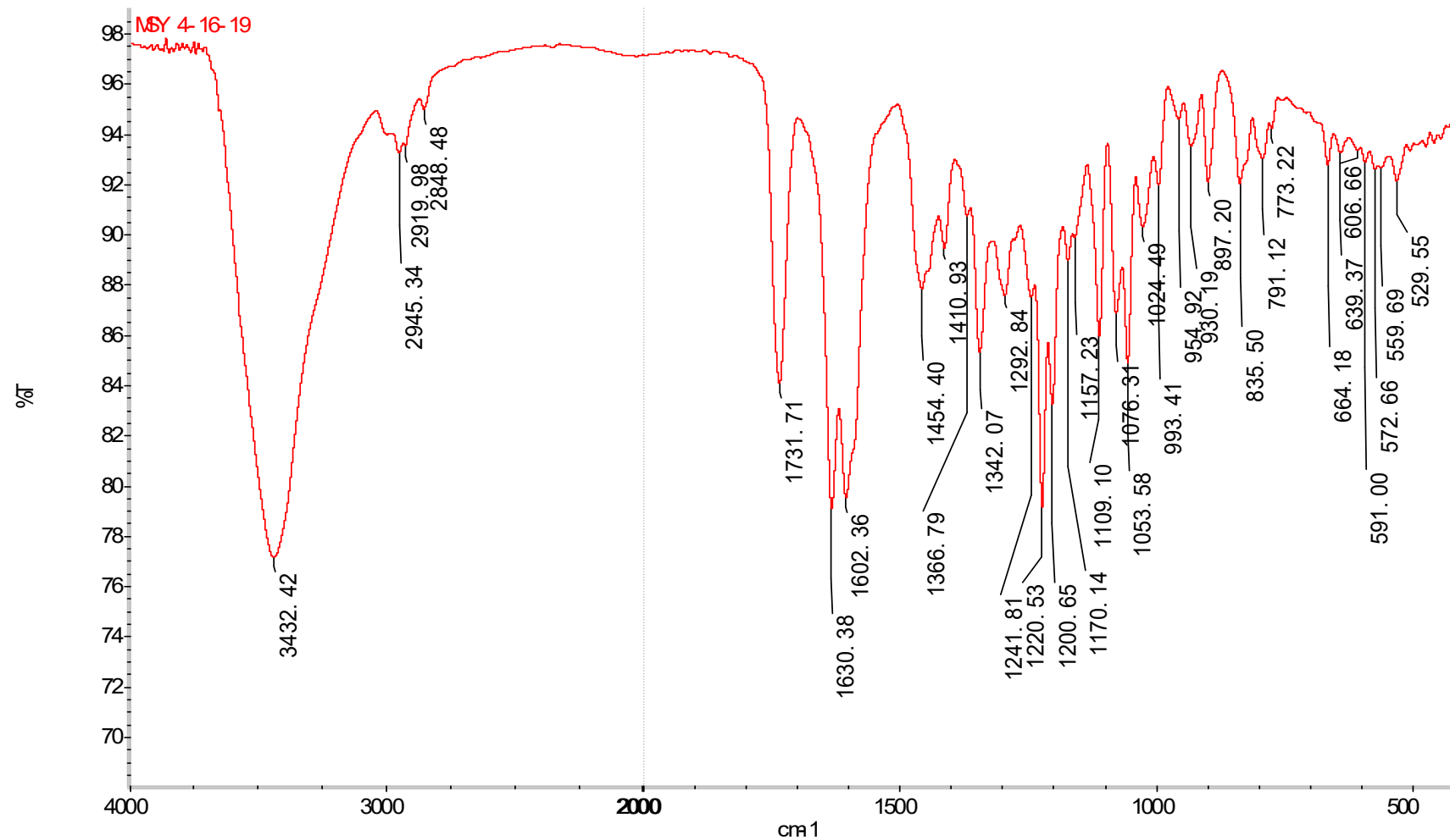
Figure S8. IR spectrum of compound 1
