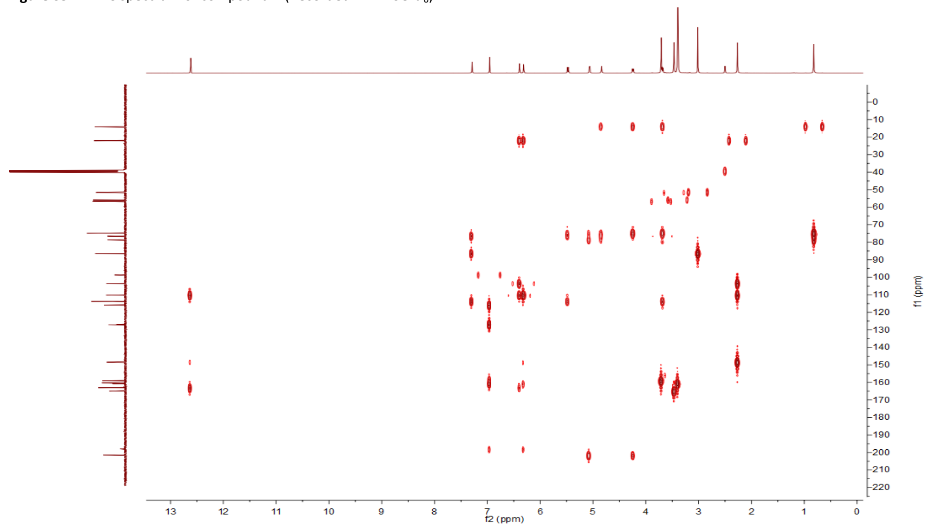
Figure S5. HMBC spectrum of compound 1 (Recorded in DMSO- d_6 )
