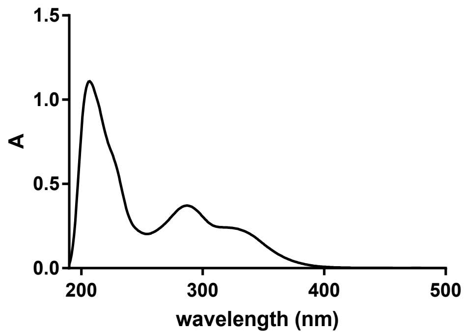
Figure S9. UV spectrum of compound 1
