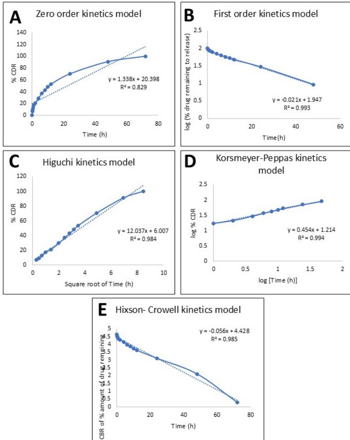
Figure S2: Drug release data of F6 formulation batch tested on (A) Zero order kinetics (B) First order kinetics (C) Higuchi kinetics (D) Korsmeyer-Peppas kinetics (E) Hixson-Crowell kinetics model.
