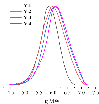
Fig. S2 GPC curves of the resulting ethylene-propylene copolymers (Entries 4-7 in Table 1) by
