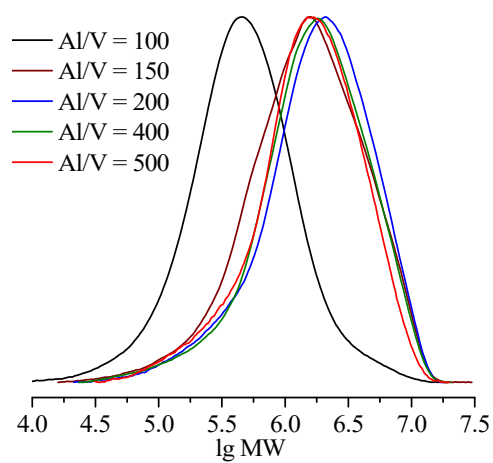
Fig. S3 GPC curves of the resulting ethylene-propylene copolymers (Entries 3, 8-11 in Table 1) with various Al/V molar ratios.
