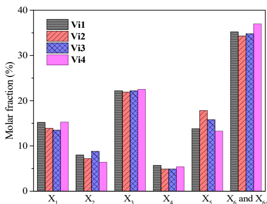
Fig. S1 Molar fraction of uninterrupted methyl sequences in the ethylene-propylene copolymers (Entries 4-7 in Table 1) prepared by using vanadium complexes Vi1-Vi4 as precatalyst.
