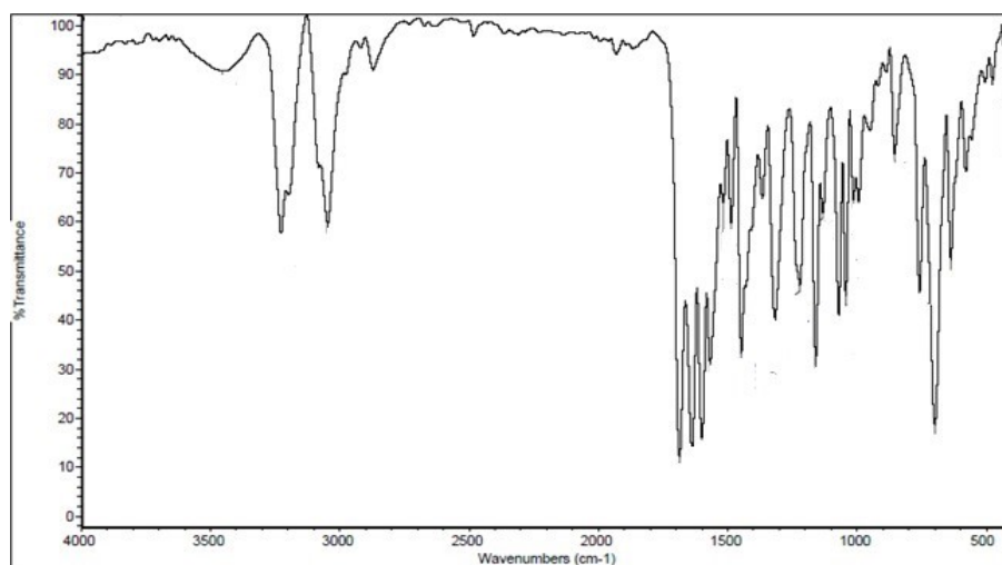
S.1. Infrared spectra of: (a) H 2 TTAH; and (b) [Zn 2 (H 2 TTAH)(OH) 4 (C 5 H 5 N) 3 C 2 H 5 OH]
