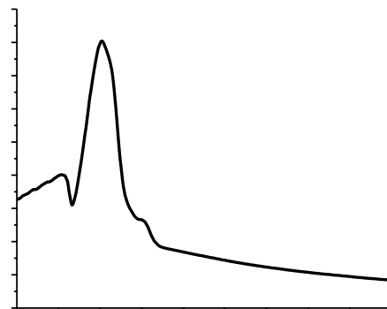
S.4. UV-Vis electronic spectra of (a) H 2 TTAH and (b) [Zn 2 (TTAH)(OH) 2 (C 5 H 5 N) 2 (C 2 H 5 OH) 2 ]
