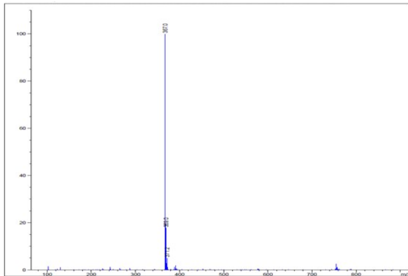
S.3. ESI- mass spectrum of H 2 TTAH
