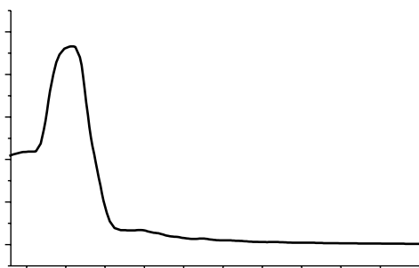
S.4. UV-Vis electronic spectra of (a) H 2 TTAH and (b) [Zn 2 (TTAH)(OH) 2 (C 5 H 5 N) 2 (C 2 H 5 OH) 2 ]
