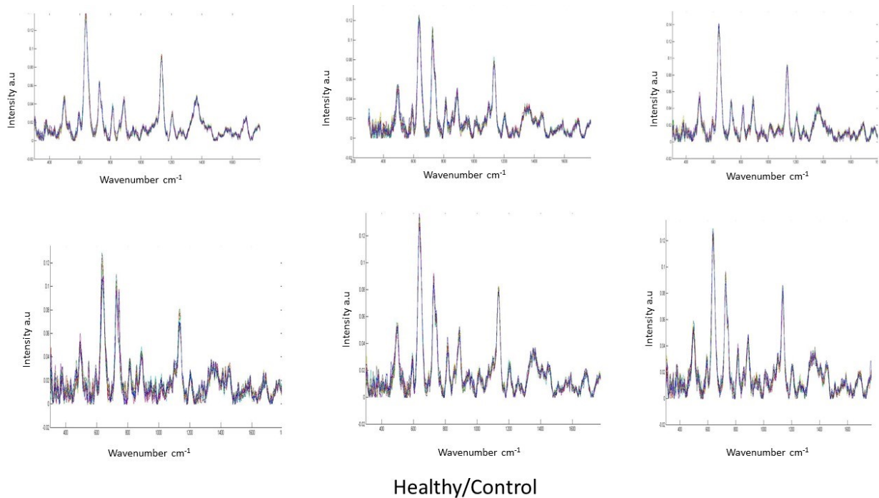
Fig. S2: Original SERS spectra of healthy/control samples.
