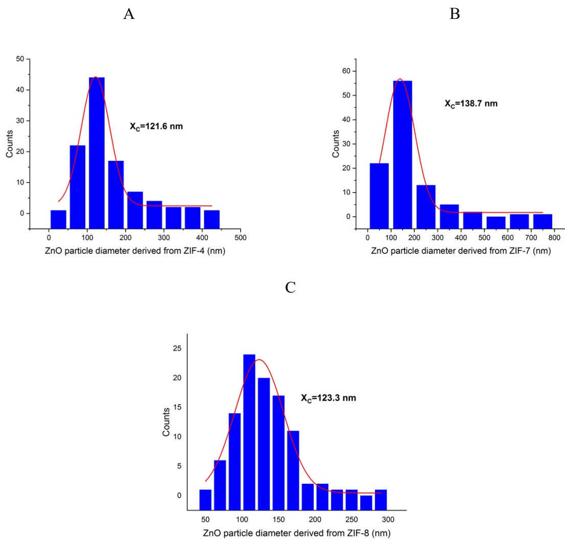
Figure S3. Graphs showing the average diameter of particles in a) ZnO derived from ZIF-4, B) ZnO derived from ZIF-7 and C) ZnO derived from ZIF-8.
