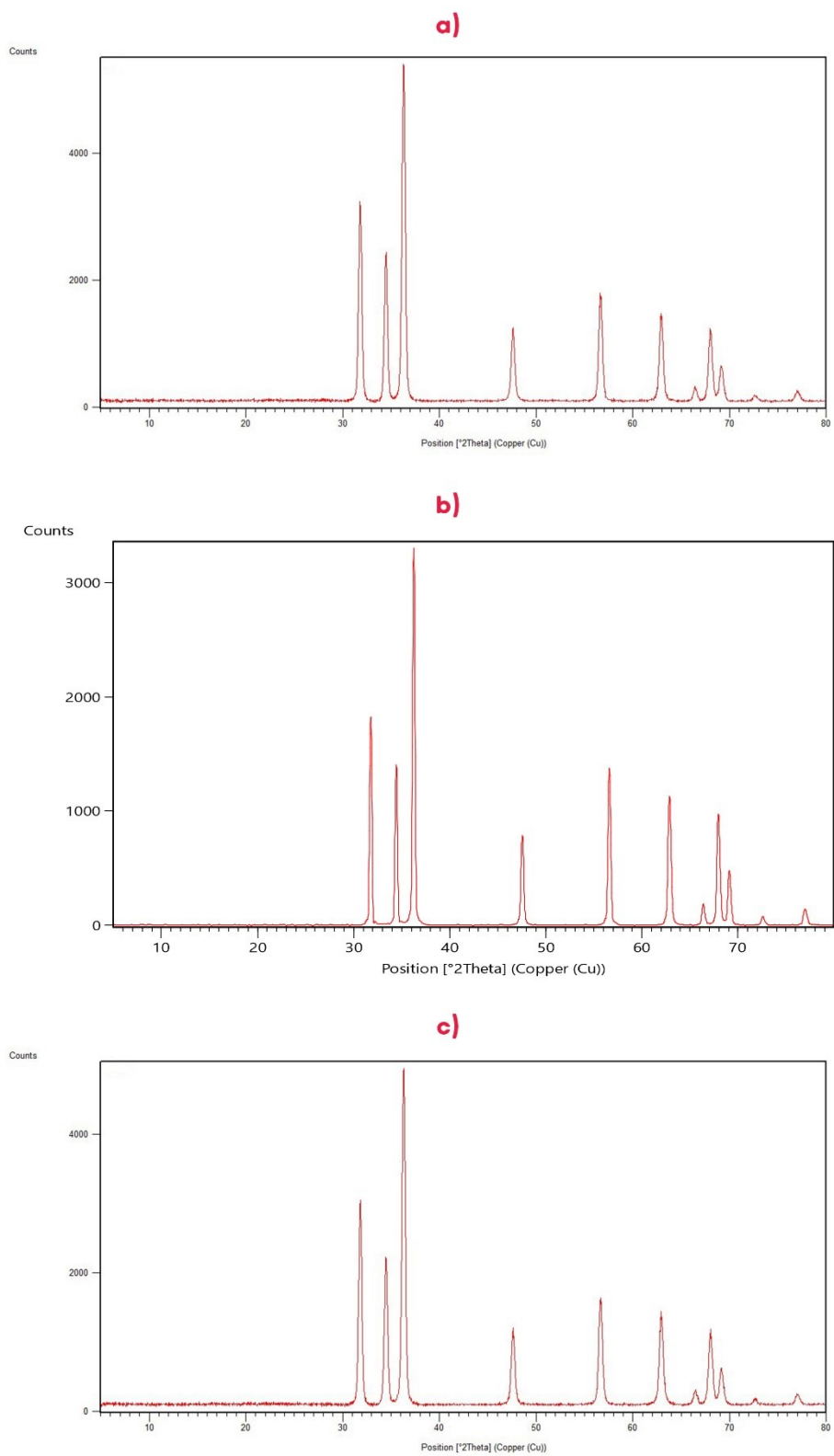
Figure S1. The PXRD patterns of three types of zinc oxide driven from a) ZIF-4, b) ZIF-7 and c) ZIF-8.
