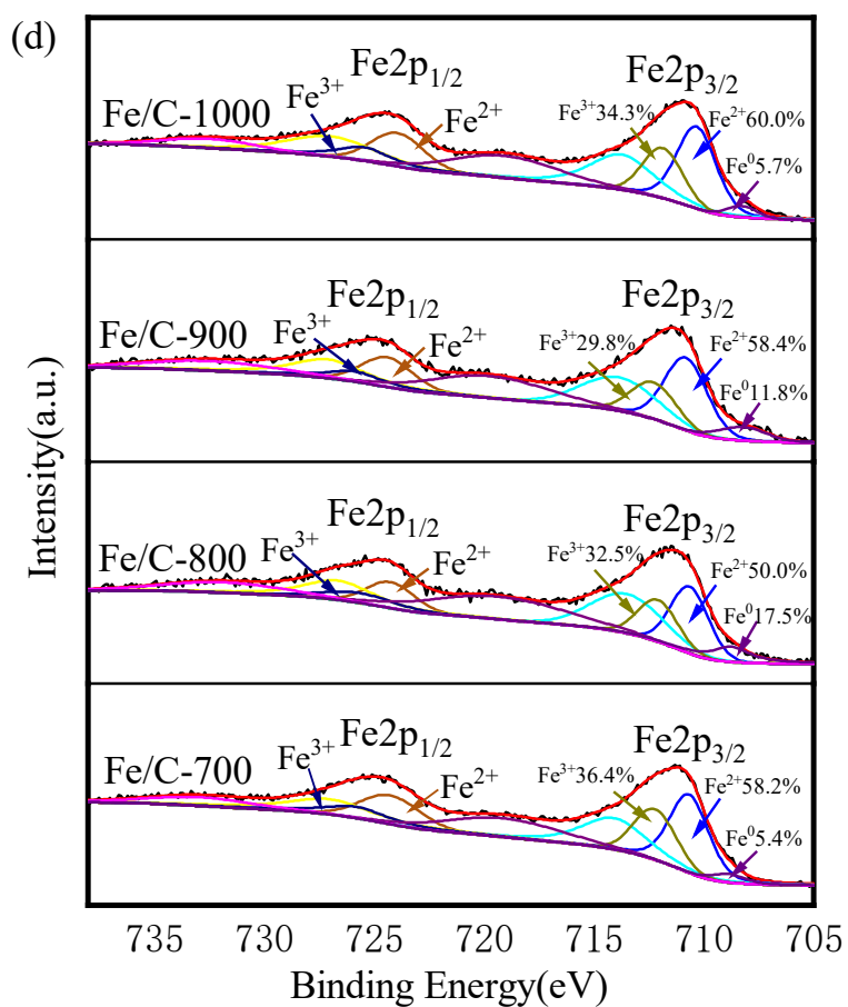
Fig. S1 XPS patterns of Fe/C catalysts: wide scan(a); C1s(b); O1s(c); and Fe2p(d)
