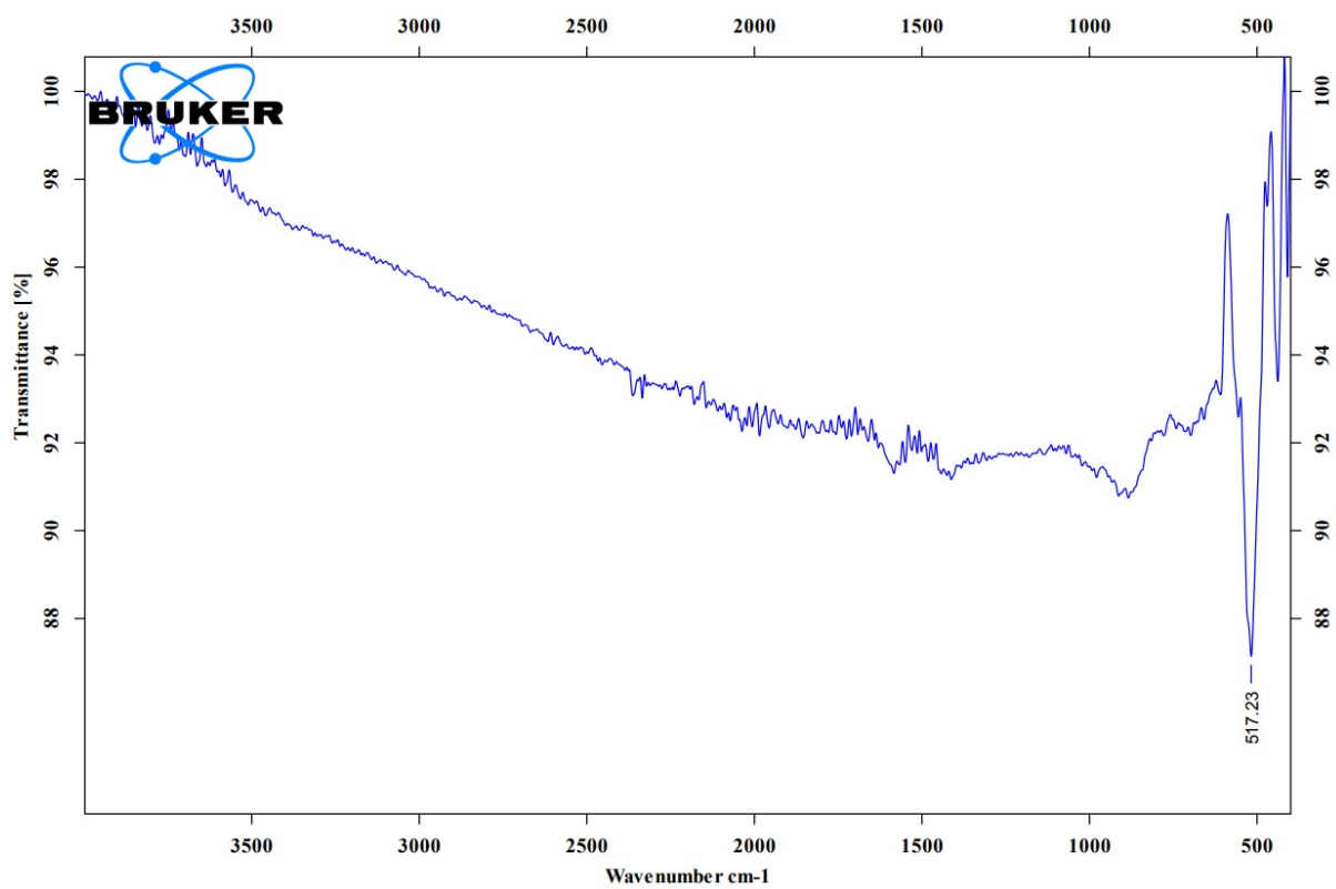
Figure S1. FTIR spectrum of spent ZnO nanoplates after used as photocatalyst for RhB degradation.
