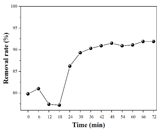
Fig. S2 The temporal evolution of defluorination efficiency in the IE-BA system.
