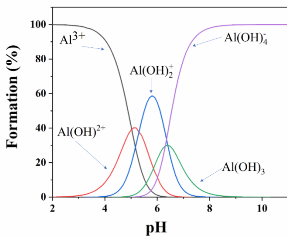
Fig. S1 Fraction-pH diagram for aluminum species in an aqueous solution. T = 25\text{ }^\circ\text{C} , [\text{Al}^{3+}]_T = 5 \times 10^{-6}\text{ M} .
