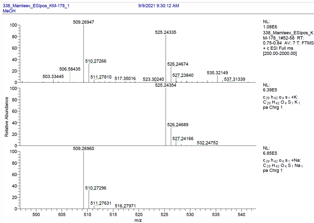
Figure S13: HRMS of compound 10c (ESI + ).
