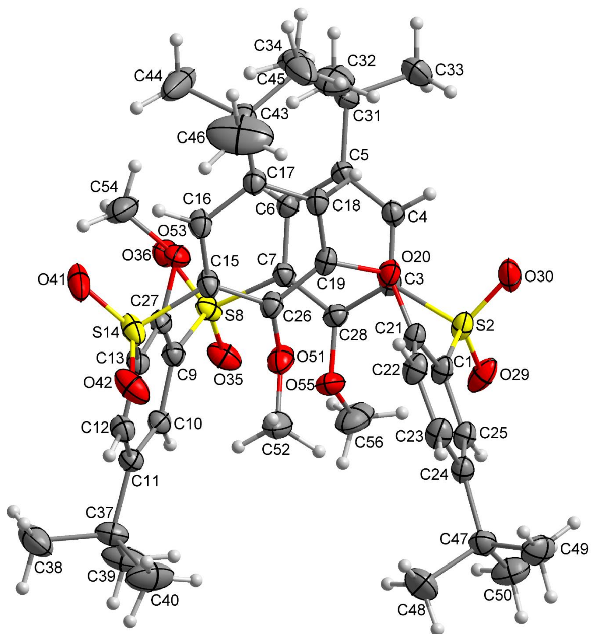
Figure S40: The numbering scheme of compound 15 . The ADPs drawn at 50 % probability level.
