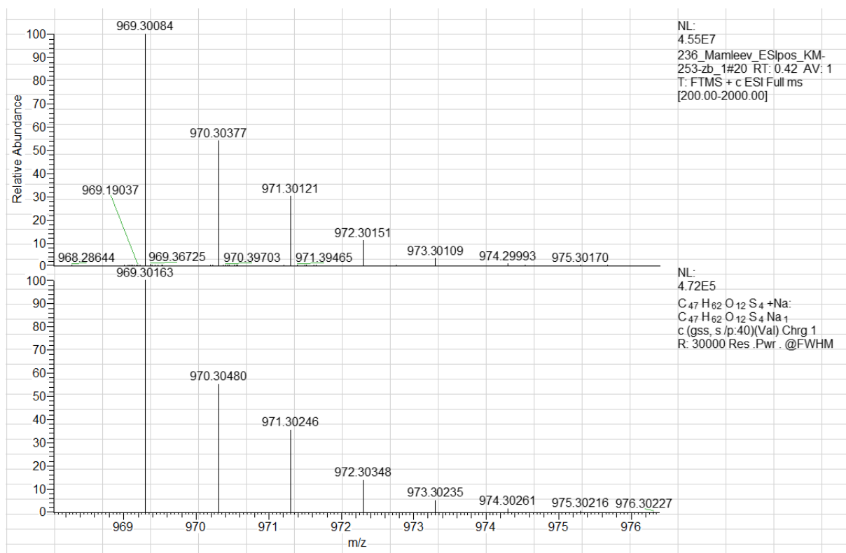
Figure S22: HRMS of compound 13 (ESI + ).
