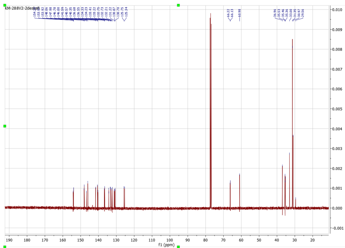
Figure S24: ^{13}\text{C} NMR of compound 14 ( \text{CDCl}_3 , 100 MHz)
