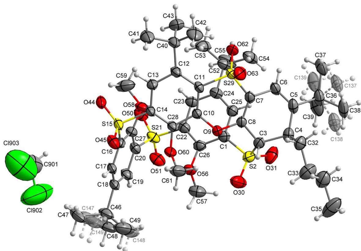
Figure S38: The numbering scheme of compound 13 . The ADPs drawn at 50 % probability level. The weakly occupied atoms depicted as transparent.
