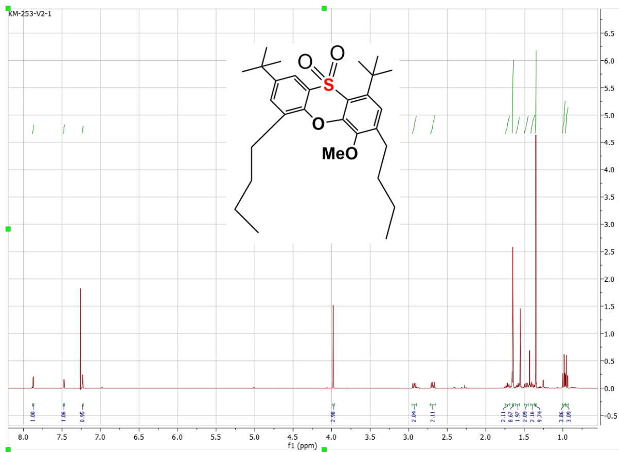
Figure S11: 1 H NMR of compound 10c (CDCl 3 , 400 MHz).
