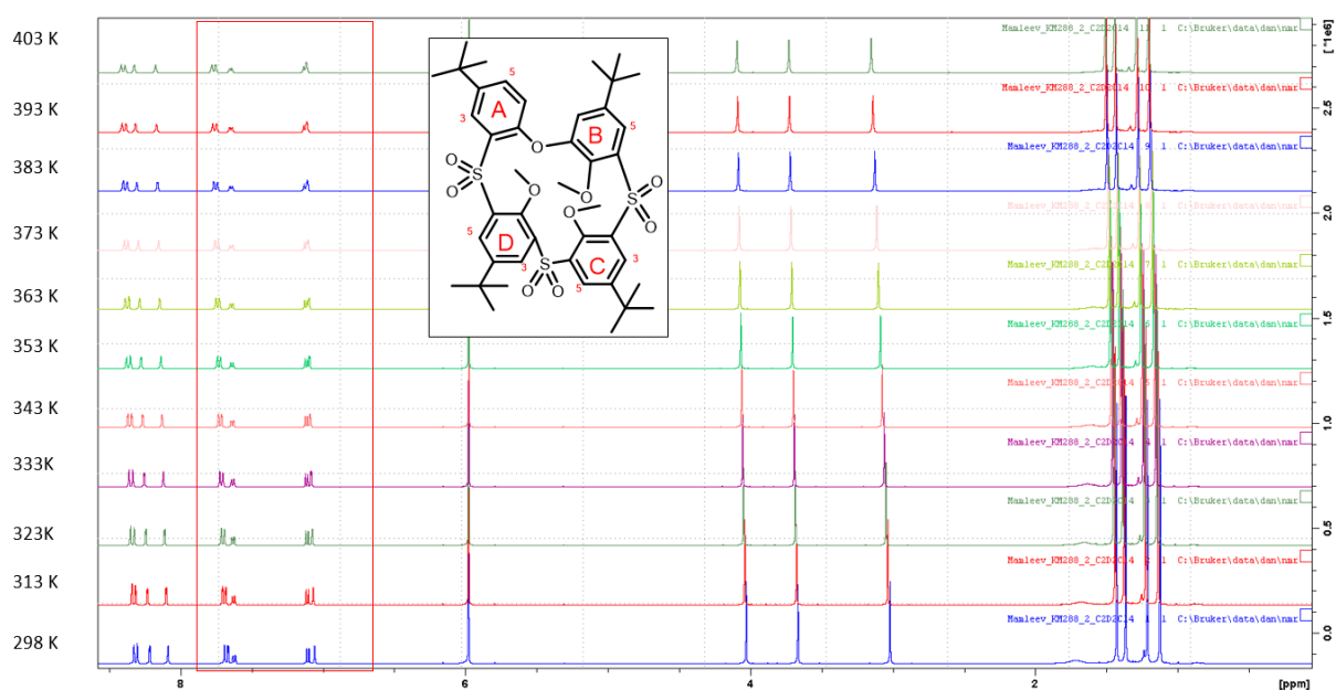
Figure S30: ^1\text{H} NMR of compound 15 ( \text{C}_2\text{D}_2\text{Cl}_4 , 500 MHz).
