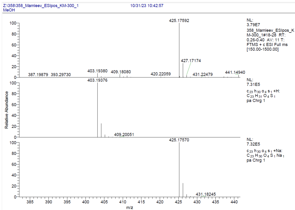
Figure S7: HRMS of compound 10a (ESI + ).
