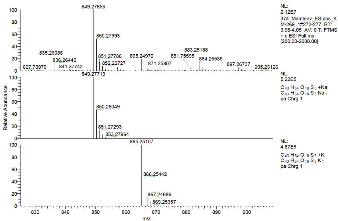
Figure S25: HRMS of compound 14 (ESI + ).
