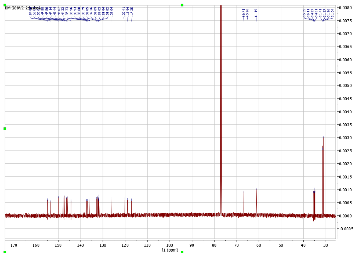
Figure S32: 13 C NMR of compound 15 (CDCl 3 , 100 MHz)
