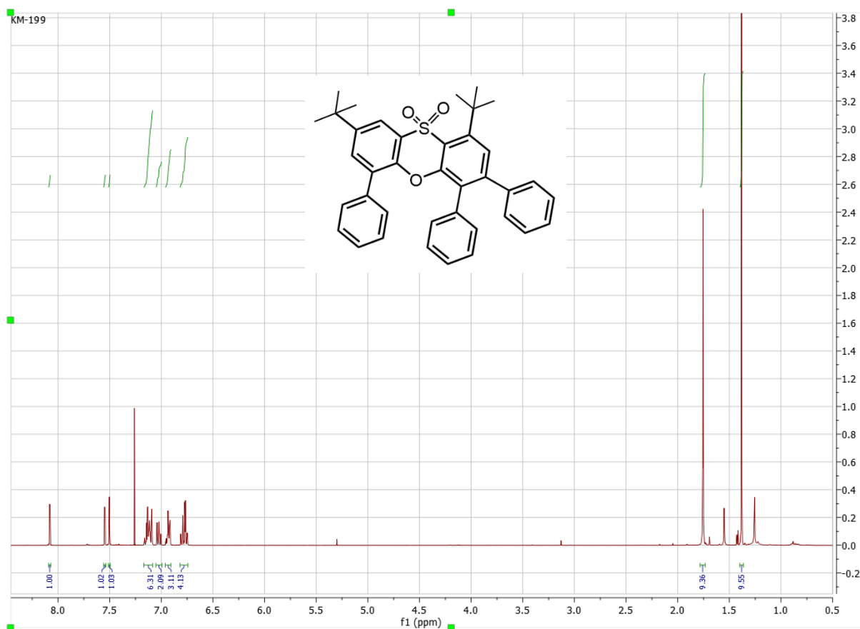
Figure S17: 1 H NMR of compound 12 (CDCl 3 , 400 MHz).
