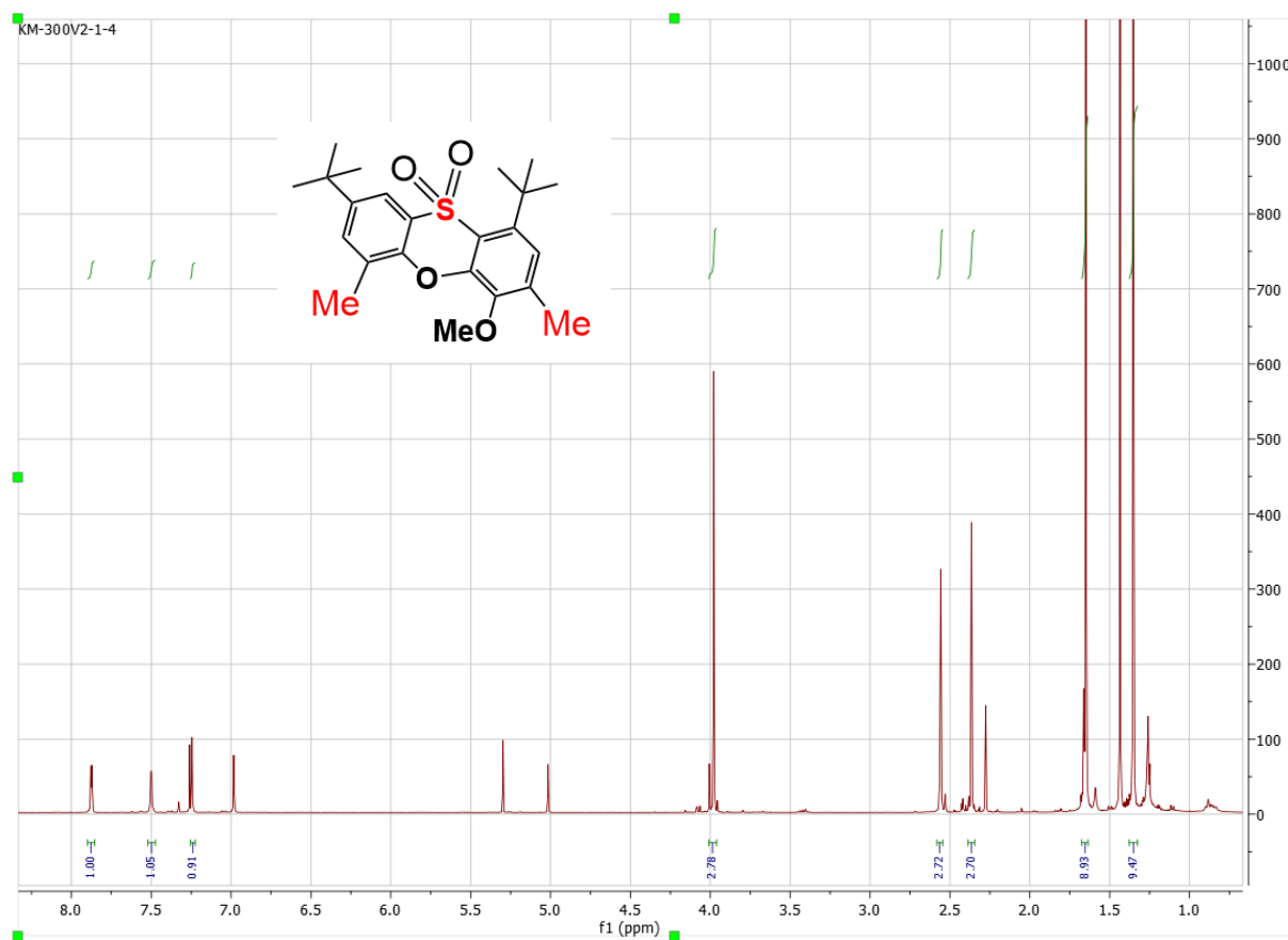
Figure S5: 1 H NMR of compound 10a (CDCl 3 , 400 MHz).
