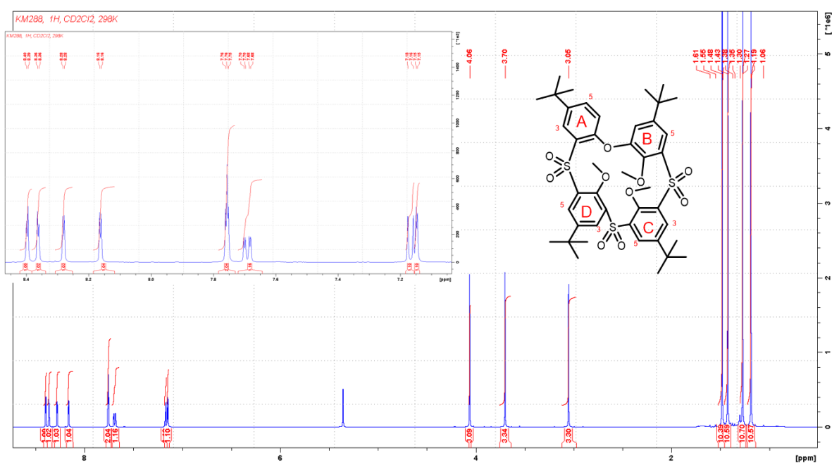
Figure S27: 1 H NMR of compound 15 (CD 2 Cl 2 , 500 MHz, 298 °K).
