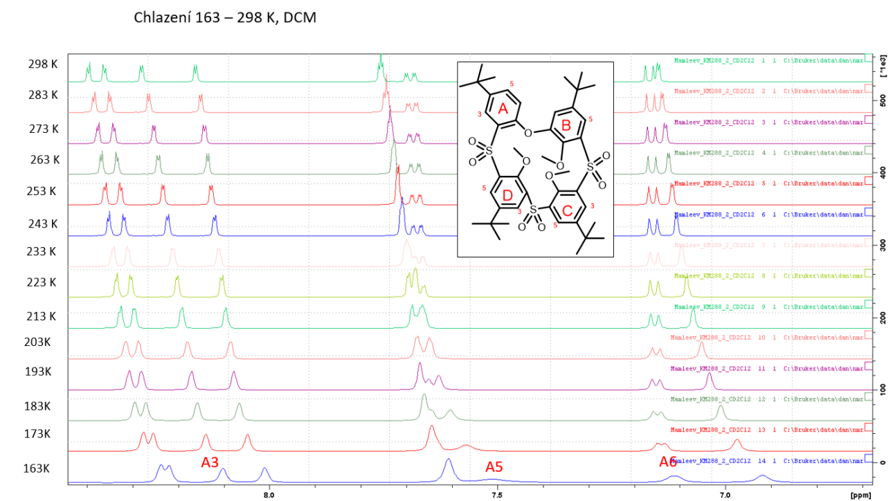
Figure S29: ^1\text{H} NMR of compound 15 ( \text{CD}_2\text{Cl}_2 , 500 MHz).
