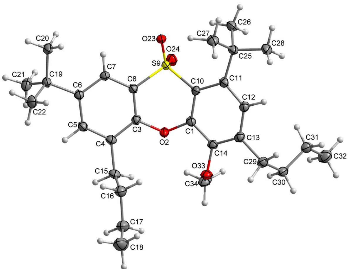
Figure S35: The numbering scheme of compound 10c . The ADPs drawn at 50 % probability level.
