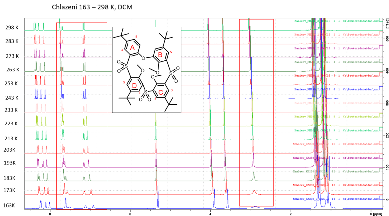
Figure S28: ^1\text{H} NMR of compound 15 ( \text{CD}_2\text{Cl}_2 , 500 MHz).
