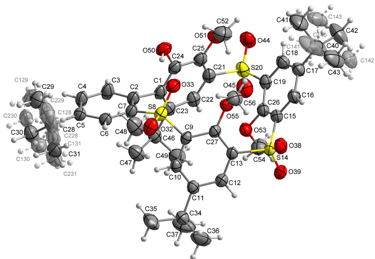
Figure S39: The numbering scheme of compound 14 . The ADPs drawn at 50 % probability level. The weakly occupied atoms depicted as transparent.
