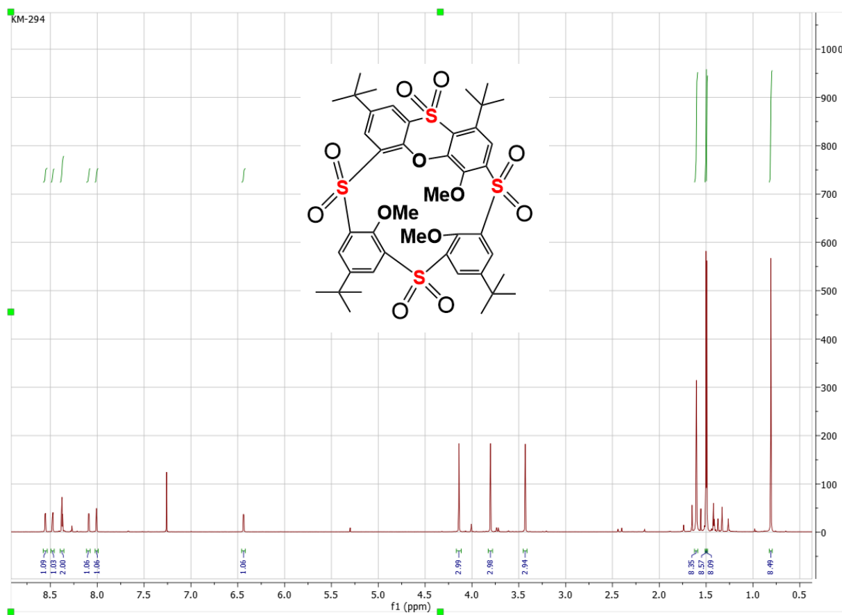
Figure S4: 1 H NMR of compound 9 (CDCl 3 , 400 MHz).
