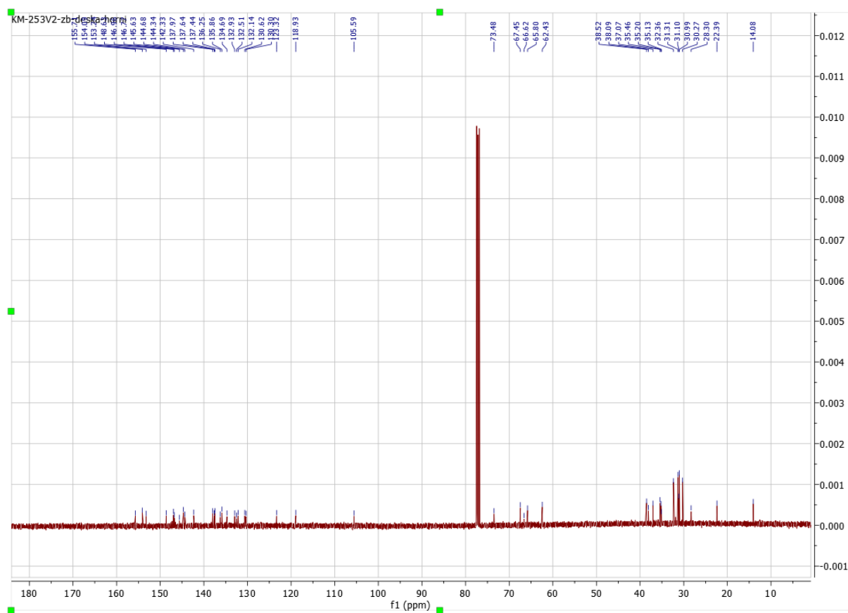
Figure S21: ^{13}\text{C} NMR of compound 13 ( \text{CDCl}_3 , 100 MHz)
