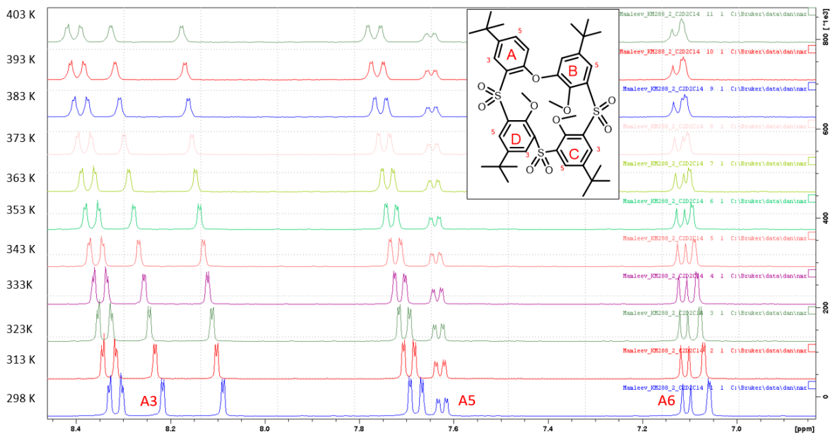
Figure S31: ^1\text{H} NMR of compound 15 ( \text{C}_2\text{D}_2\text{Cl}_4 , 500 MHz).
