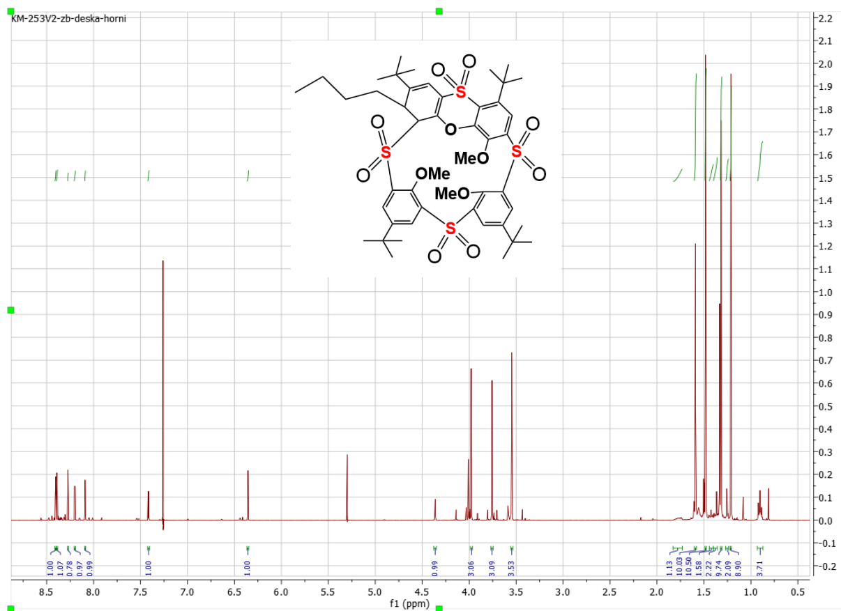
Figure S20: ^1\text{H} NMR of compound 13 (CDCl 3 , 400 MHz).
