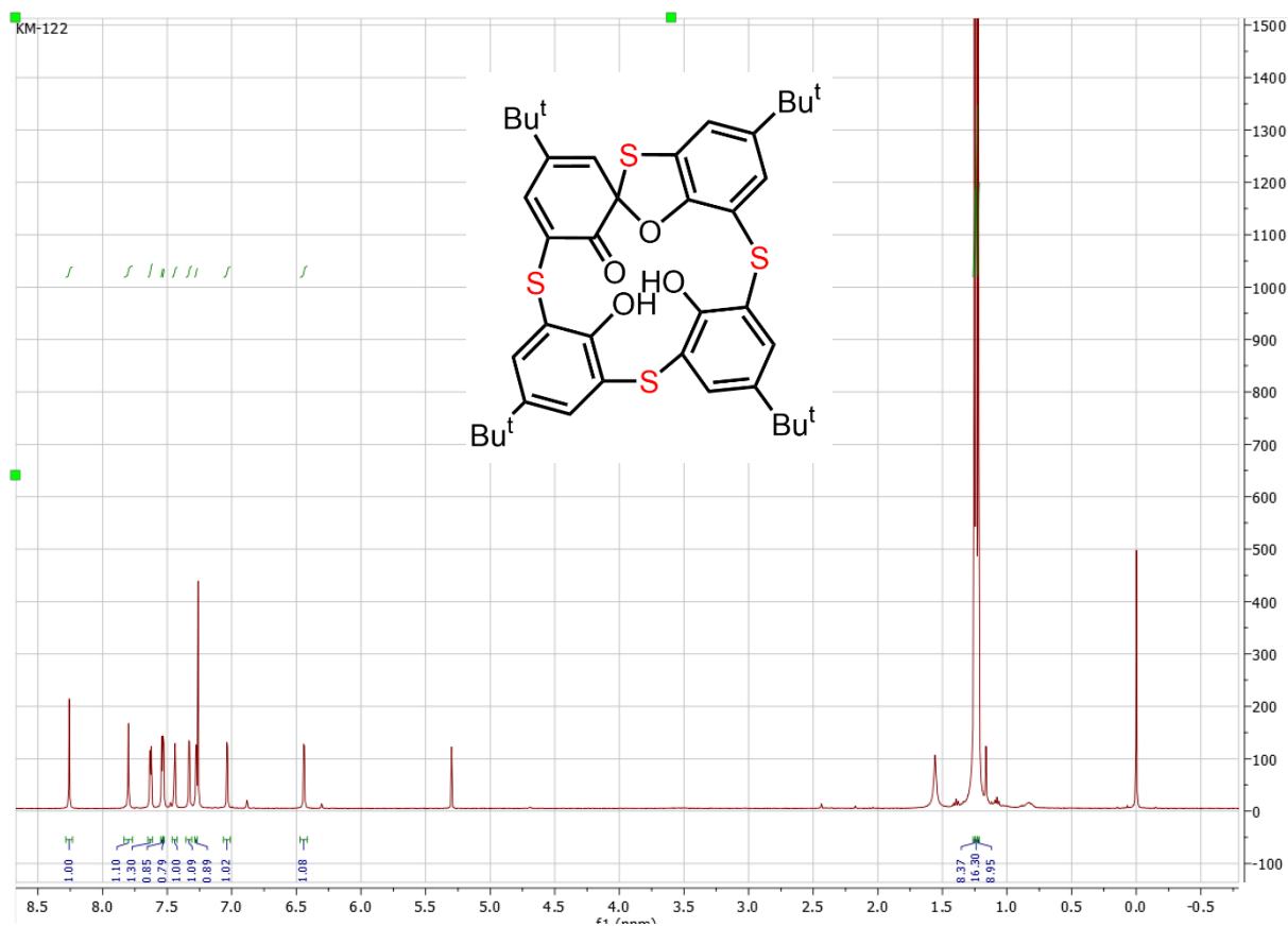
Figure S1: ^1\text{H} NMR of compound 2 ( \text{CDCl}_3 , 400 MHz).
