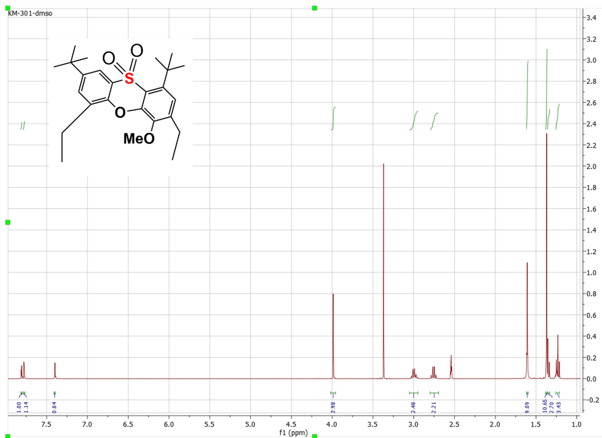
Figure S8: 1 H NMR of compound 10b (DMSO-d 6 , 400 MHz).
