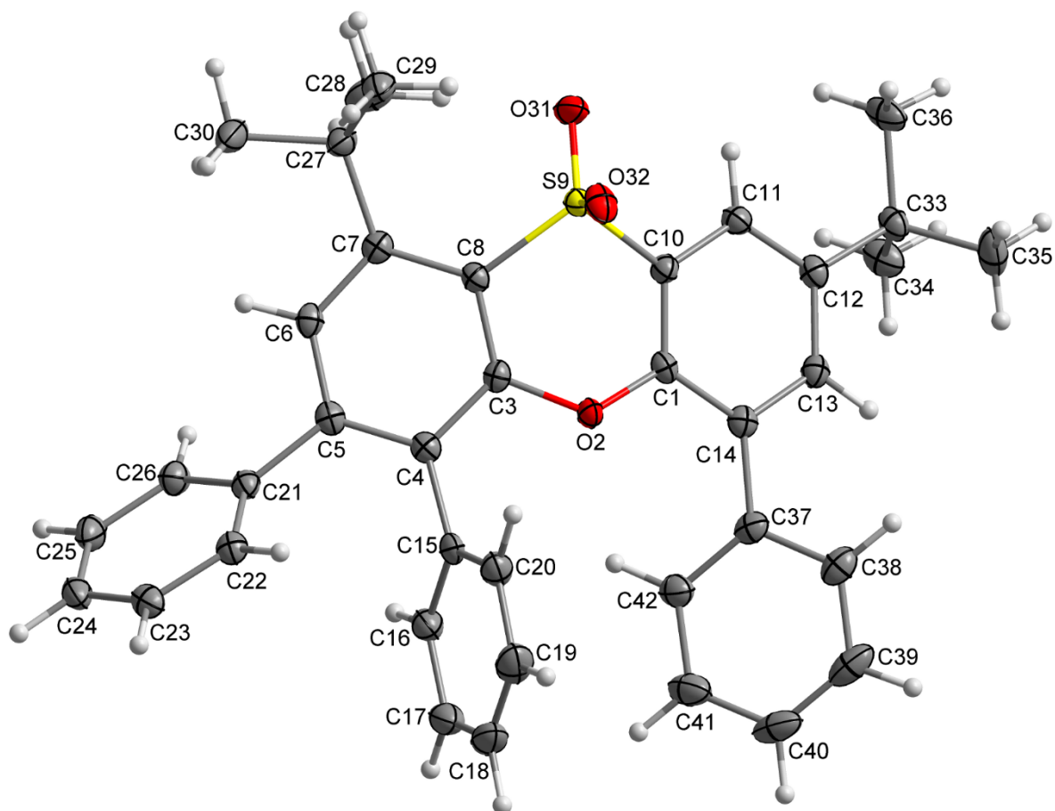
Figure S37: The numbering scheme of compound 12 . The ADPs drawn at 50 % probability level.
