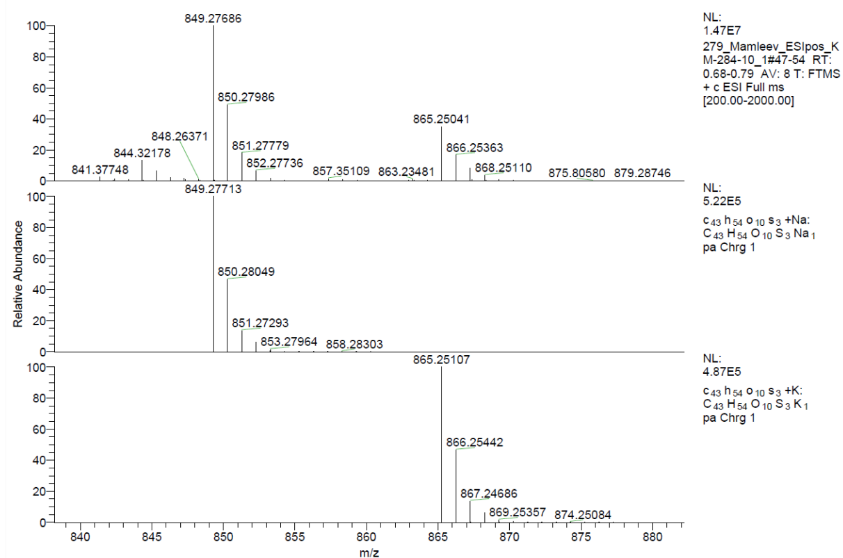
Figure S33: HRMS of compound 15 (ESI + ).
