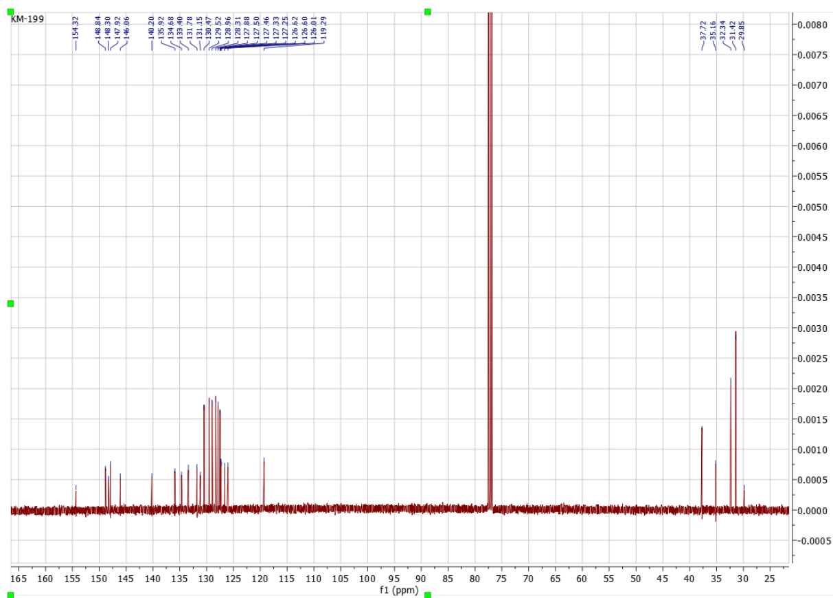
Figure S18: ^{13}\text{C} NMR of compound 12 ( \text{CDCl}_3 , 100 MHz)
