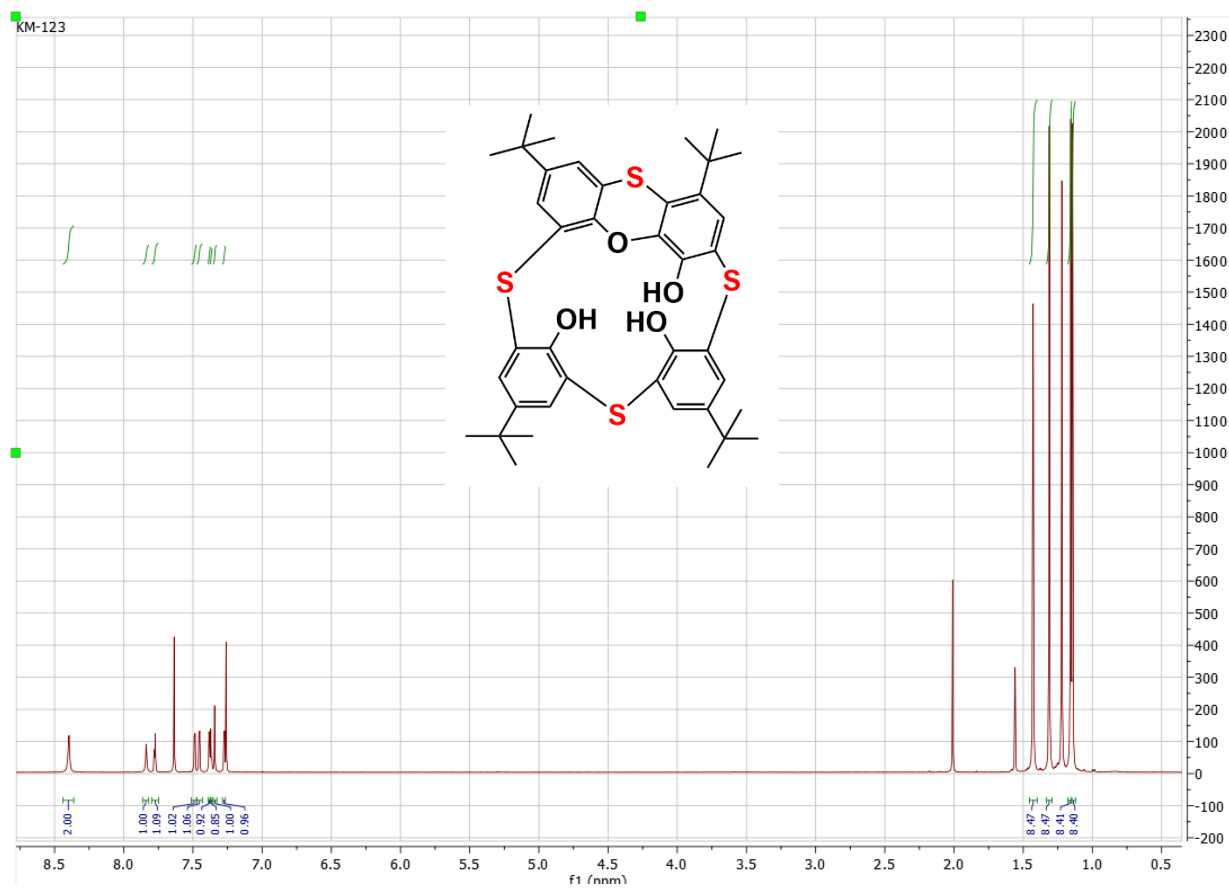
Figure S2: ^1\text{H} NMR of compound 4 (CDCl 3 , 400 MHz).
