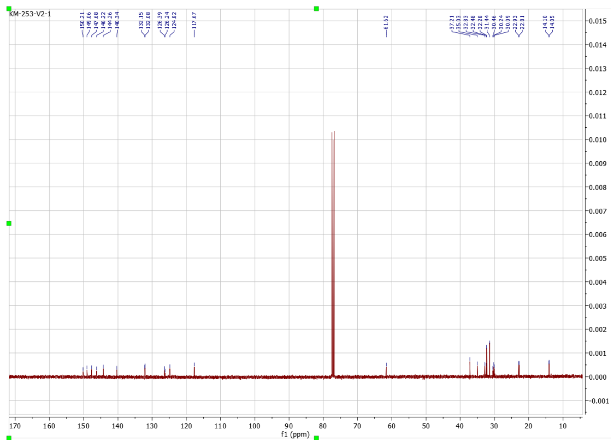
Figure S12: ^{13}\text{C} NMR of compound 10c ( \text{CDCl}_3 , 100 MHz)
