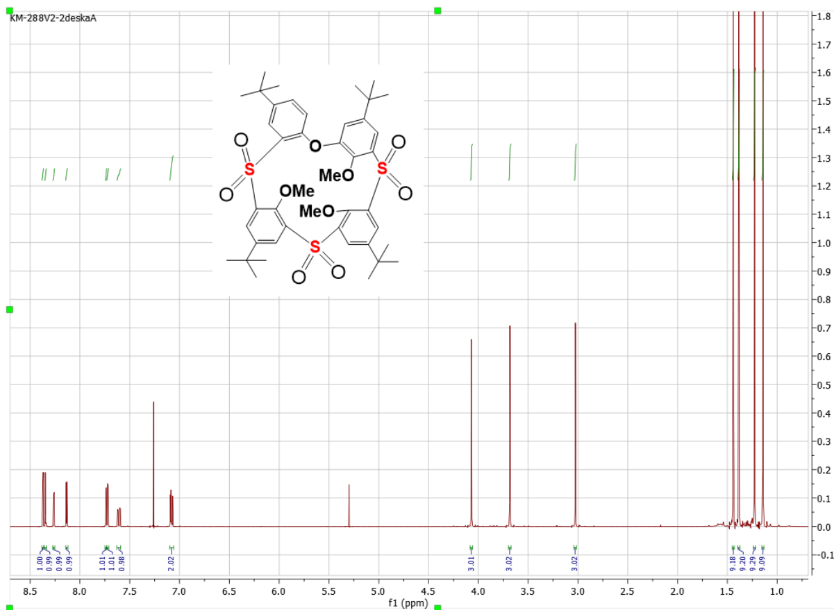
Figure S26: 1 H NMR of compound 15 (CDCl 3 , 400 MHz).
