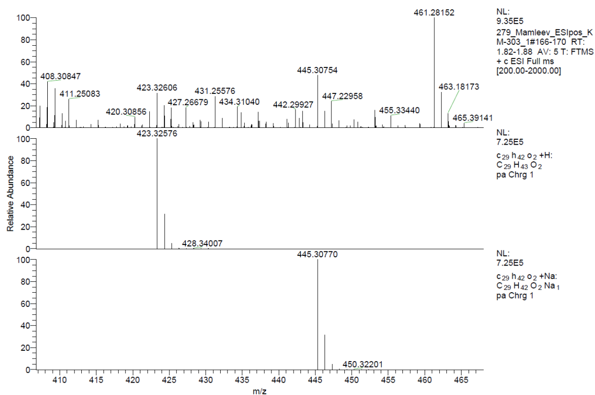
Figure S16: HRMS of compound 11 (ESI + ).
