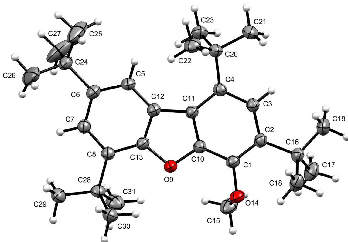
Figure S36: The numbering scheme of compound 11 , drawn at 50 % probability level.
