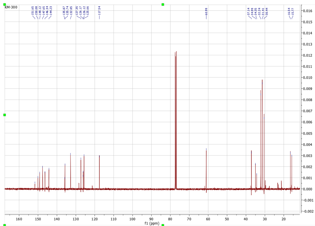
Figure S6: ^{13}\text{C} NMR of compound 10a ( \text{CDCl}_3 , 100 MHz)
