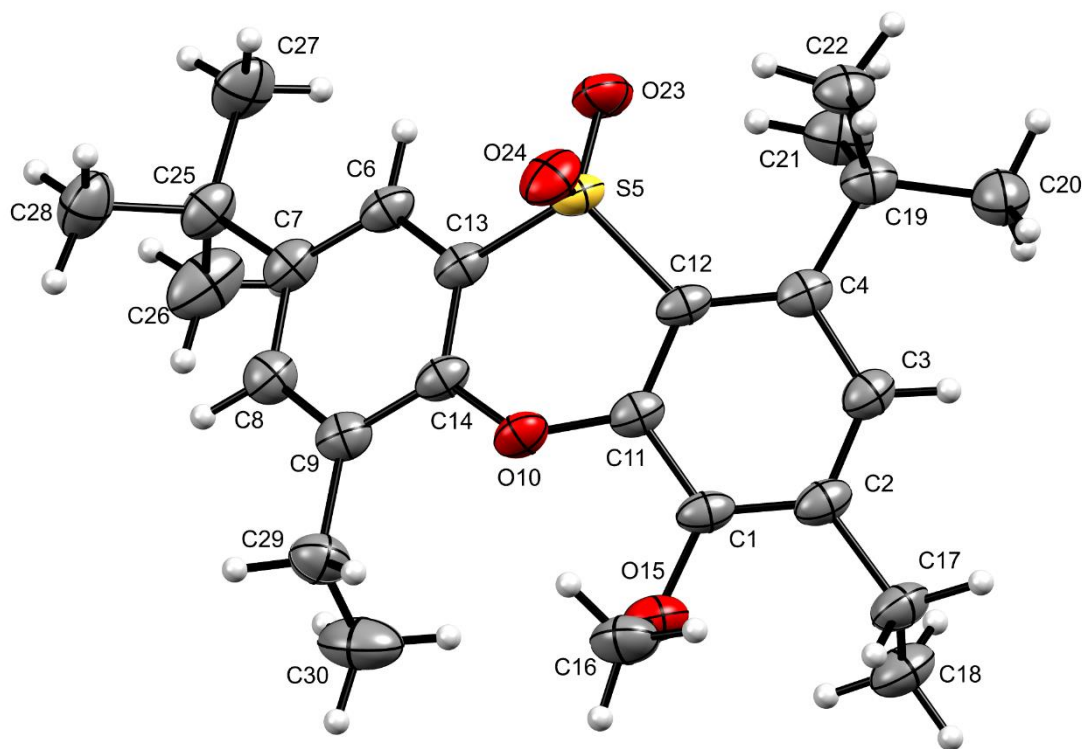
Figure S34: The numbering scheme of compound 10b , drawn at 50 % probability level.
