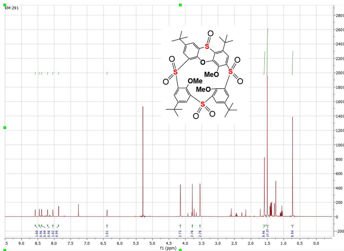
Figure S3: ^1\text{H} NMR of compound 9' (CDCl 3 , 400 MHz).
