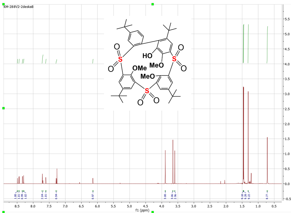
Figure S23: 1 H NMR of compound 14 (CDCl 3 , 400 MHz).
