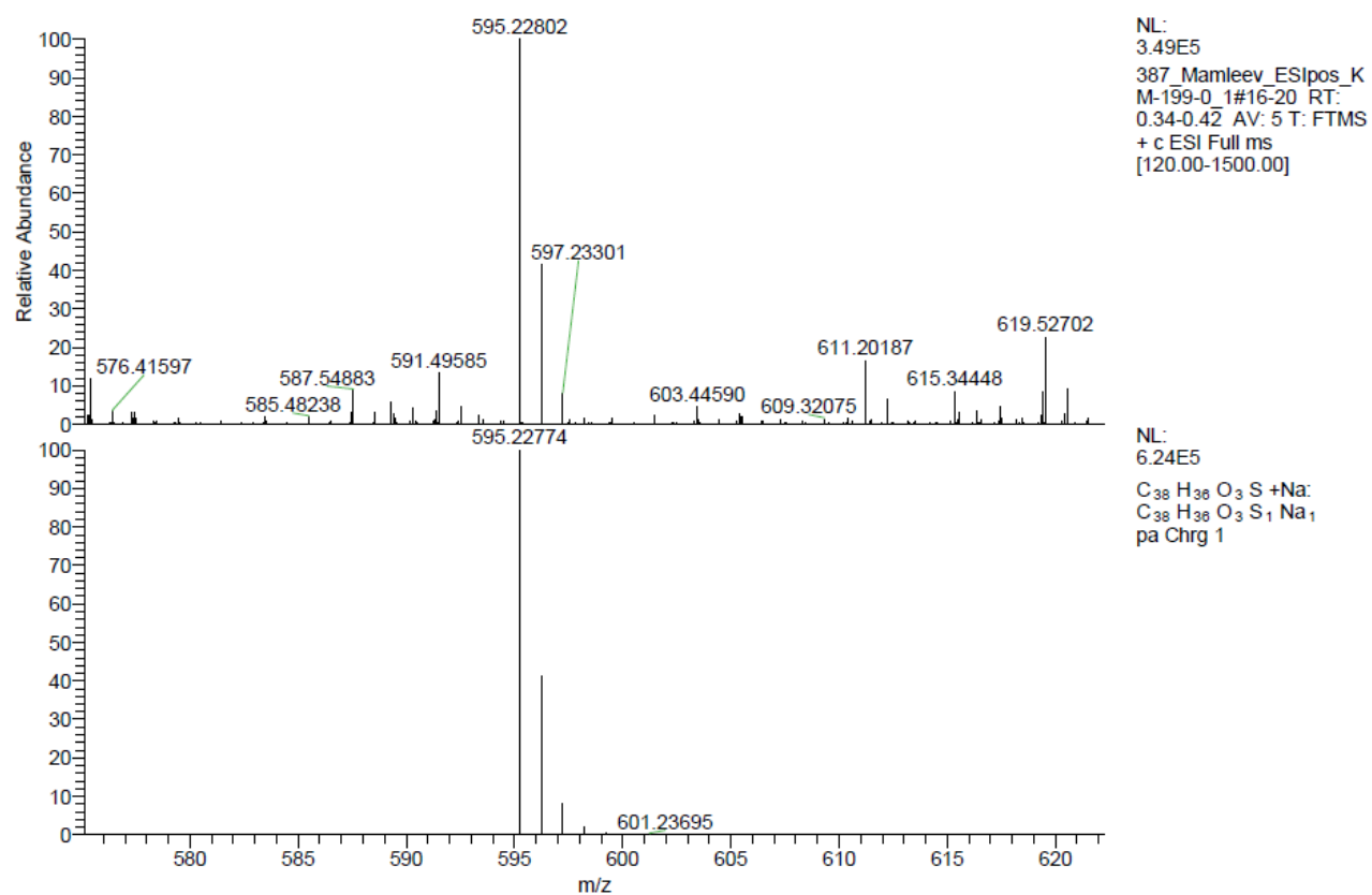
Figure S19: HRMS of compound 12 (ESI + ).
