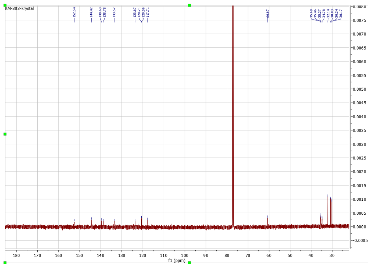
Figure S15: 13 C NMR of compound 11 (CDCl 3 , 100 MHz)
