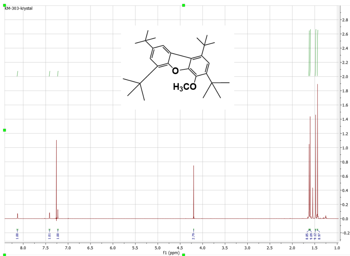
Figure S14: ^1\text{H} NMR of compound 11 ( \text{CDCl}_3 , 400 MHz).
