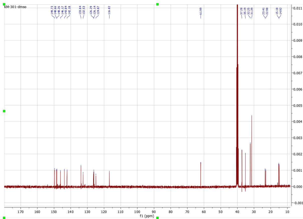
Figure S9: ^{13}\text{C} NMR of compound 10b (DMSO- \text{d}_6 , 100 MHz)
