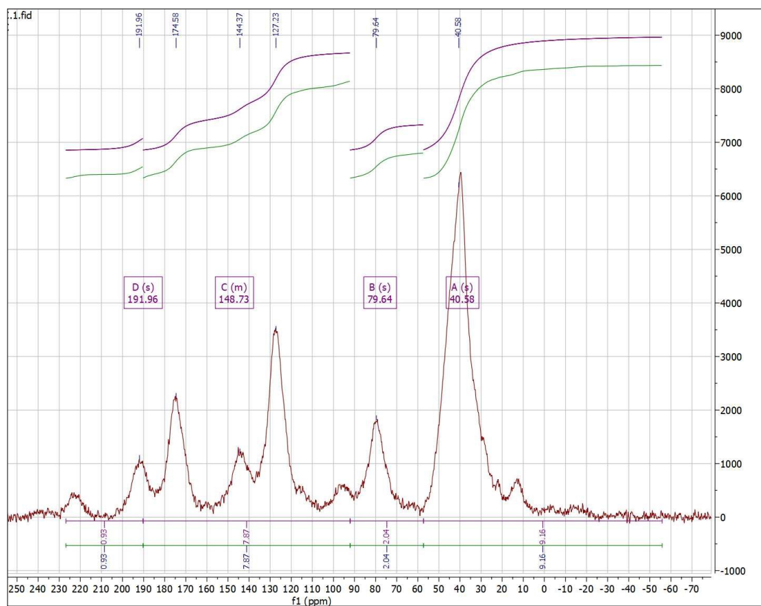
Figure S2: ^{13}\text{C} NMR spectra of prepared material.
