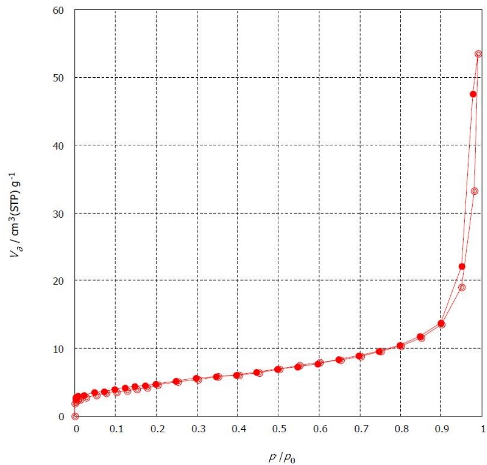
Figure S1. N_2 adsorption-desorption isotherm of prepared POPs.
