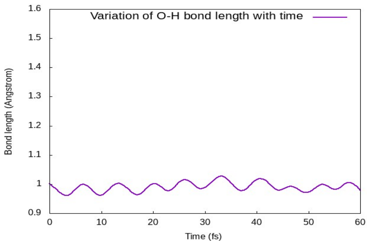
Fig. S1 Time evolution of the O-H distance of water molecule on (001) CsPbI 2 Br/H 2 O interface.
