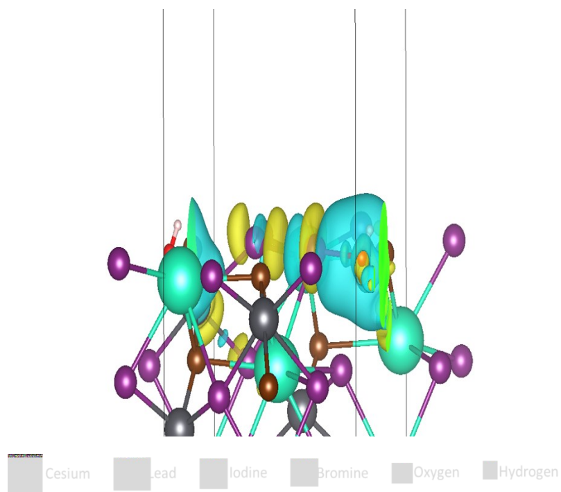
Fig S4 Charge density difference (CDD) plots of OH - on (a) (001) plane of CsPbI 2 Br and (b) (111) plane of CsPbI 2 Br
