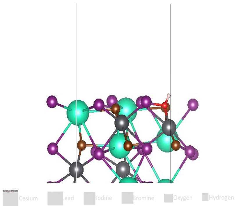
Fig S3 OH - adsorbed on the (a) (001) surface of CsPbI 2 Br and (b) (111) surface of CsPbI 2 Br
