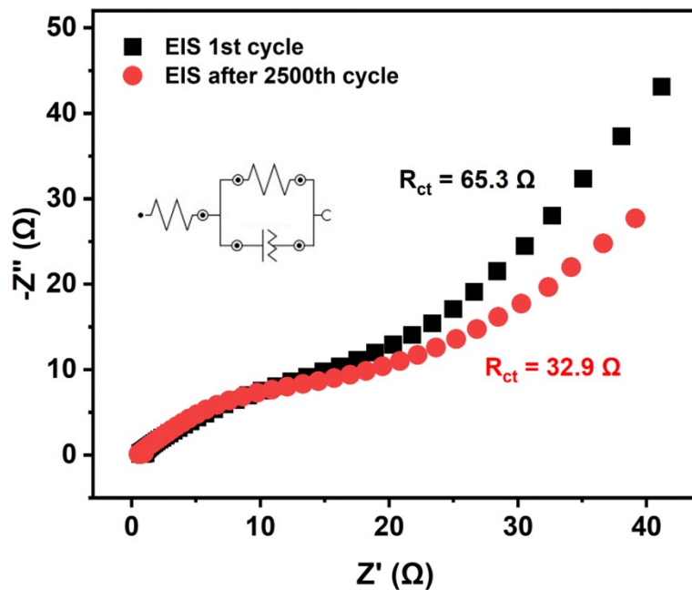
Figure S2. Nyquist plot of the prepared electrode before (black plots) and after 2500 cycles of Galvanostatic charge-discharge measurements in 3 M KOH solution (red plots).
