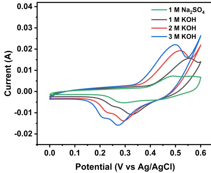
Figure S1. Cyclic voltammogram of mesoporous carbon on the surface of nickel foam electrode in the different electrolytes.
