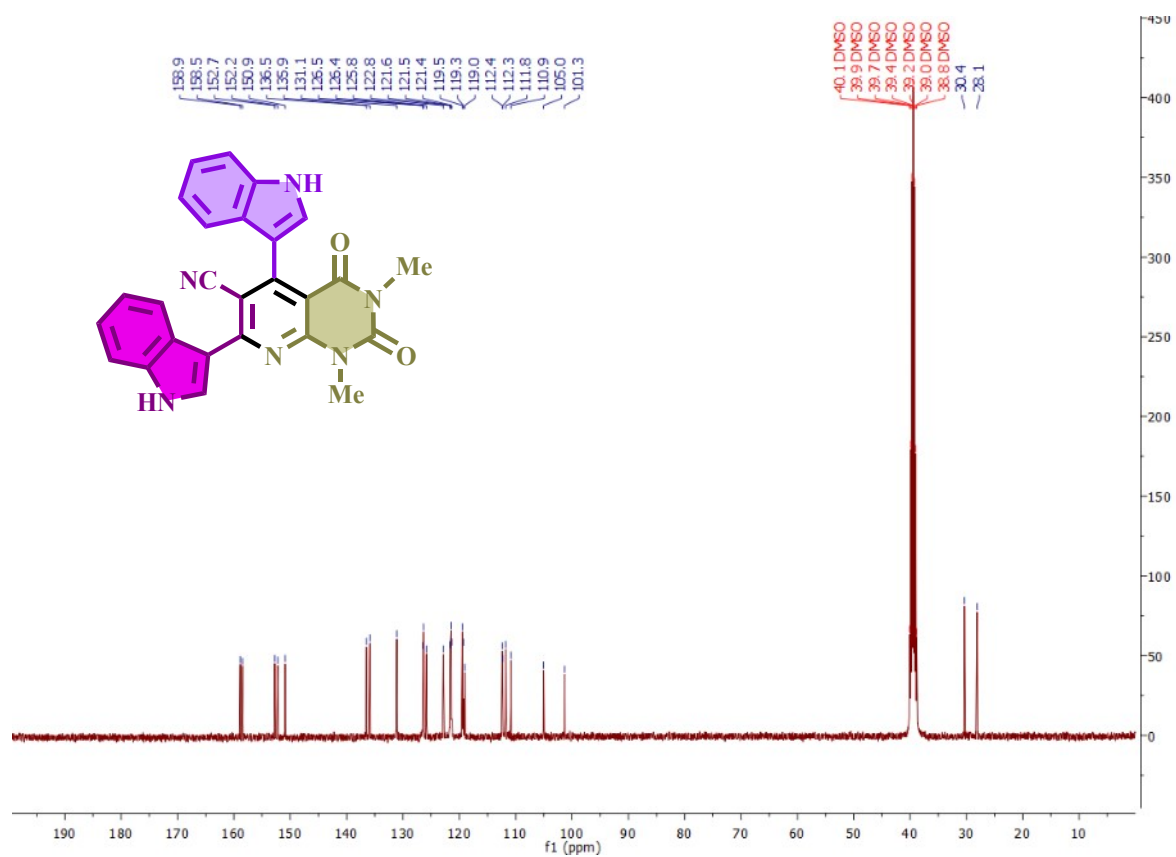
13 C-NMR spectrum of 5,7-di(1H-indol-3-yl)-1,3-dimethyl-2,4-dioxo-1,2,3,4-tetrahydropyrido[2,3-d]pyrimidine-6-carbonitrile(B10)
