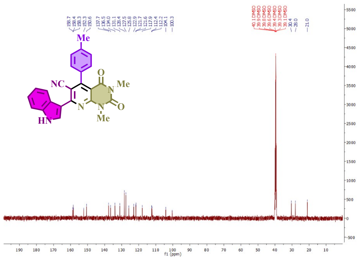
^{13}\text{C} -NMR spectrum of 7-(1H-indol-3-yl)-1,3-dimethyl-2,4-dioxo-5-(p-tolyl)-1,2,3,4-tetrahydropyrido[2,3-d]pyrimidine-6-carbonitrile (B9)
