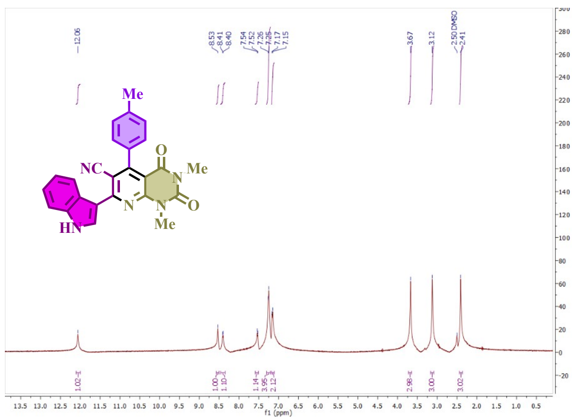
1 H-NMR spectrum of 7-(1H-indol-3-yl)-1,3-dimethyl-2,4-dioxo-5-(p-tolyl)-1,2,3,4-tetrahydropyrido[2,3-d]pyrimidine-6-carbonitrile (B9)
