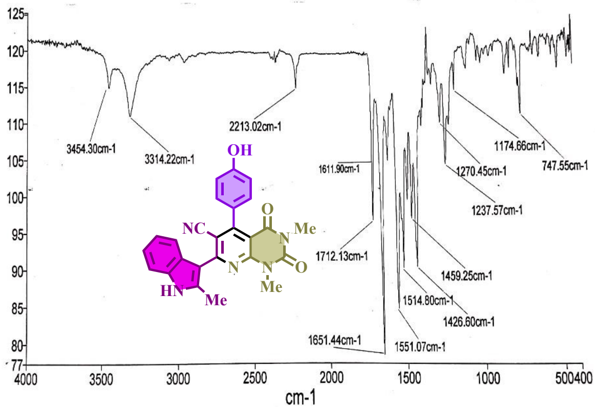
FT-IR spectrum of 5-(4-hydroxyphenyl)-1,3-dimethyl-7-(2-methyl-1H-indol-3-yl)-2,4-dioxo-1,2,3,4-tetrahydropyrido[2,3-d]pyrimidine-6-carbonitrile (C2)
