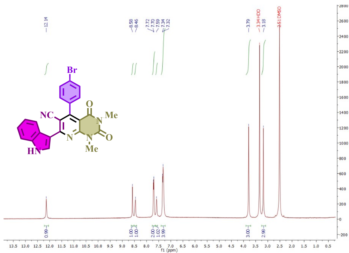
1 H-NMR spectrum of 5-(4-bromophenyl)-7-(1H-indol-3-yl)-1,3-dimethyl-2,4-dioxo-1,2,3,4-tetrahydropyrido[2,3-b]pyrimidine-6-carbonitrile (B3)
