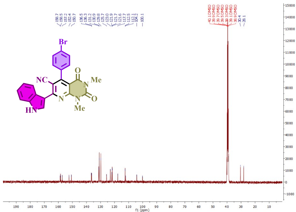
^{13}\text{C} -NMR spectrum of 5-(4-bromophenyl)-7-(1H-indol-3-yl)-1,3-dimethyl-2,4-dioxo-1,2,3,4-tetrahydropyrido[2,3-b]pyrimidine-6-carbonitrile (B3)
