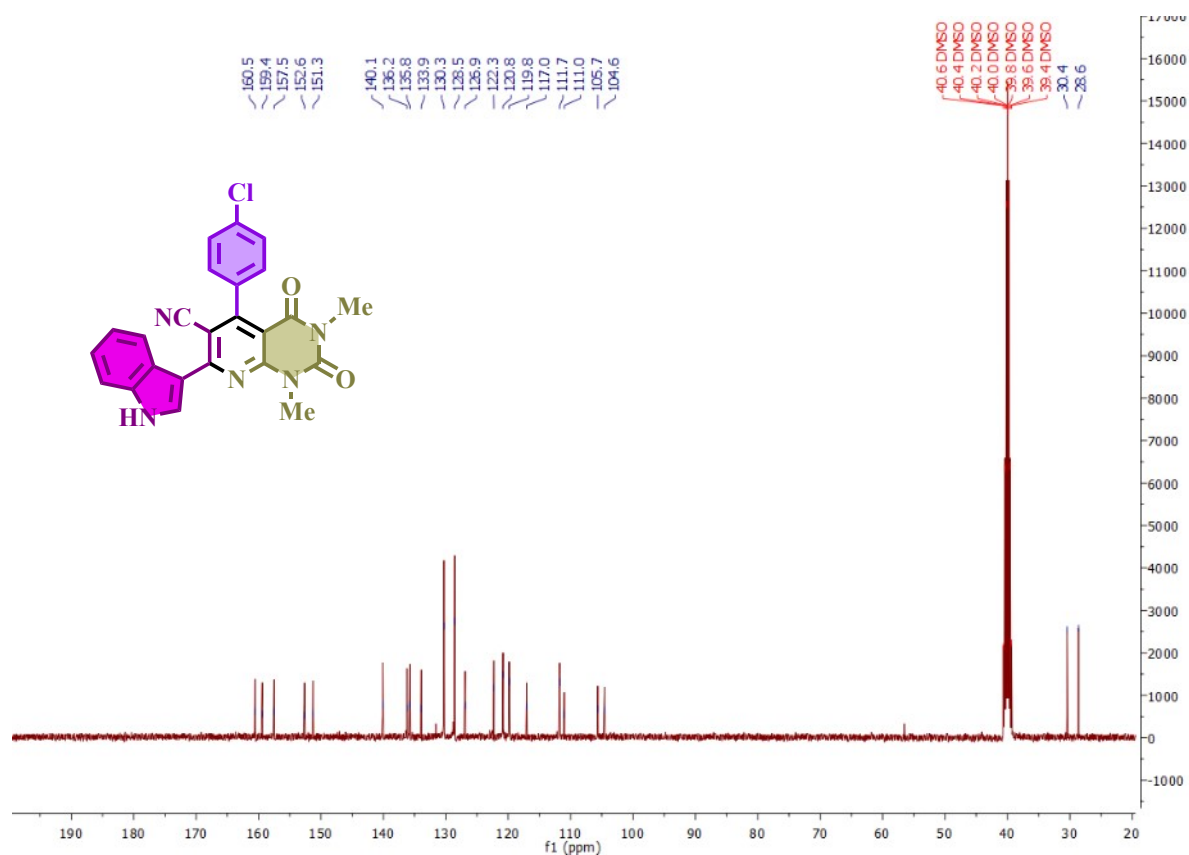
13 C-NMR spectrum of 5-(4-chlorophenyl)-7-(1H-indol-3-yl)-1,3-dimethyl-2,4-dioxo-1,2,3,4-tetrahydropyrido[2,3-d]pyrimidine-6-carbonitrile(B1)
