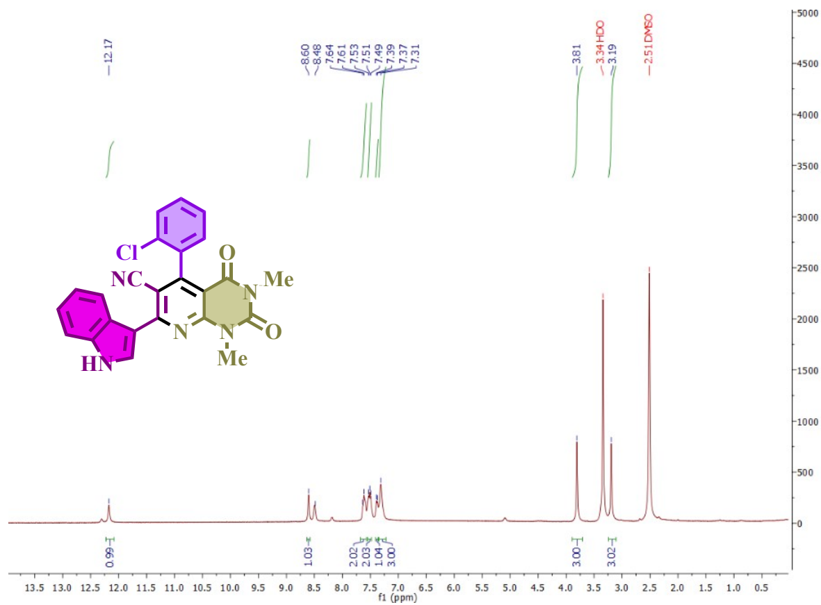
^1\text{H} -NMR spectrum of 5-(2-chlorophenyl)-7-(1H-indol-3-yl)-1,3-dimethyl-2,4-dioxo-1,2,3,4-tetrahydropyrido[2,3-d] pyrimidine-6-carbonitrile (B2)
