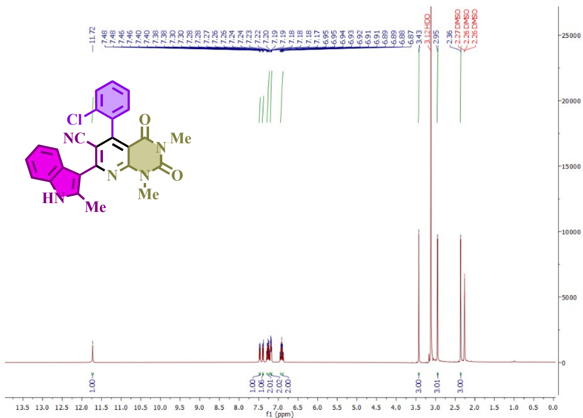
1 H-NMR spectrum of 5-(2-chlorophenyl)-7-(1H-indol-3-yl)-1,3-dimethyl-2,4-dioxo-1,2,3,4-tetrahydropyrido[2,3-d]pyrimidine-6-carbonitrile (C5)
