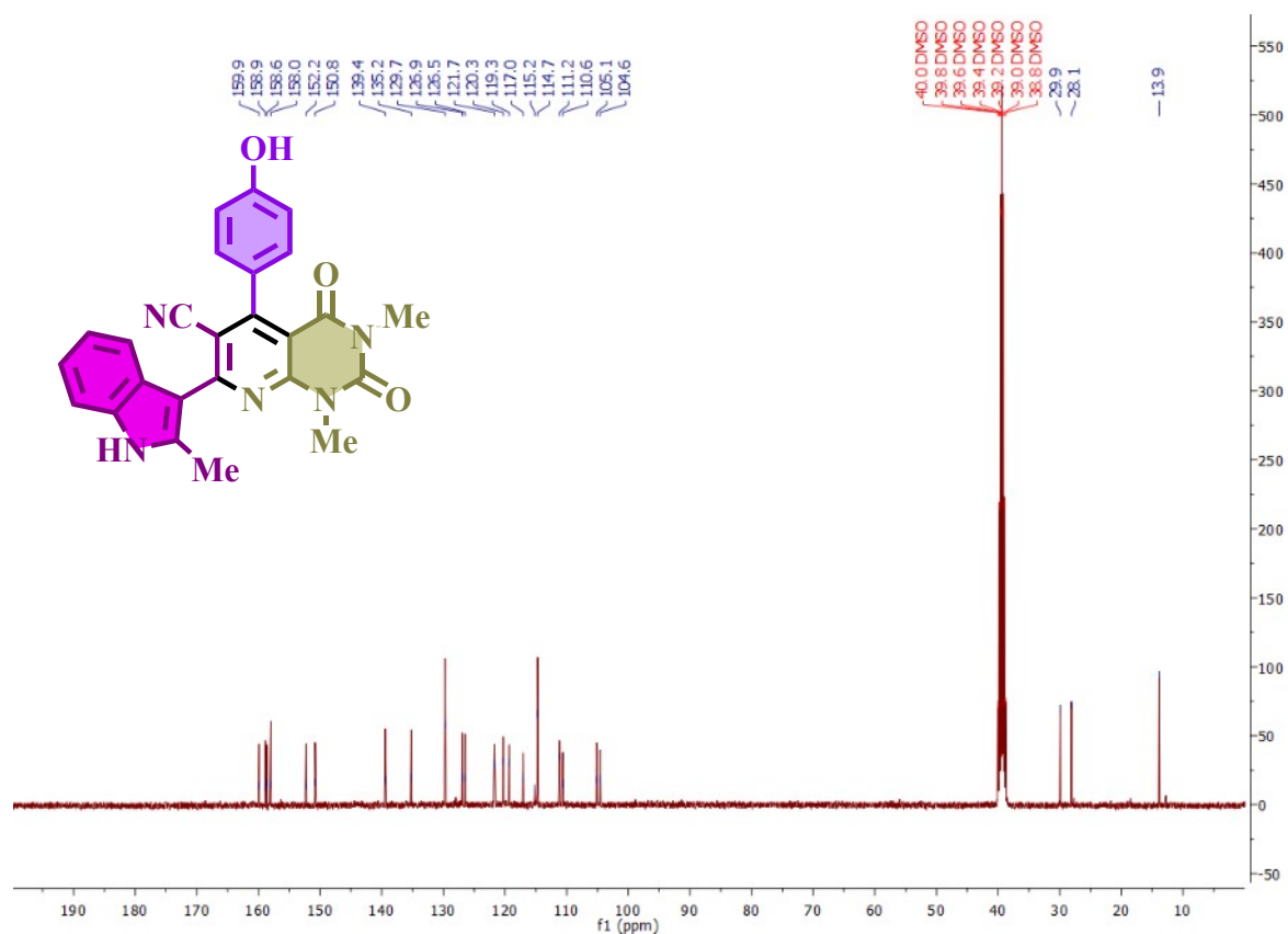
13 C-NMR spectrum of 5-(4-hydroxyphenyl)-1,3-dimethyl-7-(2-methyl-1H-indol-3-yl)-2,4-dioxo-1,2,3,4-tetrahydropyrido[2,3-d]pyrimidine-6-carbonitrile (C2)
