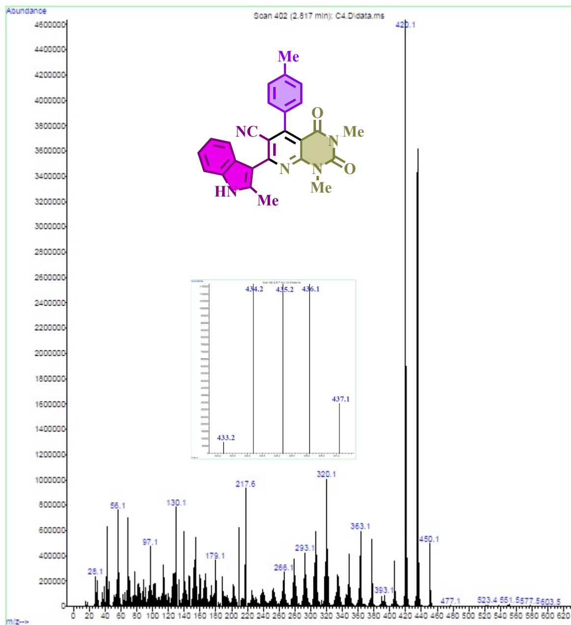
Mass spectrum of 1,3-dimethyl-7-(2-methyl-1H-indol-3-yl)-2,4-dioxo-5-(p-tolyl)-1,2,3,4-tetrahydropyrido[2,3-d]pyrimidine-6-carbonitrile (C4)
