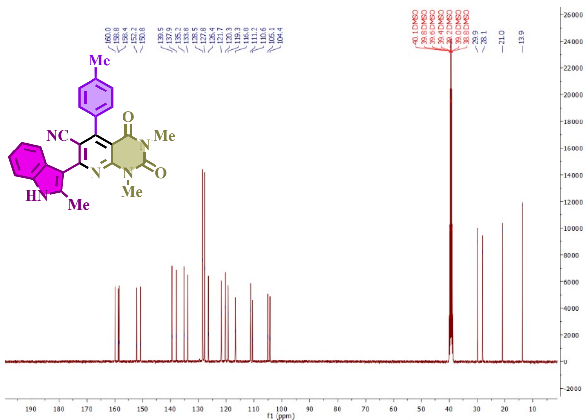
13 C-NMR spectrum of 1,3-dimethyl-7-(2-methyl-1H-indol-3-yl)-2,4-dioxo-5-(p-tolyl)-1,2,3,4-tetrahydropyrido[2,3-d]pyrimidine-6-carbonitrile (C4)
