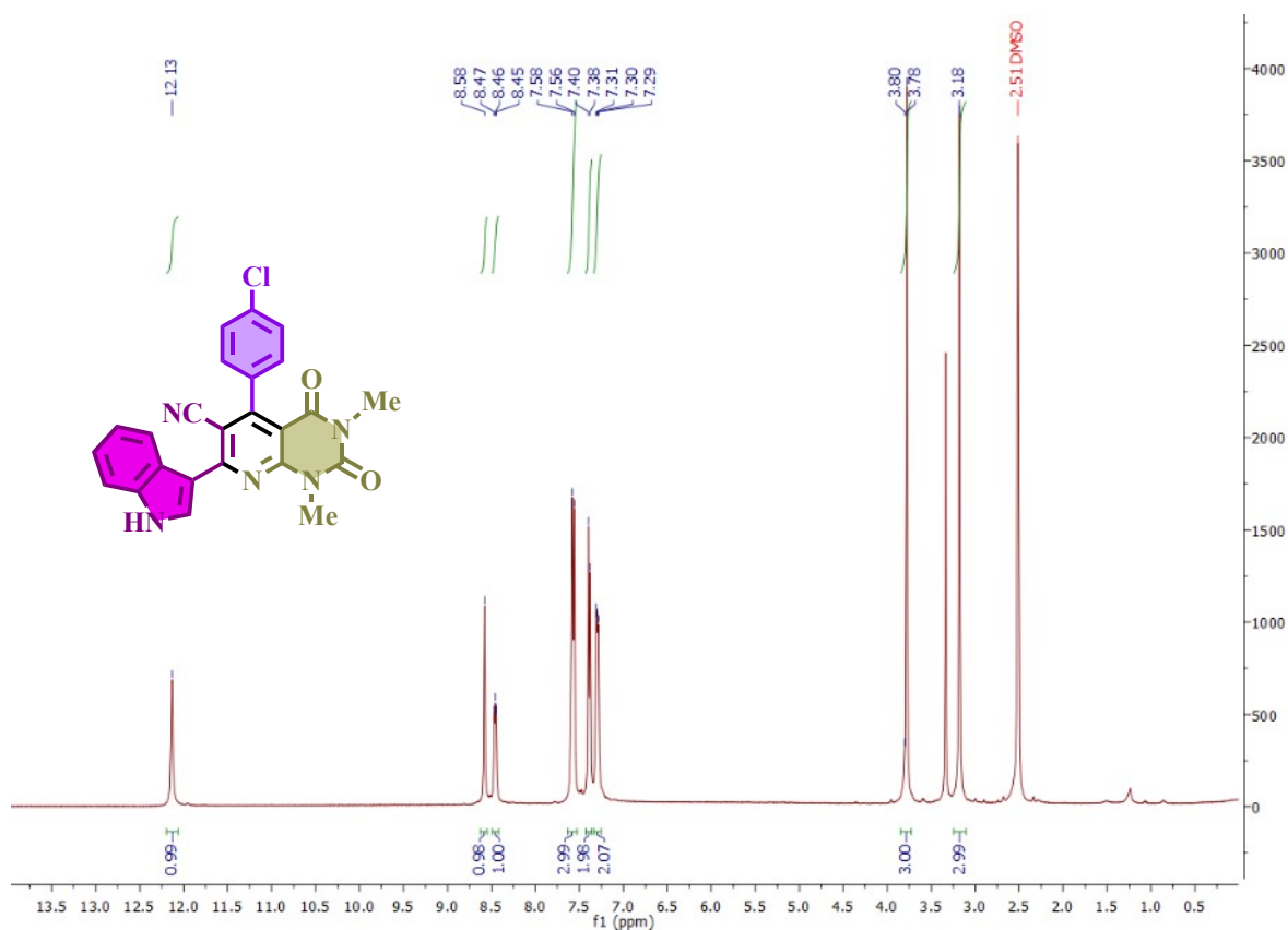
^1\text{H} -NMR spectrum of 5-(4-chlorophenyl)-7-(1H-indol-3-yl)-1,3-dimethyl-2,4-dioxo-1,2,3,4-tetrahydropyrido[2,3-d]pyrimidine-6-carbonitrile(B1)
