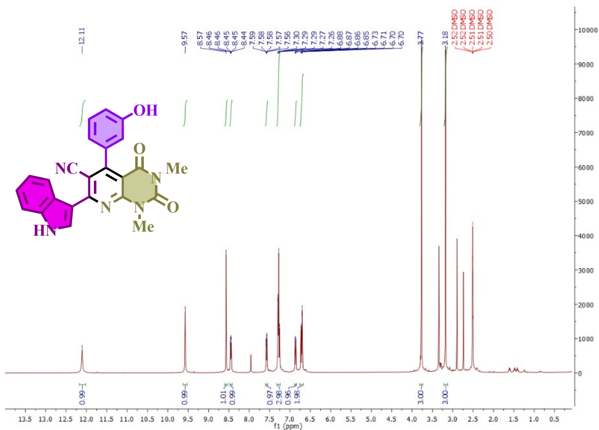
1 H-NMR spectrum of 5-(3-hydroxyphenyl)-7-(1H-indol-3-yl)-1,3-dimethyl-2,4-dioxo-1,2,3,4-tetrahydropyrido[2,3-d]pyrimidine-6-carbonitrile (B5)
