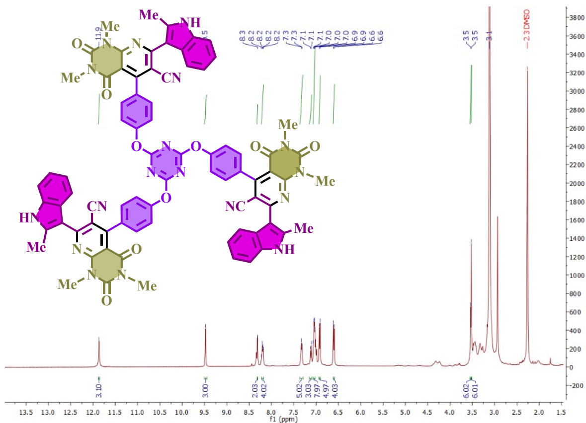
1 H-NMR spectrum of 5,5',5''-(((1,3,5-triazine-2,4,6-triyl)tris(oxy))tris(benzene-4,1-diyl))tris(7-(1H-indol-3-yl)-1,3-dimethyl-2,4-dioxo-1,2,3,4-tetrahydropyrido[2,3-d]pyrimidine-6-carbonitrile) (C7)
