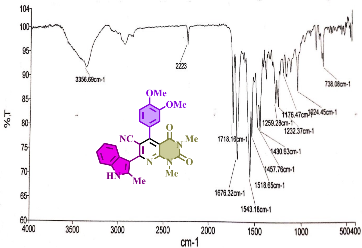
FT-IR spectrum of 5-(3,4-dimethoxyphenyl)-1,3-dimethyl-7-(2-methyl-1H-indol-3-yl)-2,4-dioxo-1,2,3,4-tetrahydropyrido[2,3-d]pyrimidine-6-carbonitrile (C6)
