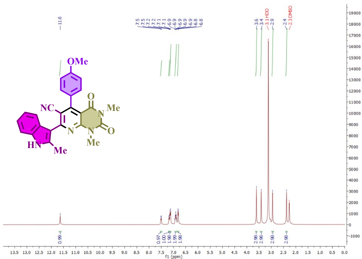
^1\text{H} -NMR spectrum of 5-(4-methoxyphenyl)-1,3-dimethyl-7-(2-methyl-1H-indol-3-yl)-2,4-dioxo-1,2,3,4-tetrahydropyrido[2,3-d]pyrimidine-6-carbonitrile (C3)
