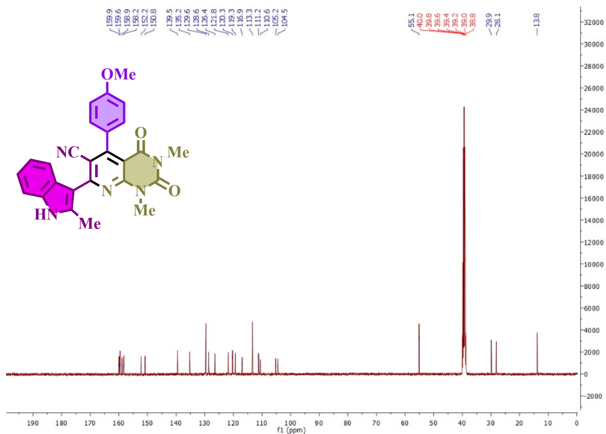
^{13}\text{C} -NMR spectrum of 5-(4-methoxyphenyl)-1,3-dimethyl-7-(2-methyl-1H-indol-3-yl)-2,4-dioxo-1,2,3,4-tetrahydropyrido[2,3-d]pyrimidine-6-carbonitrile (C3)
