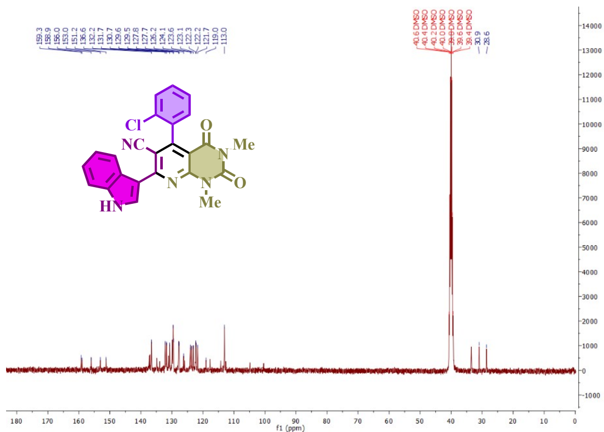
13 C-NMR spectrum of 5-(2-chlorophenyl)-7-(1H-indol-3-yl)-1,3-dimethyl-2,4-dioxo-1,2,3,4-tetrahydropyrido[2,3-d] pyrimidine-6-carbonitrile (B2)
