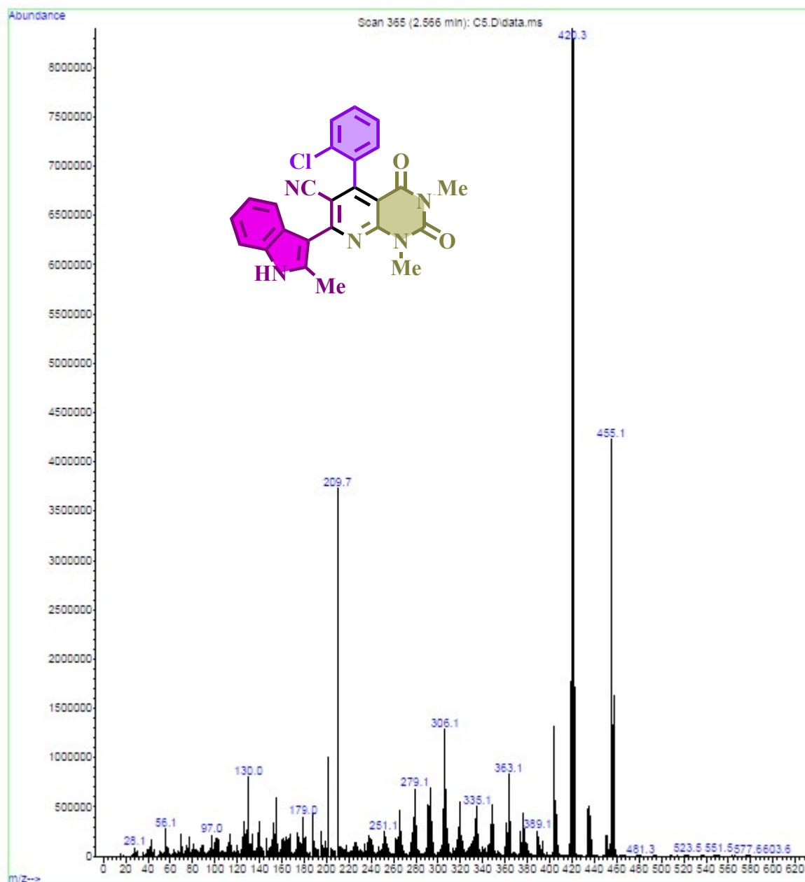
Mass spectrum of 5-(2-chlorophenyl)-7-(1H-indol-3-yl)-1,3-dimethyl-2,4-dioxo-1,2,3,4-tetrahydropyrido[2,3-d]pyrimidine-6-carbonitrile (C5)
