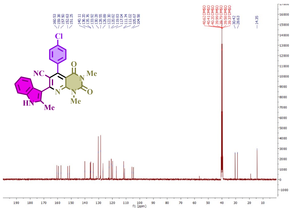
^{13}\text{C} -NMR spectrum of 5-(4-chlorophenyl)-1,3-dimethyl-7-(2-methyl-1H-indol-3-yl)-2,4-dioxo-1,2,3,4-tetrahydropyrido[2,3-d]pyrimidine-6-carbonitrile (C1)
