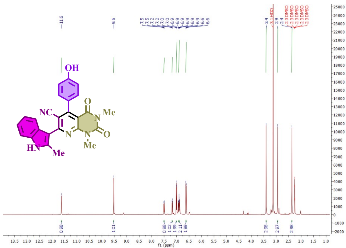
1 H-NMR spectrum of 5-(4-hydroxyphenyl)-1,3-dimethyl-7-(2-methyl-1H-indol-3-yl)-2,4-dioxo-1,2,3,4-tetrahydropyrido[2,3-d]pyrimidine-6-carbonitrile (C2)
