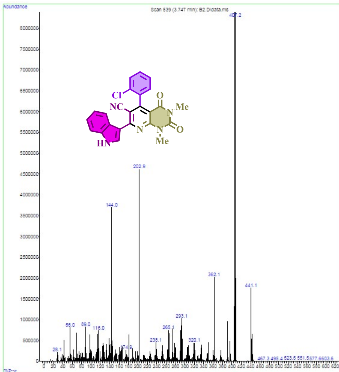
Mass spectrum of 5-(2-chlorophenyl)-7-(1H-indol-3-yl)-1,3-dimethyl-2,4-dioxo-1,2,3,4-tetrahydropyrido[2,3-d] pyrimidine-6-carbonitrile (B2)
