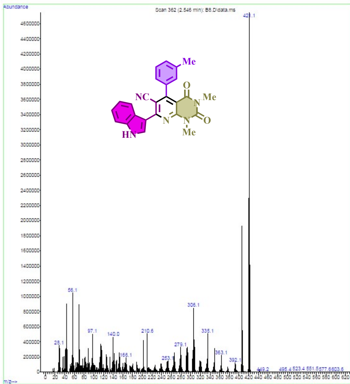
Mass spectrum of 7-(1H-indol-3-yl)-1,3-dimethyl-2,4-dioxo-5-(m-tolyl)-1,2,3,4-tetrahydropyrido[2,3-d]pyrimidine-6-carbonitrile (B8)
