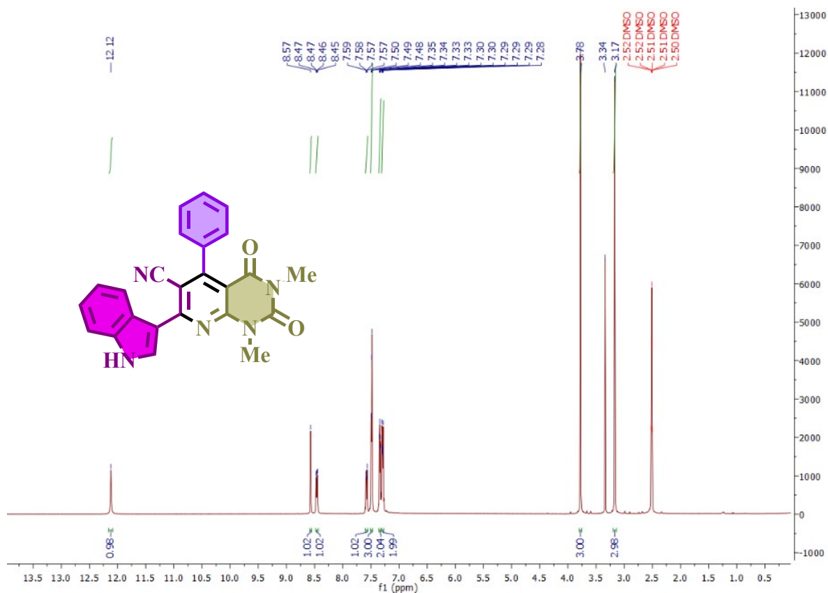
1 H-NMR spectrum of 7-(1H-indol-3-yl)-1,3-dimethyl-2,4-dioxo-5-phenyl-1,2,3,4-tetrahydropyrido[2,3-d]pyrimidine-6-carbonitrile (B4)
