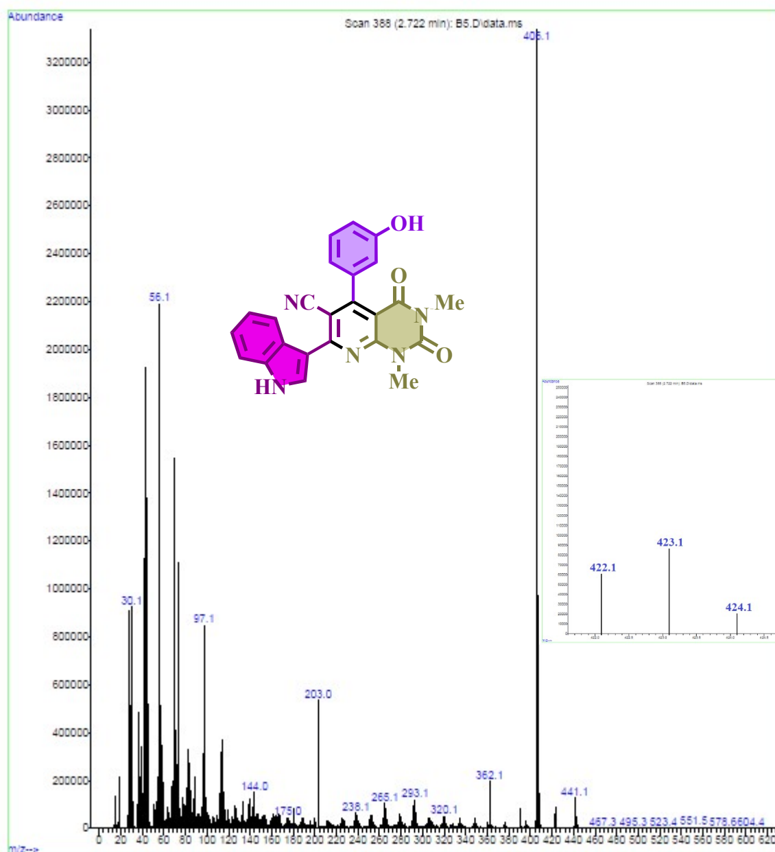
Mass spectrum of 5-(3-hydroxyphenyl)-7-(1H-indol-3-yl)-1,3-dimethyl-2,4-dioxo-1,2,3,4-tetrahydropyrido[2,3-d]pyrimidine-6-carbonitrile (B5)
