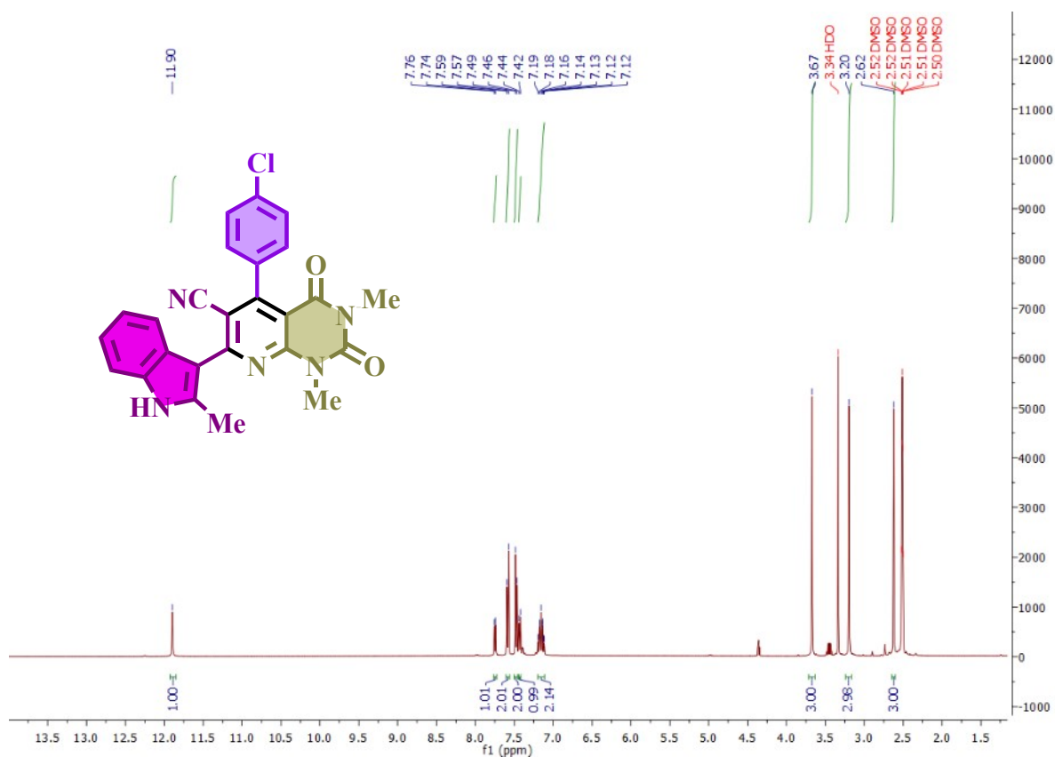
1 H-NMR spectrum of 5-(4-chlorophenyl)-1,3-dimethyl-7-(2-methyl-1H-indol-3-yl)-2,4-dioxo-1,2,3,4-tetrahydropyrido[2,3-d]pyrimidine-6-carbonitrile (C1)
