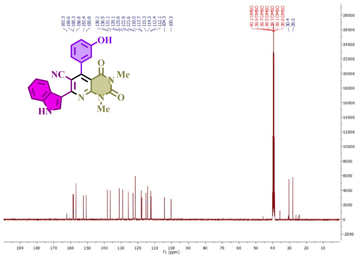
^{13}\text{C} -NMR spectrum of 5-(3-hydroxyphenyl)-7-(1H-indol-3-yl)-1,3-dimethyl-2,4-dioxo-1,2,3,4-tetrahydropyrido[2,3-d]pyrimidine-6-carbonitrile (B5)
