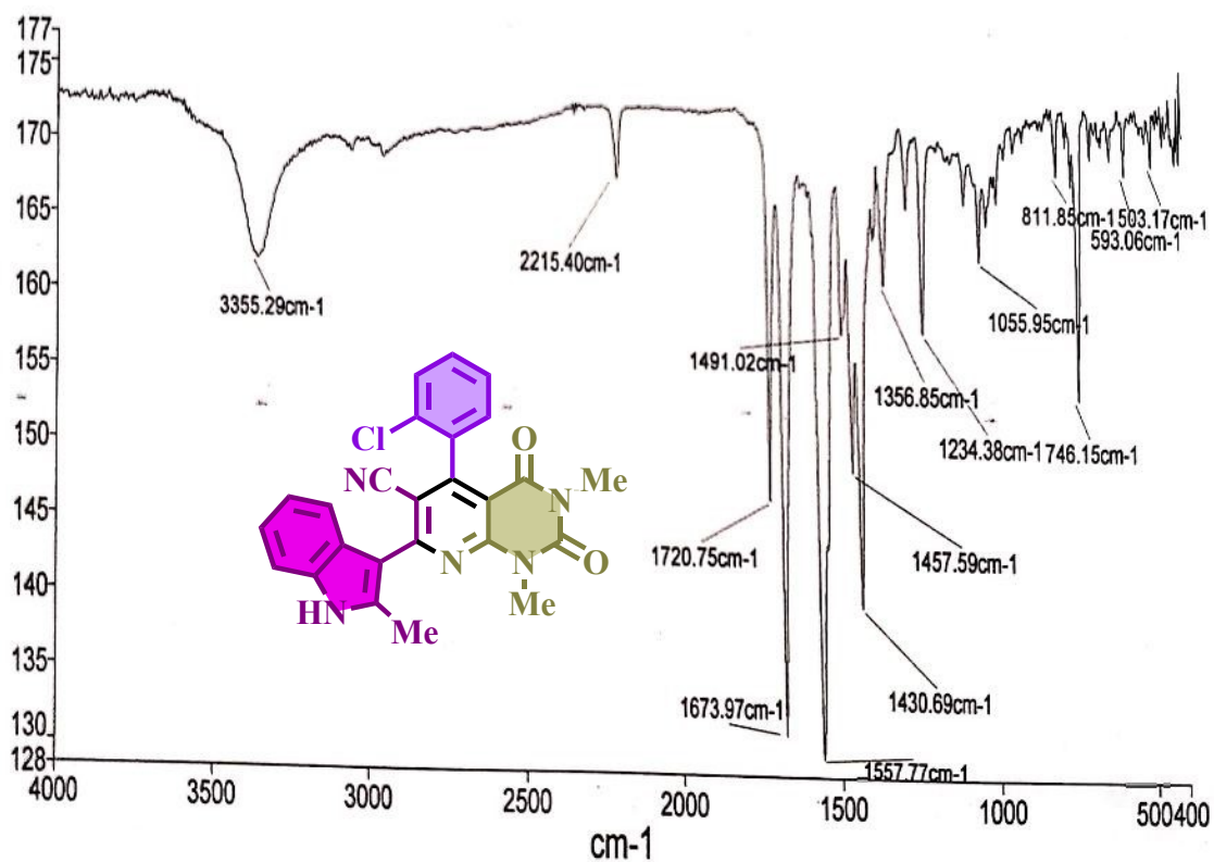
FT-IR spectrum of 5-(2-chlorophenyl)-7-(1H-indol-3-yl)-1,3-dimethyl-2,4-dioxo-1,2,3,4-tetrahydropyrido[2,3-d]pyrimidine-6-carbonitrile (C5)
