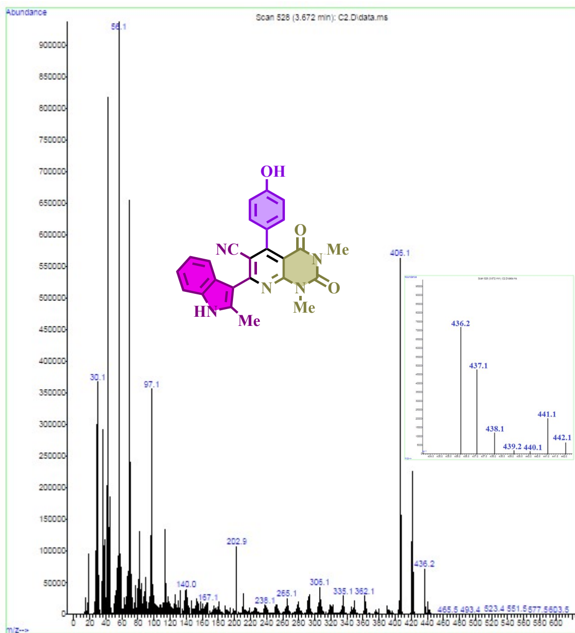
Mass spectrum of 5-(4-hydroxyphenyl)-1,3-dimethyl-7-(2-methyl-1H-indol-3-yl)-2,4-dioxo-1,2,3,4-tetrahydropyrido[2,3-d]pyrimidine-6-carbonitrile (C2)
