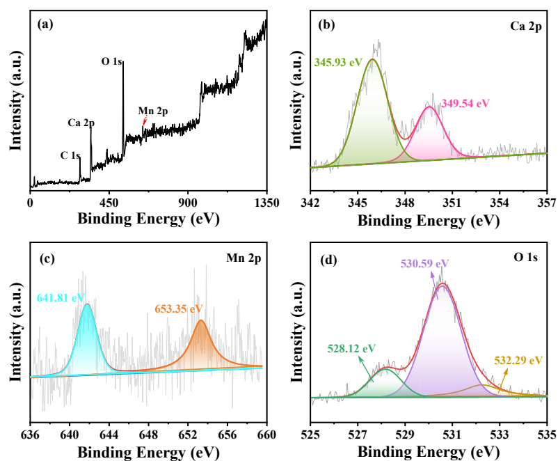
Fig. S1 XPS measurement spectra of 50%FA-100:10 Mn after 10 cycles: (a) XPS full spectrum, (b) XPS spectra of Ca 2p, (c) XPS spectra of Mn 2p and (d) XPS spectra of O 1s.
