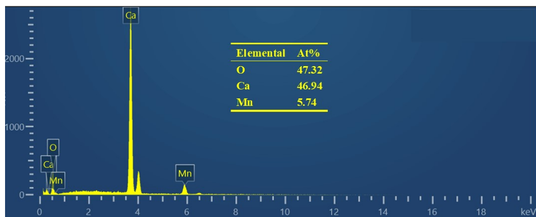
Fig. S2 Elemental mapping line scan image after 10 cycles of material 50FA-100:10 Mn
