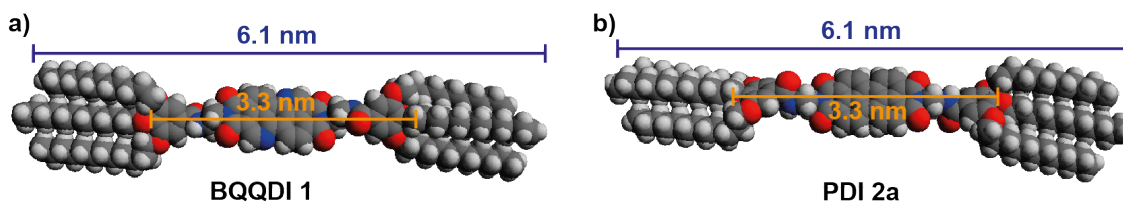
Figure SM2. Optimized geometry for the monomeric units of BQQDI 1 (a) and PDI 2 (b) showing the distances of the aromatic core, including the benzoate groups, and the complete molecule.
