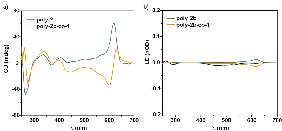
Figure SM1. a) CD and b) LD spectra of poly-2b and poly-2b-co-1 (experimental conditions: MCH/DCE 7/3 as solvent, c_T = 10 \mu\text{M} ).
