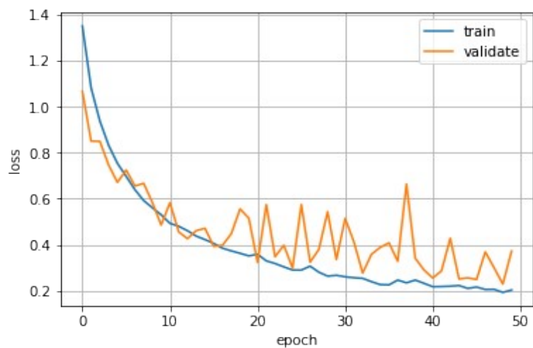
Figure S1: The loss function evaluated at each epoch of training the multiphase inception classifier, for both the training and validation data.
