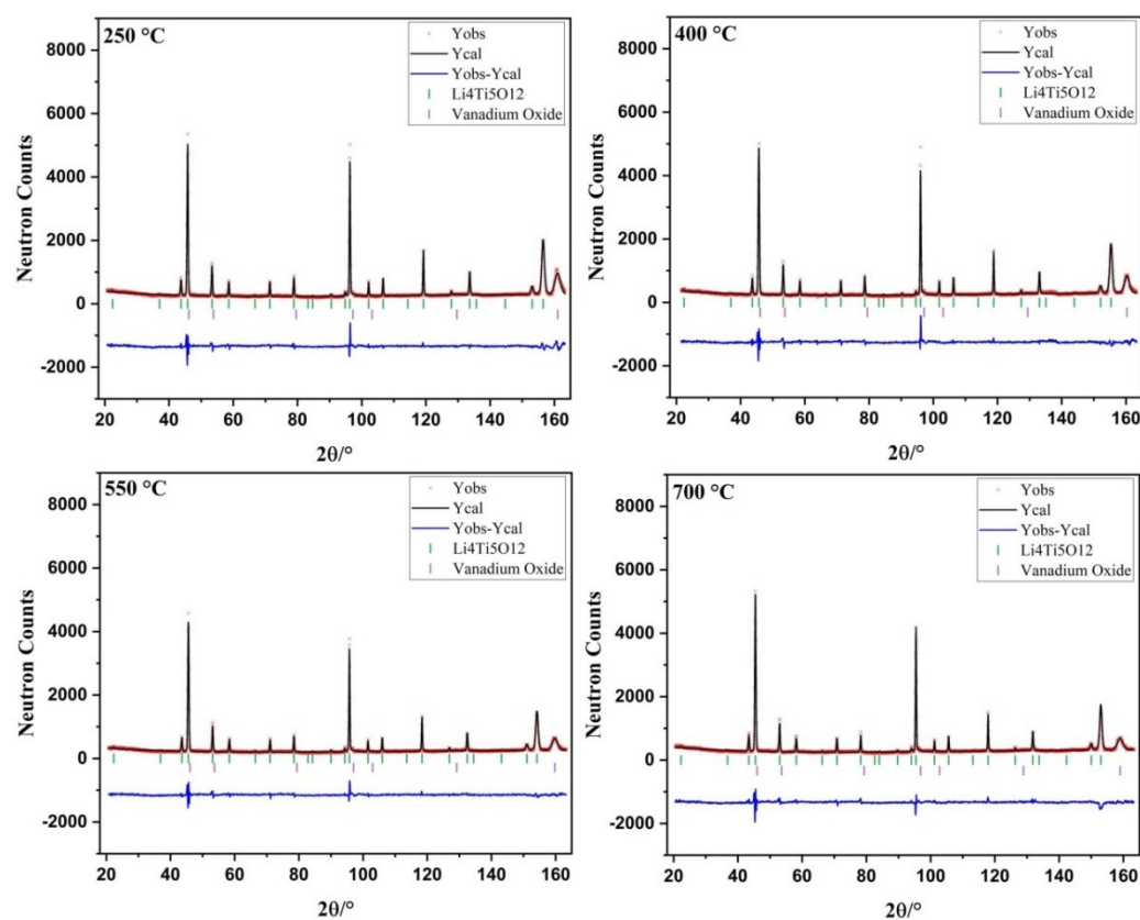
Figure S1. Rietveld refinement plots of \text{Li}_4\text{Ti}_5\text{O}_{12} at high temperature.
