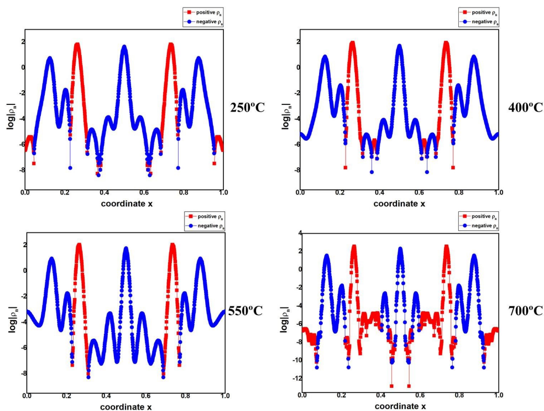
Figure S2. Nuclear density distribution of \text{Li}_4\text{Ti}_5\text{O}_{12} from fractional Cartesian coordinate (0,0,0) to (1,1,1) at 250 °C, 400 °C, 550 °C, 700 °C.
