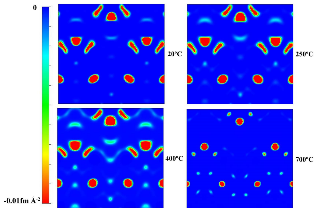
Figure S3. Two-dimensional scattering density map at (101) face of \text{Li}_4\text{Ti}_5\text{O}_{12} at 20 °C, 250 °C, 400 °C, 700 °C.
