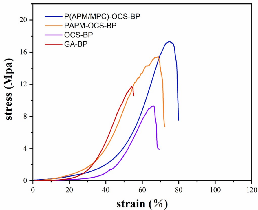
S2. Stress-strain curve of GA-BP, OCS-BP, PAM-OCS-BP, and P(APM/MPC)-OCS-BP.
