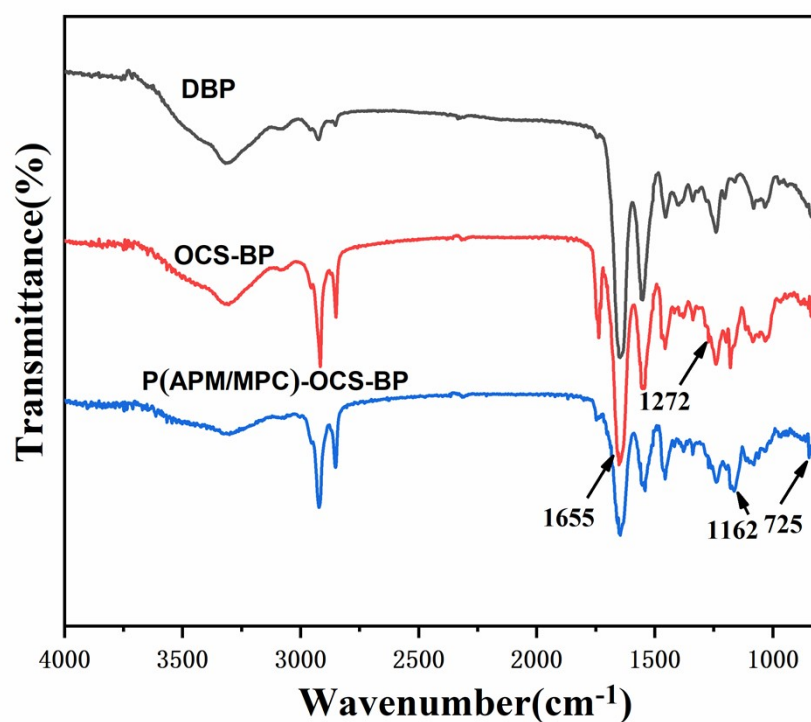
S1. FTIR spectra of DBP, OCS-BP, and P(APM/MPC)-OCS-BP.
