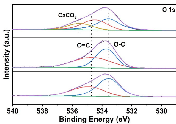
Fig. s1 High-resolution XPS spectra of O 1s.
