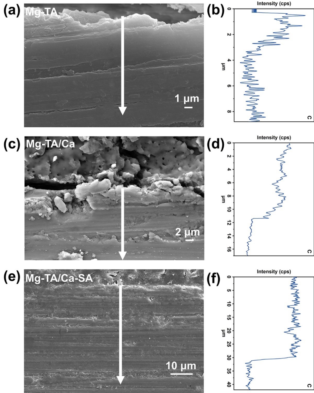
Fig. s2. (a), (c) and (e) Cross-sectional SEM morphology; (b), (d), (f) EDS line scanning results.
