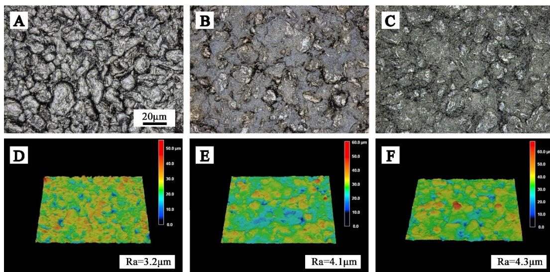
Fig. S1 LCM images of PEEK (A,D), PHC (B,E) and PBHC (C,F).
