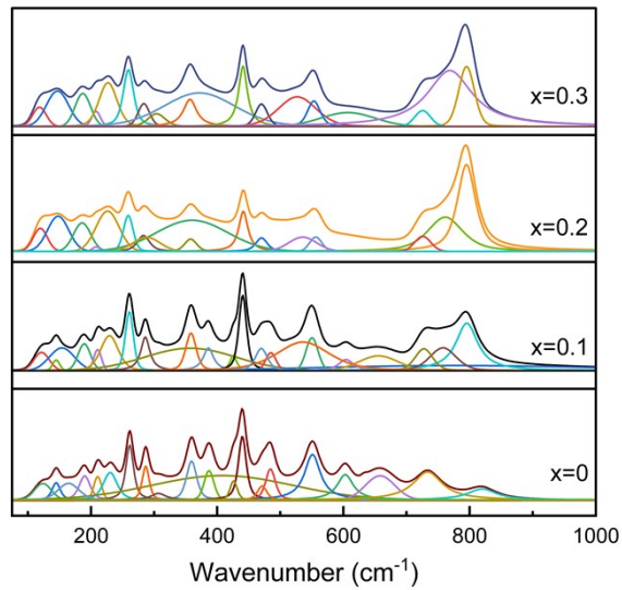
Figure SI 2. Raman fitted data for individual sample (1-x)CZT-xCZN were shown.
