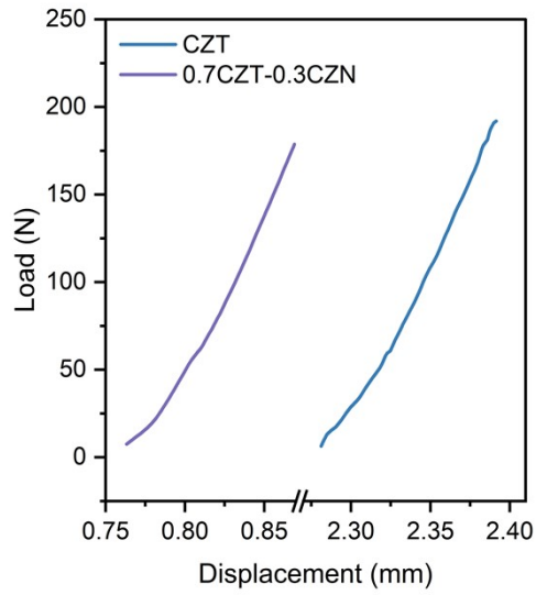
Figure SI 1. Flexural load-displacement curves of CZT (blue line) and 0.7CZT-0.3CZN (purple line) were shown.
