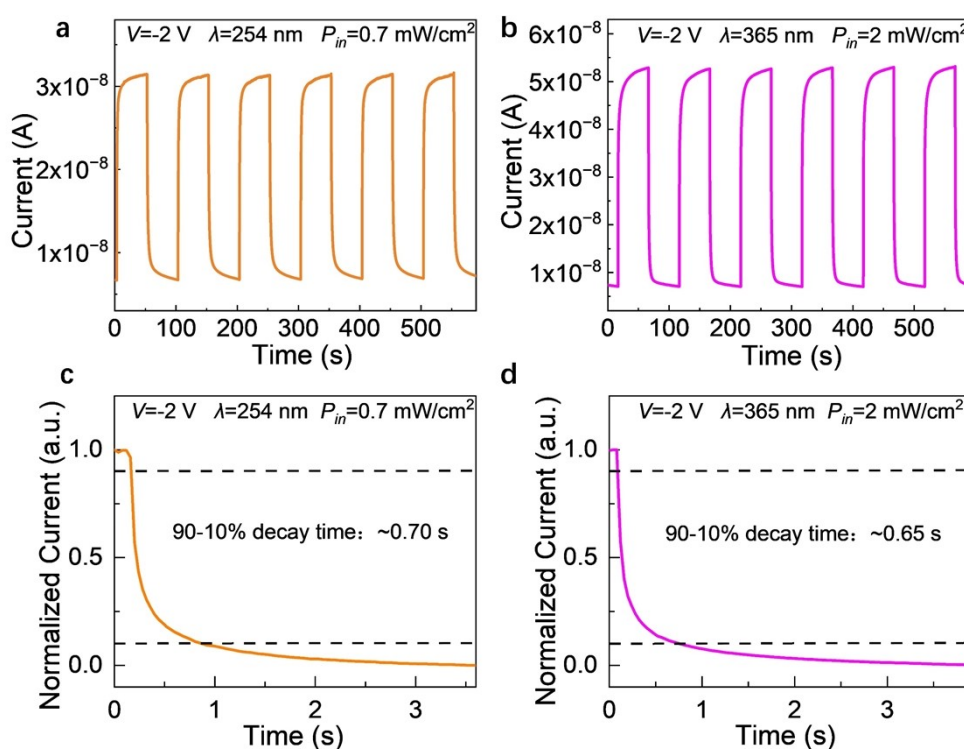
Figure S1: The I - t curves of ZnO-a-Ga 2 O 3 core-shell microwire under (a) 254 nm and (b) 365 nm light illumination at -2 V. The normalized decay edges under (c) 254 nm light illumination and (d) 365 nm light illumination at -2 V.
