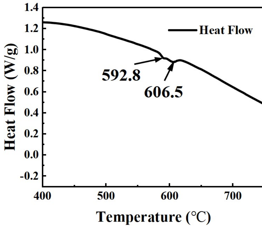
Fig. S1. DSC curves of Nd-Fe-Ga alloy.
