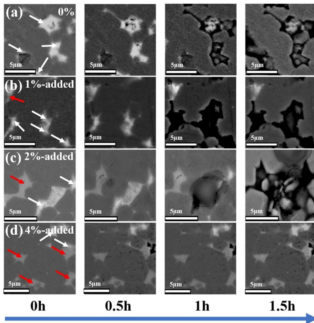
Fig. S2. Corrosion morphology evolution of different phases for the investigated magnets with different Nd-Fe-Ga addition after immersing in 3.5% NaCl solution varying for different times. In-situ images in the local area for 0 (a), 1% (b), 2% (c) and 4% addition(d) ranging from 0 to 90 min.
