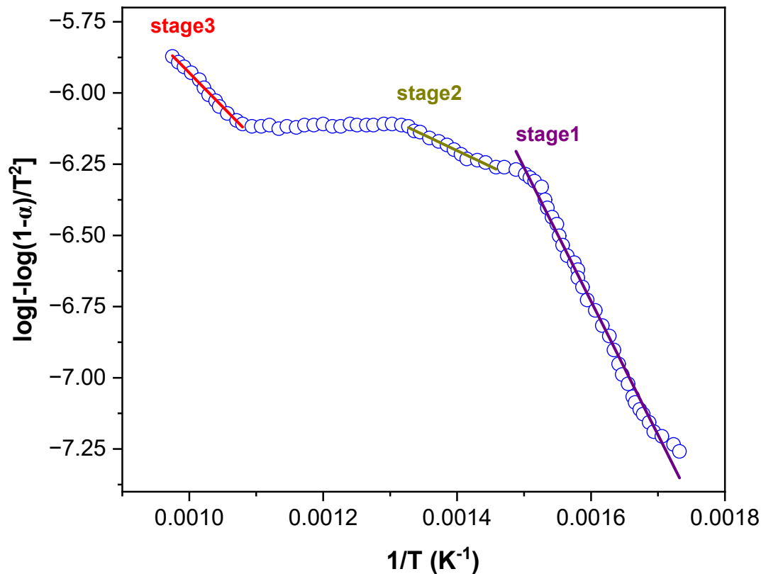
Figure S1. Coats-Redfern relationship for poly(AN-co-AMPS).
