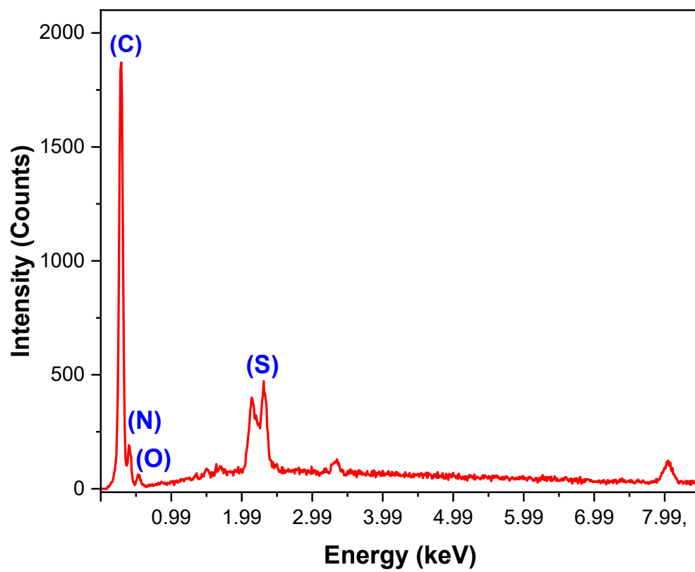
Figure S2. EDX analysis of poly(AN-co-AMPS).
