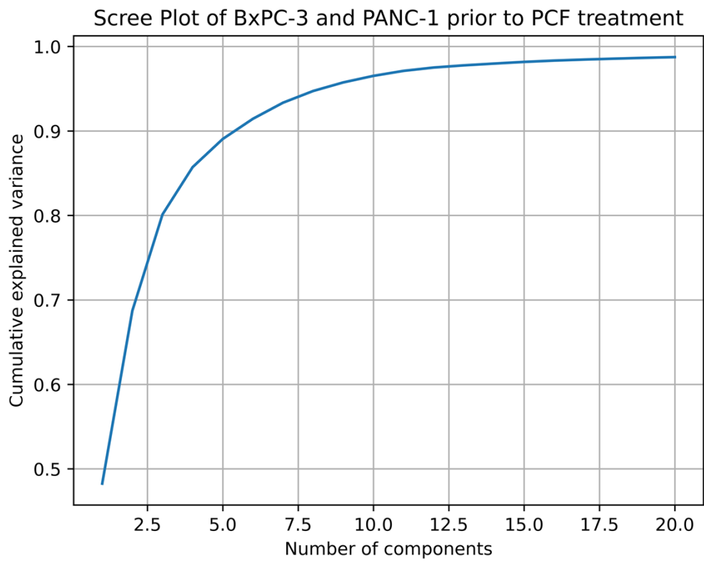
Figure S3a: Scree plot of Raman data for BxPC-3 and PANC-1 prior to PCF exposure.
