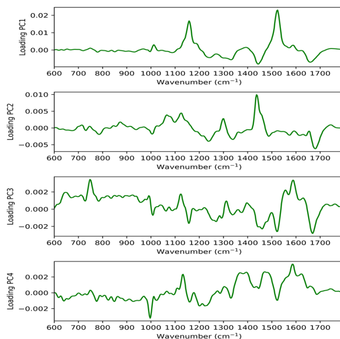
Figure S6: Loadings plot of Raman data comparing BxPC-3 with PANC-1 cells post PCF-treatment.
