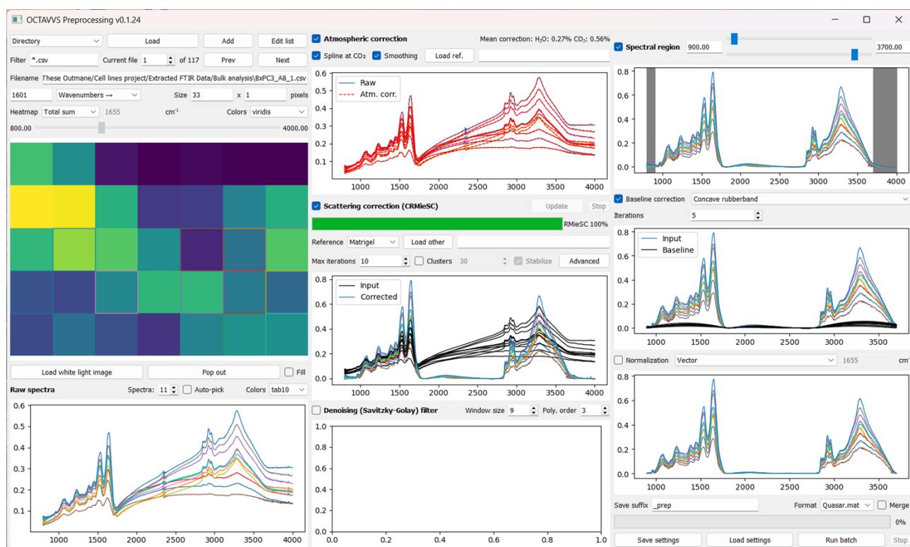
Figure S2: An example of preprocessing steps of FTIR images performed on BxPC-3 and PANC-1 cells in OCTAVVS preprocessing after background removal using Kmeans clustering.
