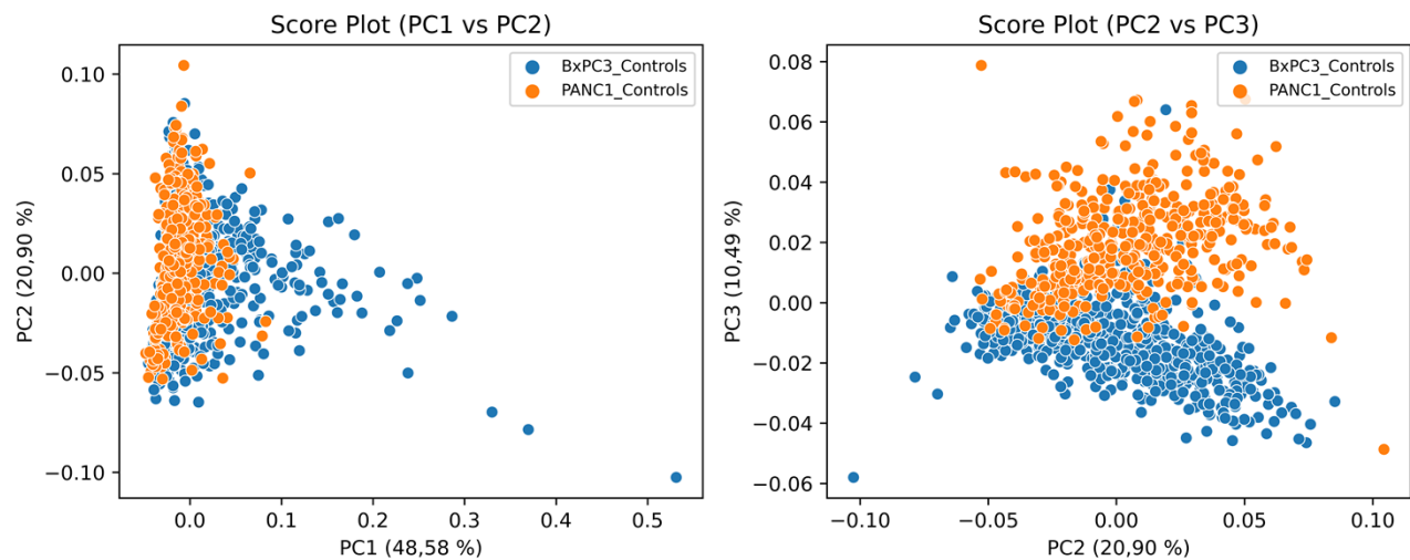
Figure S3b: Scores plot of Raman data for BxPC-3 and PANC-1 prior to PCF exposure.
