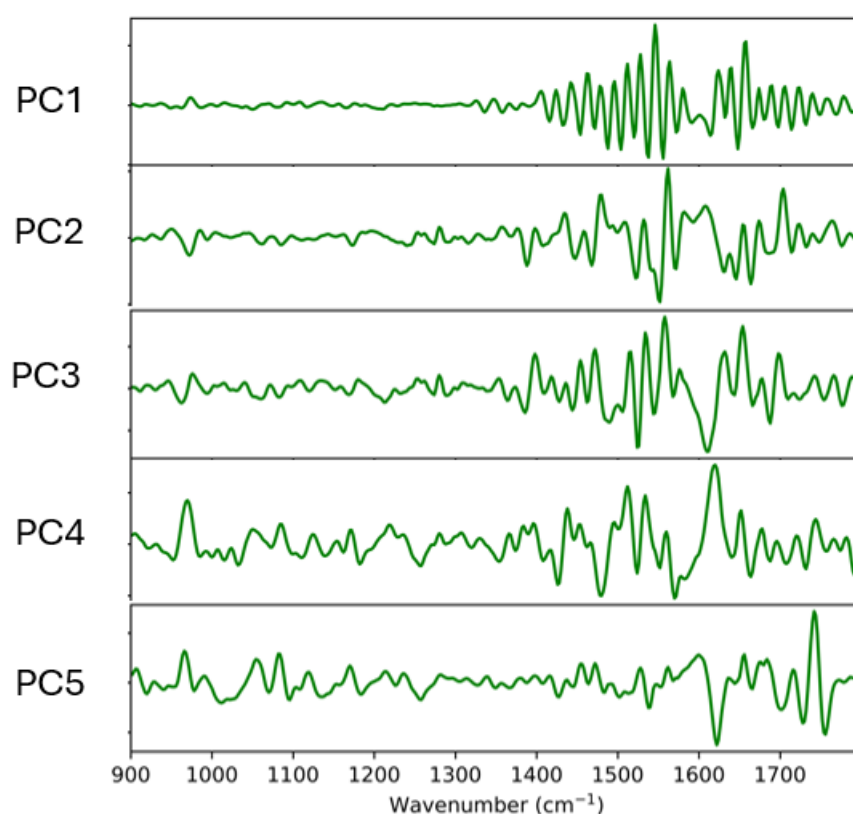
Figure S4b: Loading plot for FTIR data of BxPC-3 and PANC-1 cells pre-exposure to PCF.
