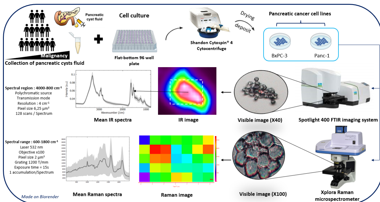
Figure S1: Experimental workflow of this study.
