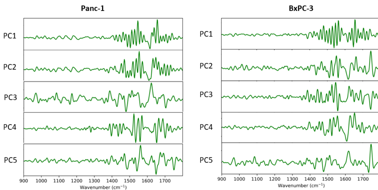
Figure S5: Loadings plot for FTIR of BxPC-3 and PANC-1 cells post-exposure to PCF.
