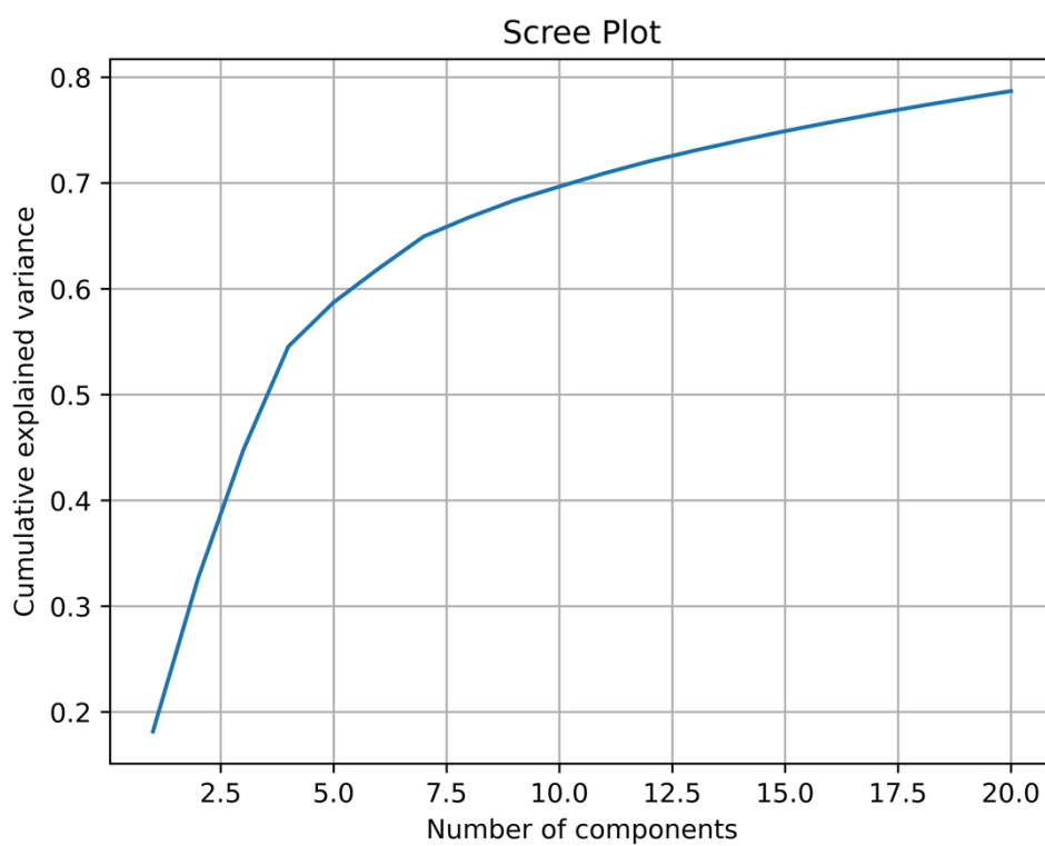
Figure S4a: Scree plot of FTIR data for BxPC-3 and PANC-1 prior to PCF exposure.
