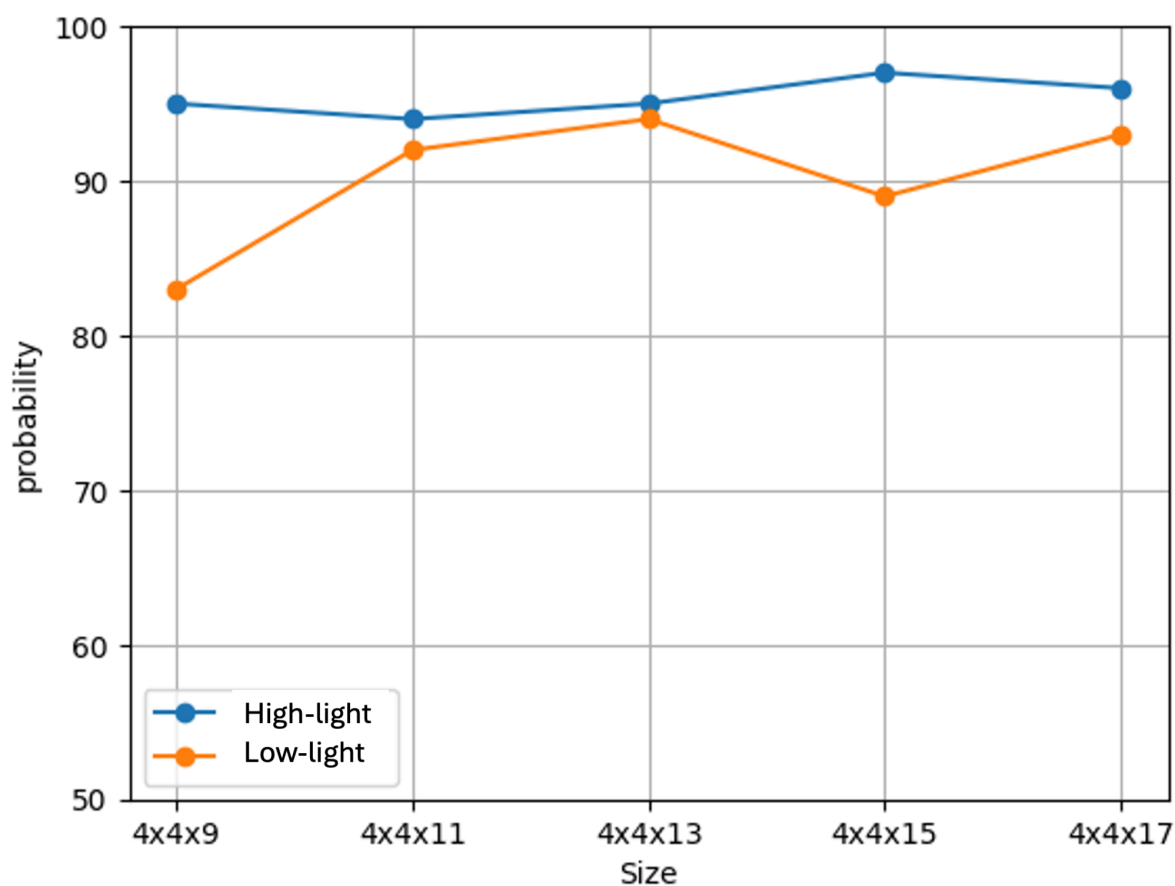
Figure X1: Dependence of CNN classification probabilities for high-light (HL) and low-light (LL) samples on time bin count n=4,5,6,7,8 .
