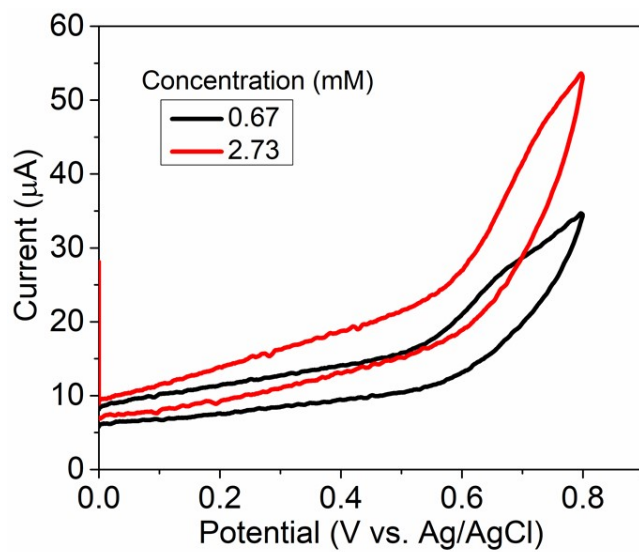
Fig. S2. Cyclic voltammograms for the lower and higher concentration of cartab at CNTs fiber.
