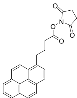
Figure S1. The chemical structure of PASE
