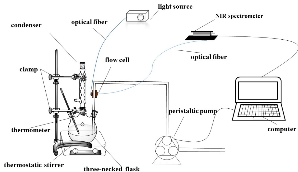
Fig. S1 Schemes of the experimental setups for aspirin synthesis and spectral measurement
