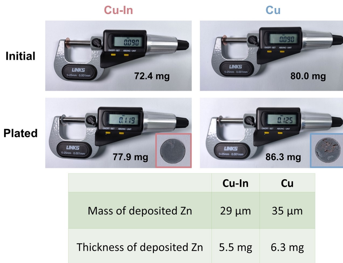
Fig. S4 Details on the current collector before and after Zn pre-deposition.
