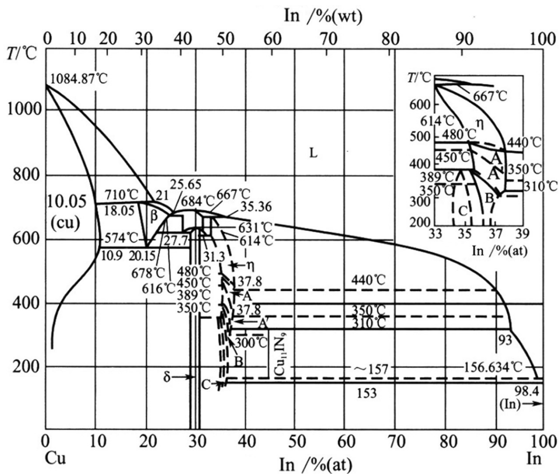
Fig. S1 Cu-In phase diagram.
