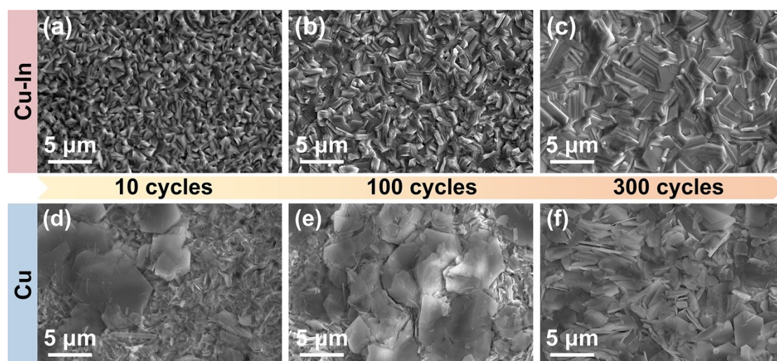
Fig. S5 SEM images of the deposited Cu–In (a–c) and Cu (d–f) electrodes after cycling 10, 100, and 300 times in the asymmetric battery.
