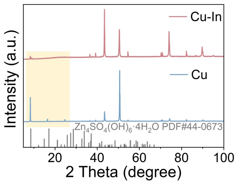
Fig. S6 XRD patterns after cycling 10 cycles in the asymmetric battery.
