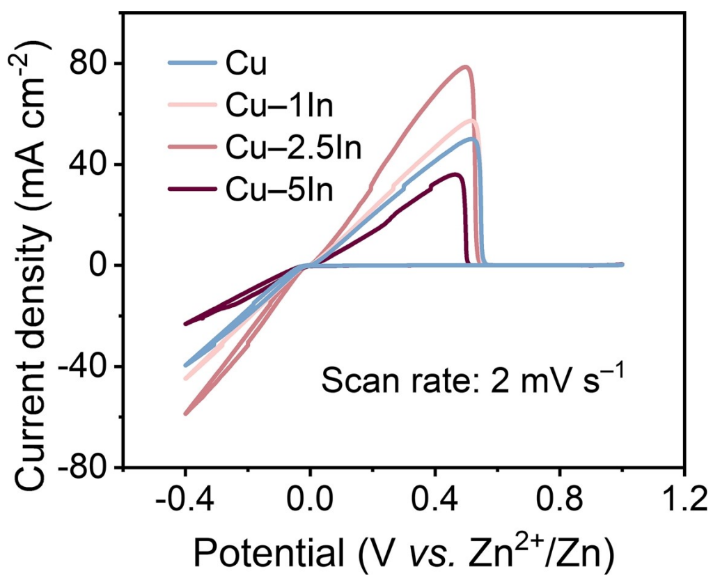
Fig. S3 CV curves of asymmetric cells.
