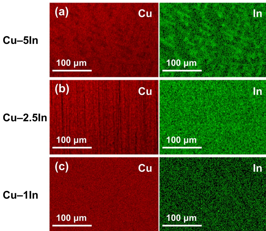
Fig. S2 EDS mapping of three Cu-In alloy and pure Cu.
