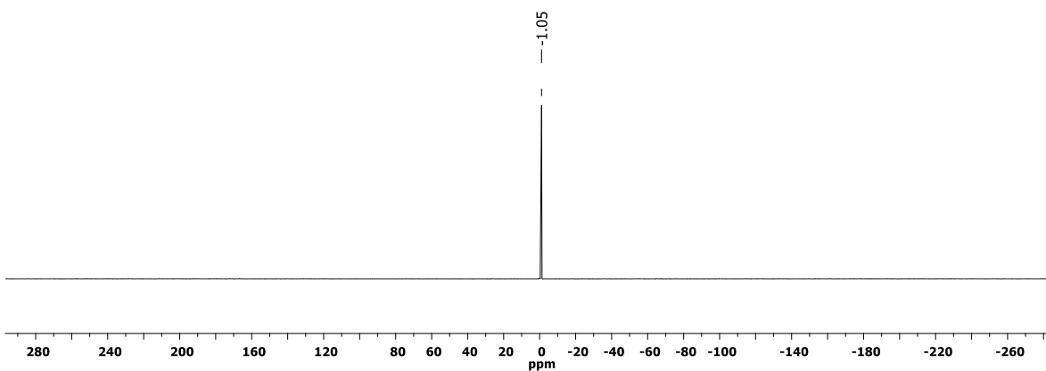
Figure S57 ^{31}\text{P}\{^1\text{H}\} NMR spectrum of 3ae ( \text{CDCl}_3 , 300 K).
