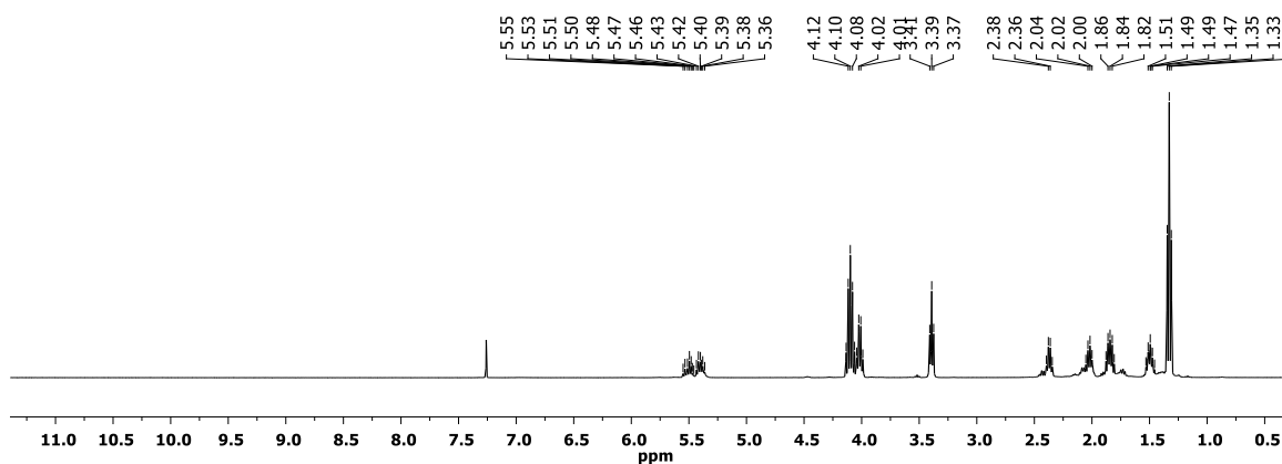
Figure S62 1 H NMR spectrum of 3ag (CDCl 3 , 300 K).
