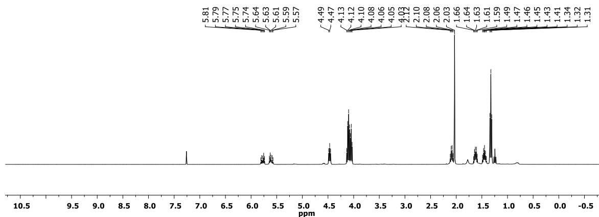
Figure S41 1 H NMR spectrum of 2ah (CDCl 3 , 300 K).
