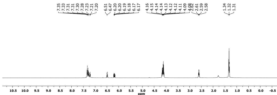
Figure S44 1 H NMR spectrum of 3aa (CDCl 3 , 300 K).
