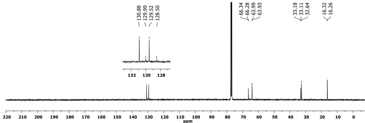
Figure S49 ^{13}\text{C}\{^1\text{H}\} NMR spectrum of 3ab ( \text{CDCl}_3 , 300 K).
