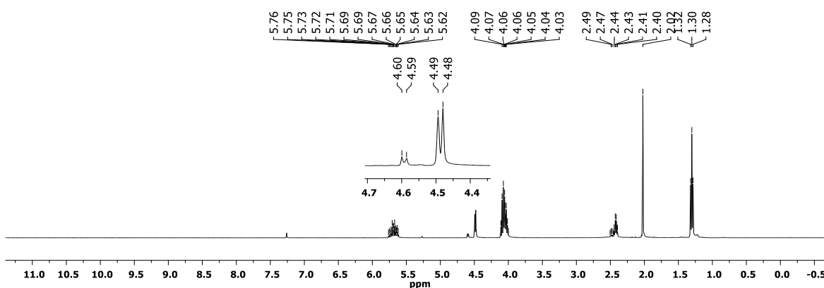
Figure S56 ^1\text{H} NMR spectrum of 3ae ( \text{CDCl}_3 , 300 K).
