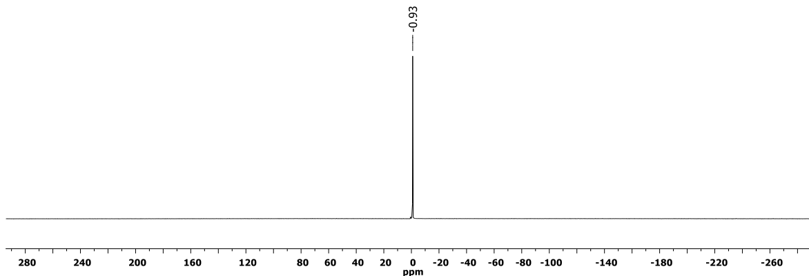
Figure S45 ^{31}\text{P}\{^1\text{H}\} NMR spectrum of 3aa ( \text{CDCl}_3 , 300 K).
