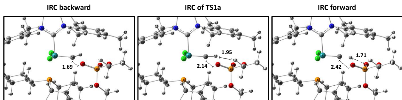
Figure S76 The intrinsic reaction coordinate (IRC) profile for the molecular transformation of TS1a at the M06L/def2-SVP level of theory; Optimized geometries of the transition states ( TS1a ) with distances in Å.
