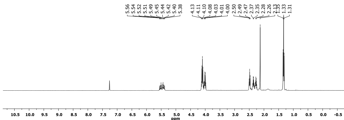
Figure S53 1 H NMR spectrum of 3ad (CDCl 3 , 300 K).
