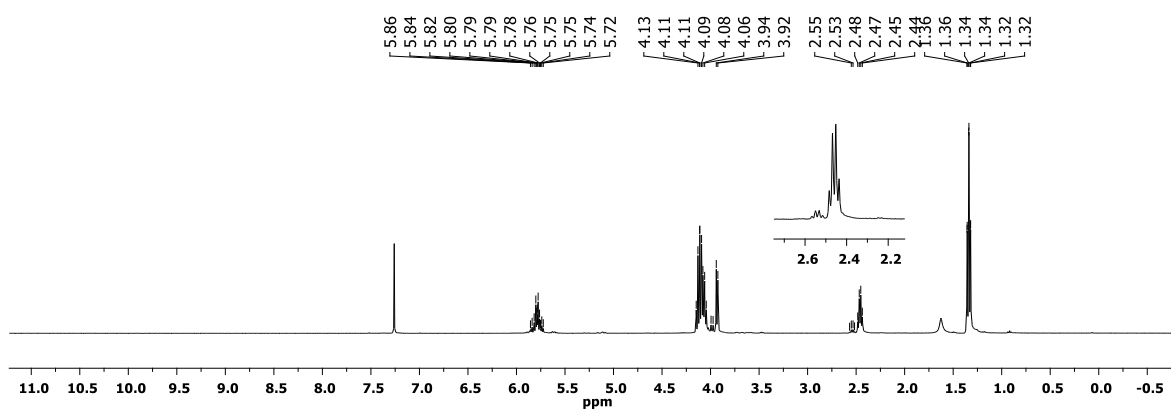
Figure S47 ^1\text{H} NMR spectrum of 3ab ( \text{CDCl}_3 , 300 K).
