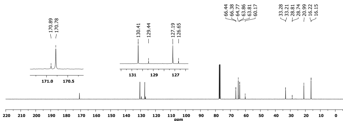
Figure S58 ^{13}\text{C}\{^1\text{H}\} NMR spectrum of 3ae ( \text{CDCl}_3 , 300 K).
