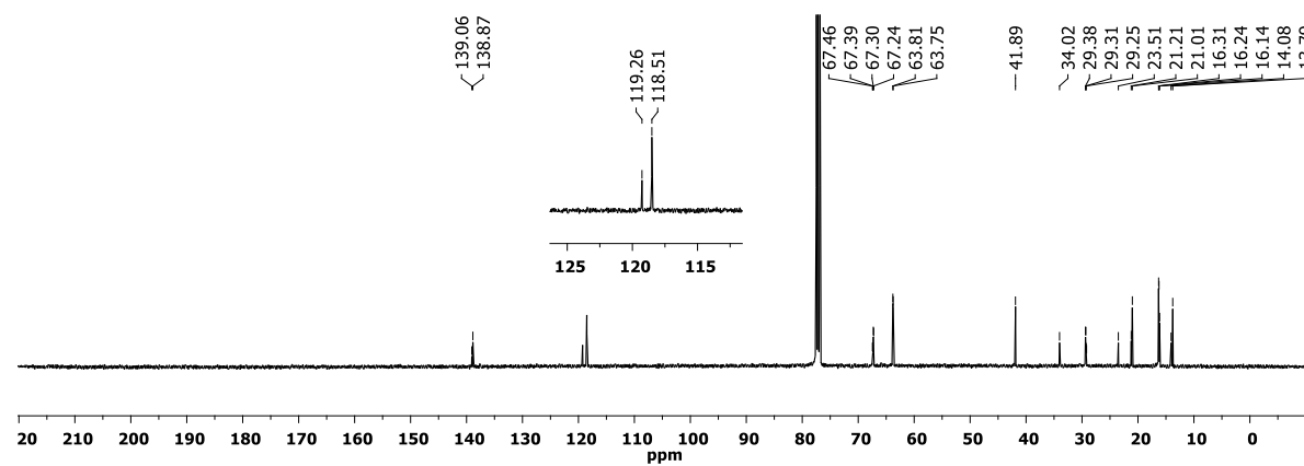
Figure S61 13 C{ 1 H} NMR spectrum of 3af (CDCl 3 , 300 K).
