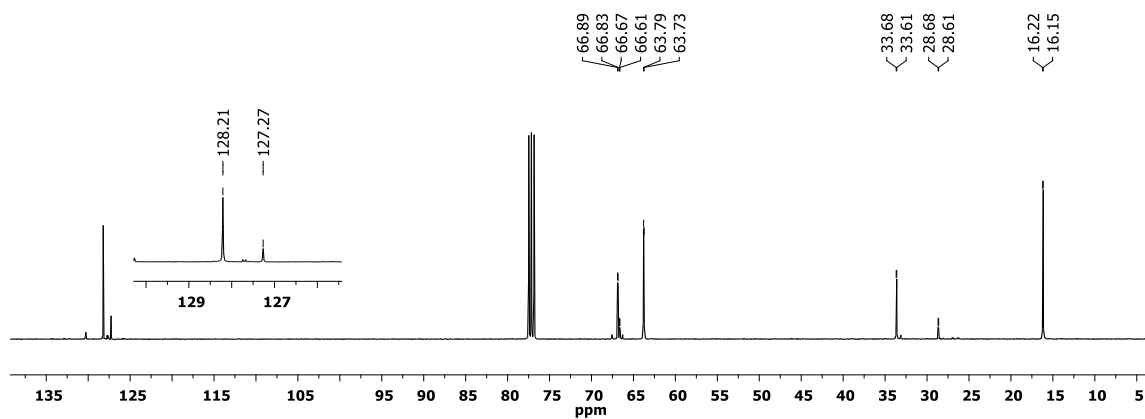
Figure S73 ^{13}\text{C}\{^1\text{H}\} NMR spectrum of dimer 3a (CDCl 3 , 300 K).
