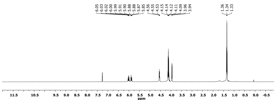
Figure S23 1 H NMR spectrum of 2ab ( \text{CDCl}_3 , 300 K).
