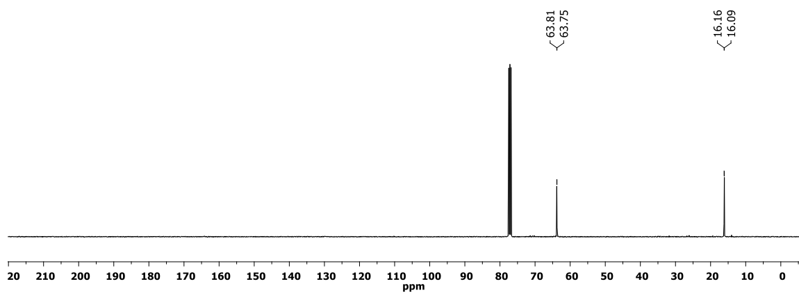
Figure S19 ^{13}\text{C}\{^1\text{H}\} NMR spectrum of 5 ( \text{CDCl}_3 , 300 K).
