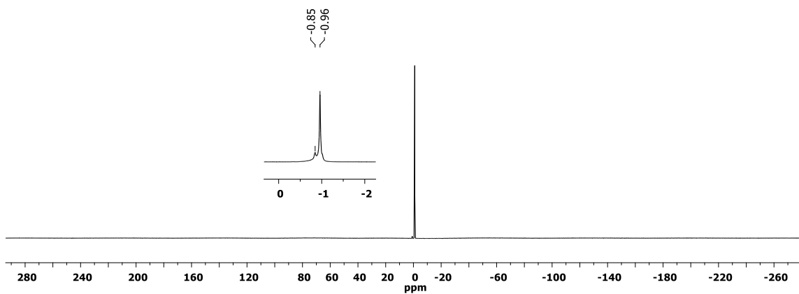
Figure S66 ^{31}\text{P}\{^1\text{H}\} NMR spectrum of 3ah (CDCl 3 , 300 K).
