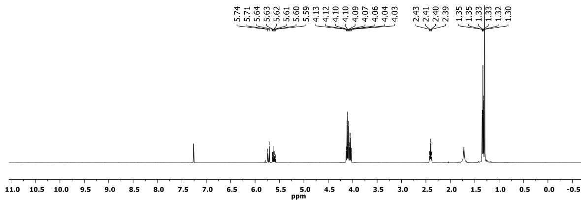
Figure S50 ^1\text{H} NMR spectrum of 3ac ( \text{CDCl}_3 , 300 K).
