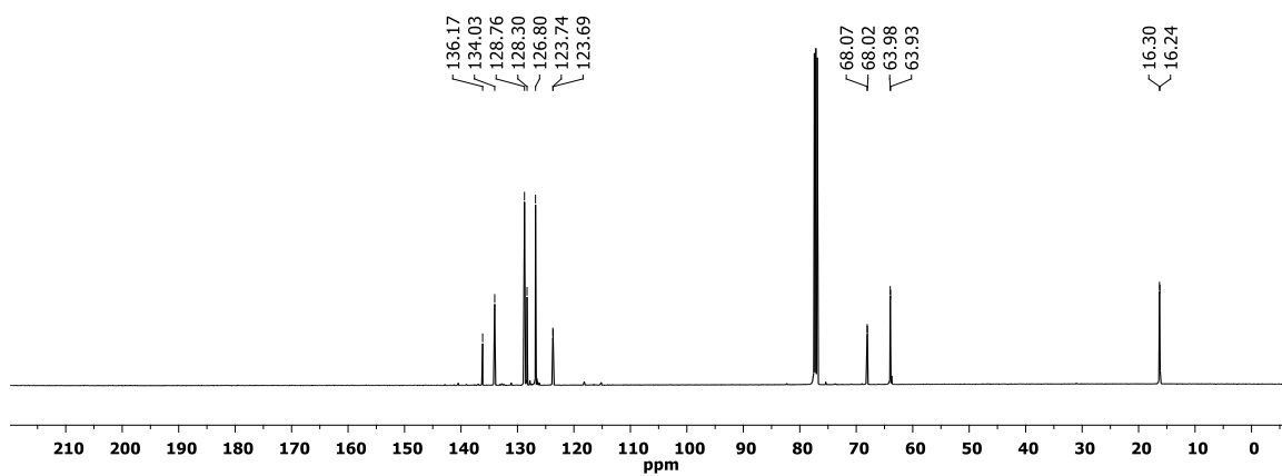
Figure S22 13 C{ 1 H} NMR spectrum of 2aa (CDCl 3 , 300 K).
