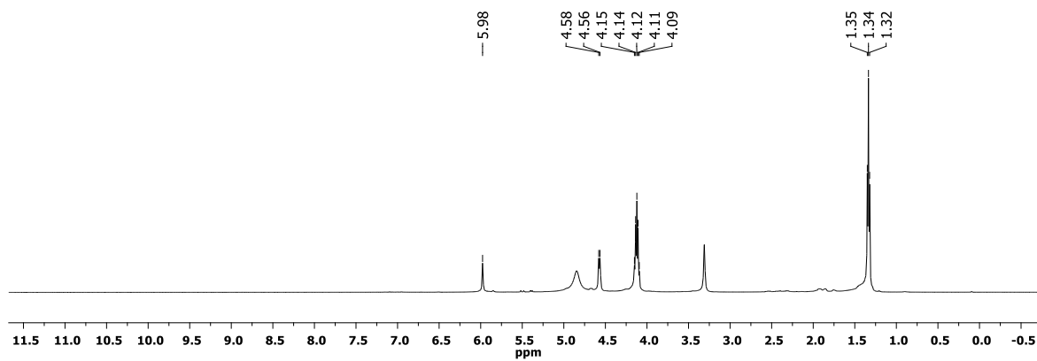
Figure S68 ^1\text{H} NMR spectrum of dimer 2a ( \text{CD}_3\text{OD} , 300 K).
