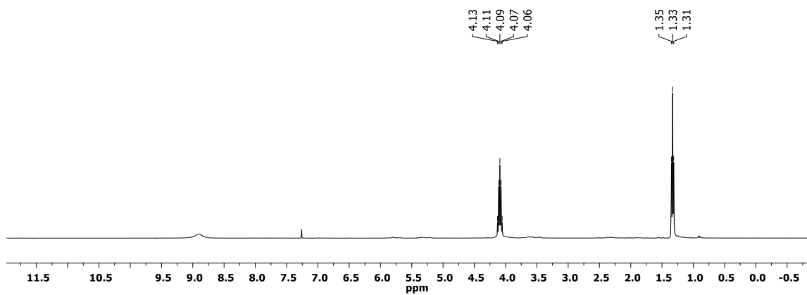
Figure S17 ^1\text{H} NMR spectrum of 5 ( \text{CDCl}_3 , 300 K).
