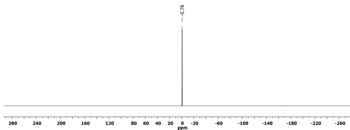
Figure S21 31 P{ 1 H} NMR spectrum of 2aa (CDCl 3 , 300 K).
