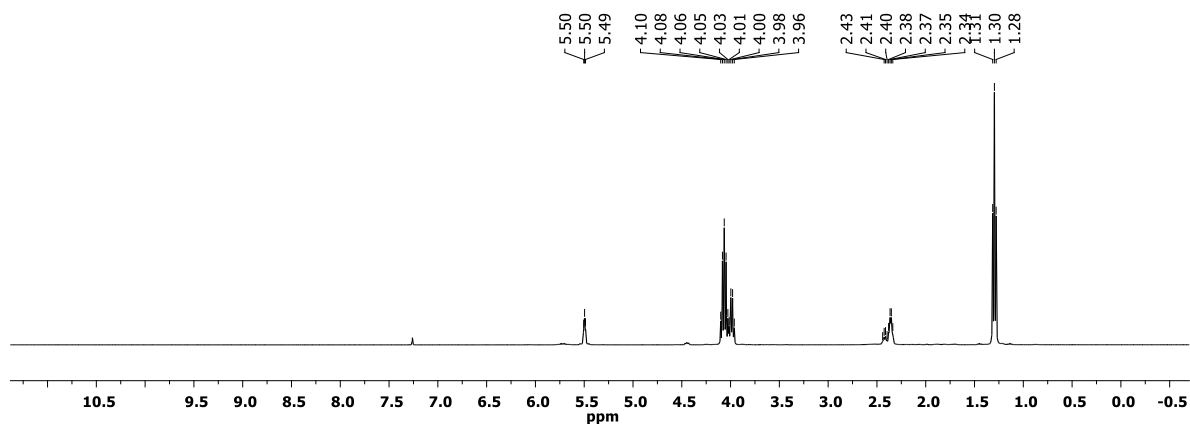
Figure S71 1 H NMR spectrum of dimer 3a ( \text{CDCl}_3 , 300 K).
