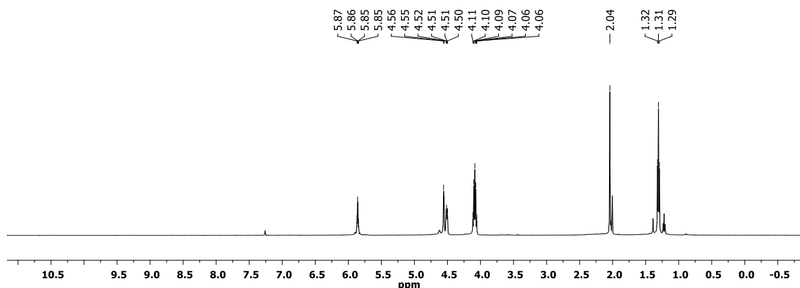
Figure S32 1 H NMR spectrum of 2ae ( \text{CDCl}_3 , 300 K).
