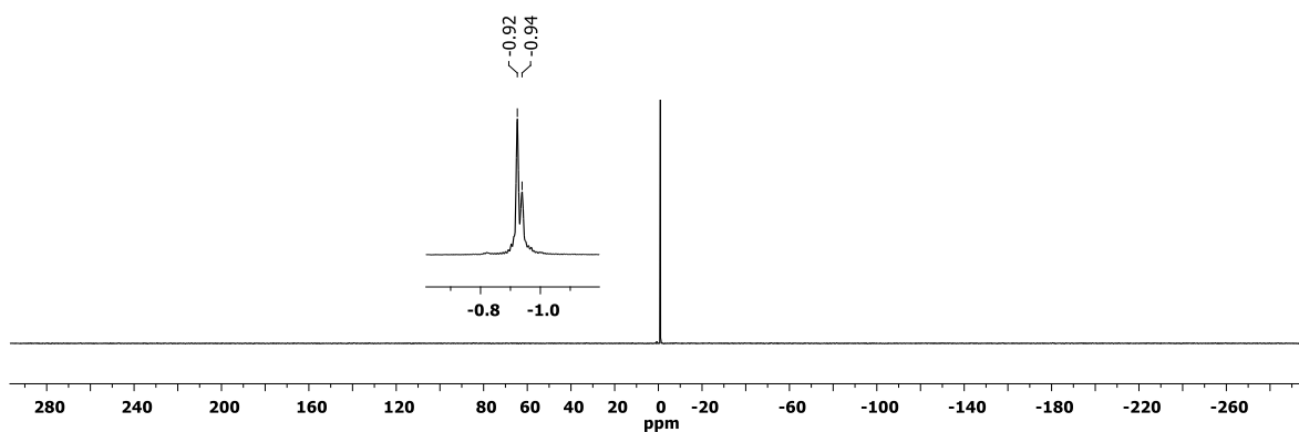
Figure S60 31 P{ 1 H} NMR spectrum of 3af (CDCl 3 , 300 K).
