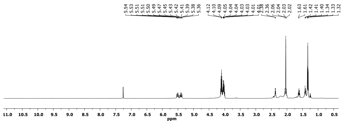
Figure S65 ^1\text{H} NMR spectrum of 3ah (CDCl 3 , 300 K).
