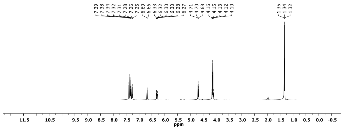
Figure S20 1 H NMR spectrum of 2aa (CDCl 3 , 300 K).
