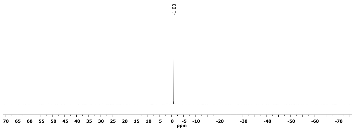
Figure S72 ^{31}\text{P}\{^1\text{H}\} NMR spectrum of dimer 3a (CDCl 3 , 300 K).
