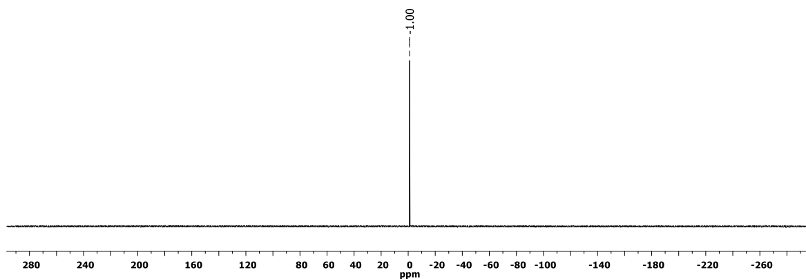
Figure S48 ^{31}\text{P}\{^1\text{H}\} NMR spectrum of 3ab ( \text{CDCl}_3 , 300 K).
