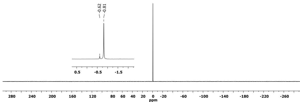
Figure S42 31 P{ 1 H} NMR spectrum of 2ah (CDCl 3 , 300 K).
