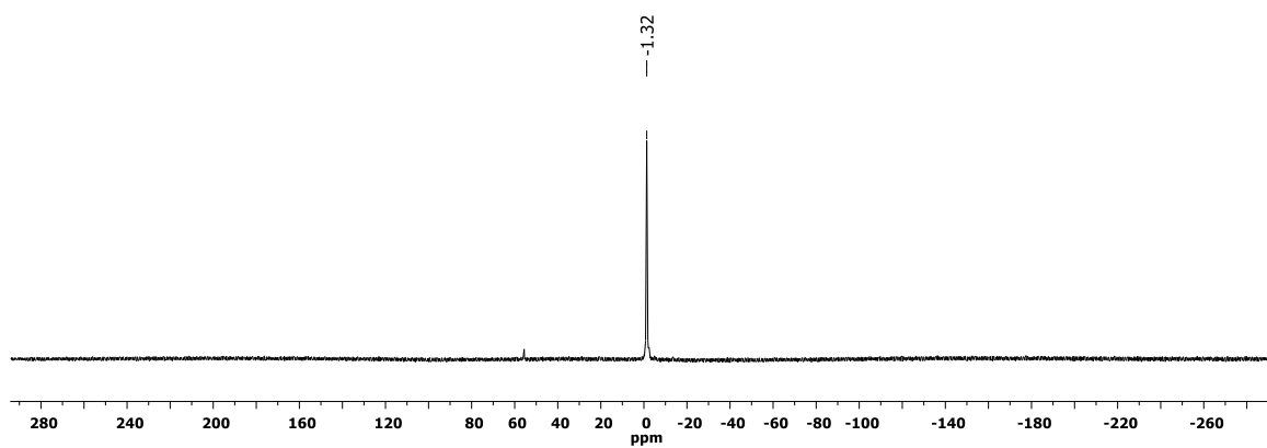
Figure S69 ^{31}\text{P}\{^1\text{H}\} NMR spectrum of dimer 2a ( \text{CD}_3\text{OD} , 300 K).
