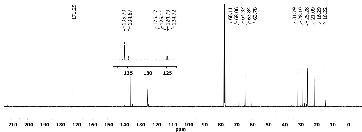
Figure S43 13 C{ 1 H} NMR spectrum of 2ah (CDCl 3 , 300 K).
