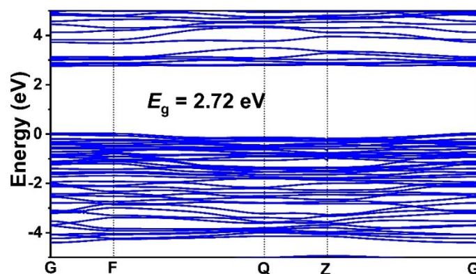
Fig. S1 Electronic band structure of PBE calculation
