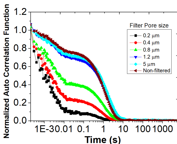
Figure S1: Normalised DLS autocorrelation functions for glycine solutions at 25°C with 1.5 supersaturation, filtered with PES of various pore sizes, as well as non-filtered.
