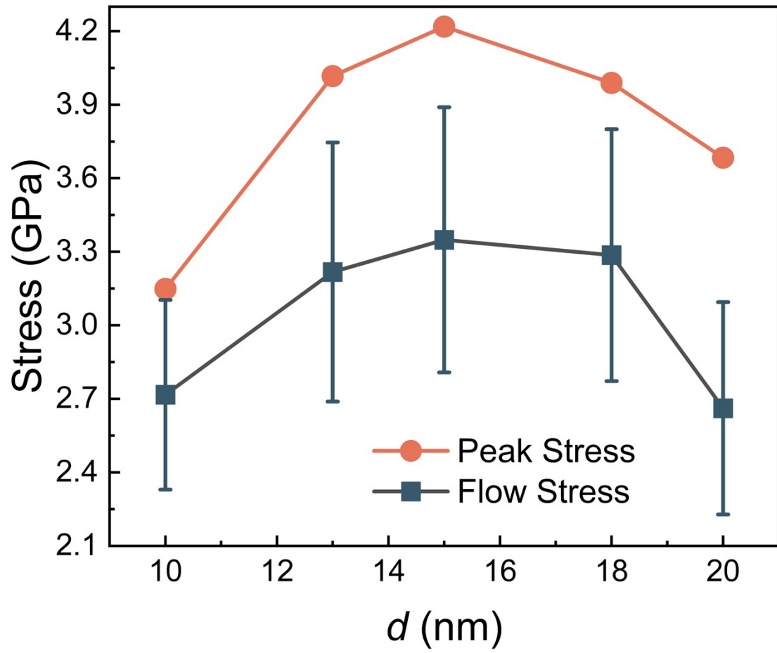
Fig. S1 Variation of peak and average flow stress of CoCrNi with d at \lambda = 5.54 nm.
