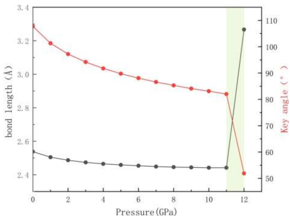
Fig. S1 Relationship between Zn-Se bond length and Zn-Se-Zn bond angle with pressure
