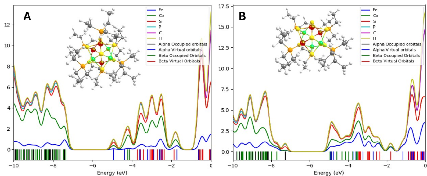
Figure S6. Partial density of States (PDOS) for (A) [\text{Co}_3\text{Fe}_3\text{S}_8\text{L}_6]^+ and (B) [\text{Co}_3\text{Fe}_3\text{S}_8\text{L}_5]^+ at the PBE0-D3/CEP-31G level of theory on the optimized geometry. FWHM = 0.30 eV
