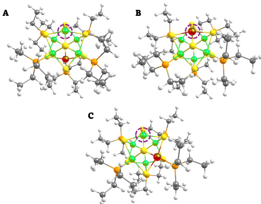
Figure S2. Symmetry isomers of undercoordinated \text{Co}_5\text{Fe NC} (A) Co – trans, (B) Fe, and (C) Co – cis. The circle shows the metal where the ligand was removed. (Color scheme: green = Co, red = Fe, yellow = S, orange = P, grey = C, white = H)
