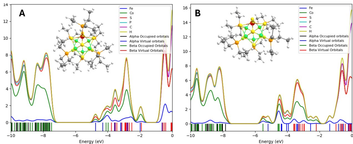
Figure S5. Partial density of States (PDOS) for (A) [\text{Co}_5\text{FeS}_8\text{L}_6]^+ and (B) [\text{Co}_5\text{FeS}_8\text{L}_5]^+ at the PBE0-D3/CEP-31G level of theory on the optimized geometry. FWHM = 0.30 eV
