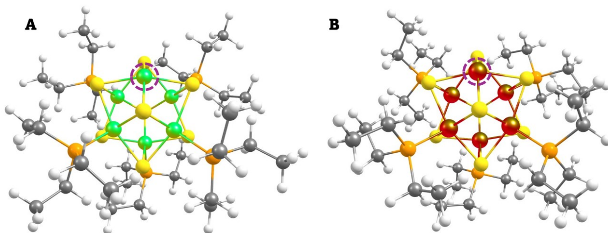
Figure S1. Symmetry isomers of undercoordinated (A) Co 6 and (B) Fe 6 NCs. The circle shows the metal where the ligand was removed. (Color scheme: green = Co, red = Fe, yellow = S, orange = P, grey = C, white = H)
