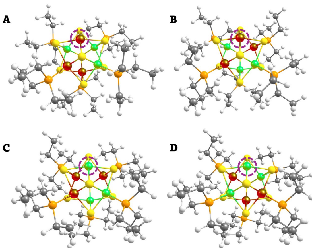
Figure S3. Symmetry isomers of undercoordinated \text{Co}_3\text{Fe}_3 NC (A) Fe – 1 (B) Fe – 2 (C) Co – 1 (D) Co – 2 . The circle shows the metal where the ligand was removed. (Color scheme: green = Co, red = Fe, yellow = S, orange = P, grey = C, white = H)
