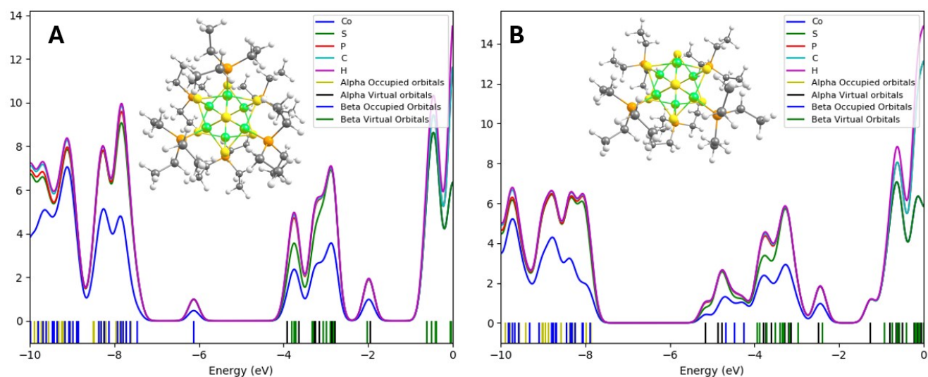
Figure S4. Partial density of States (PDOS) for (A) [Co 6 S 8 L 6 ] + and (B) [Co 6 S 8 L 5 ] + at the PBE0-D3/CEP-31G level of theory on the optimized geometry. FWHM = 0.30 eV
