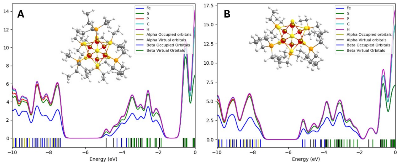
Figure S7. Partial density of States (PDOS) for (A) [\text{Fe}_6\text{S}_8\text{L}_6]^+ and (B) [\text{Fe}_6\text{S}_8\text{L}_5]^+ at the PBE0-D3/CEP-31G level of theory on the optimized geometry. FWHM = 0.30 eV
