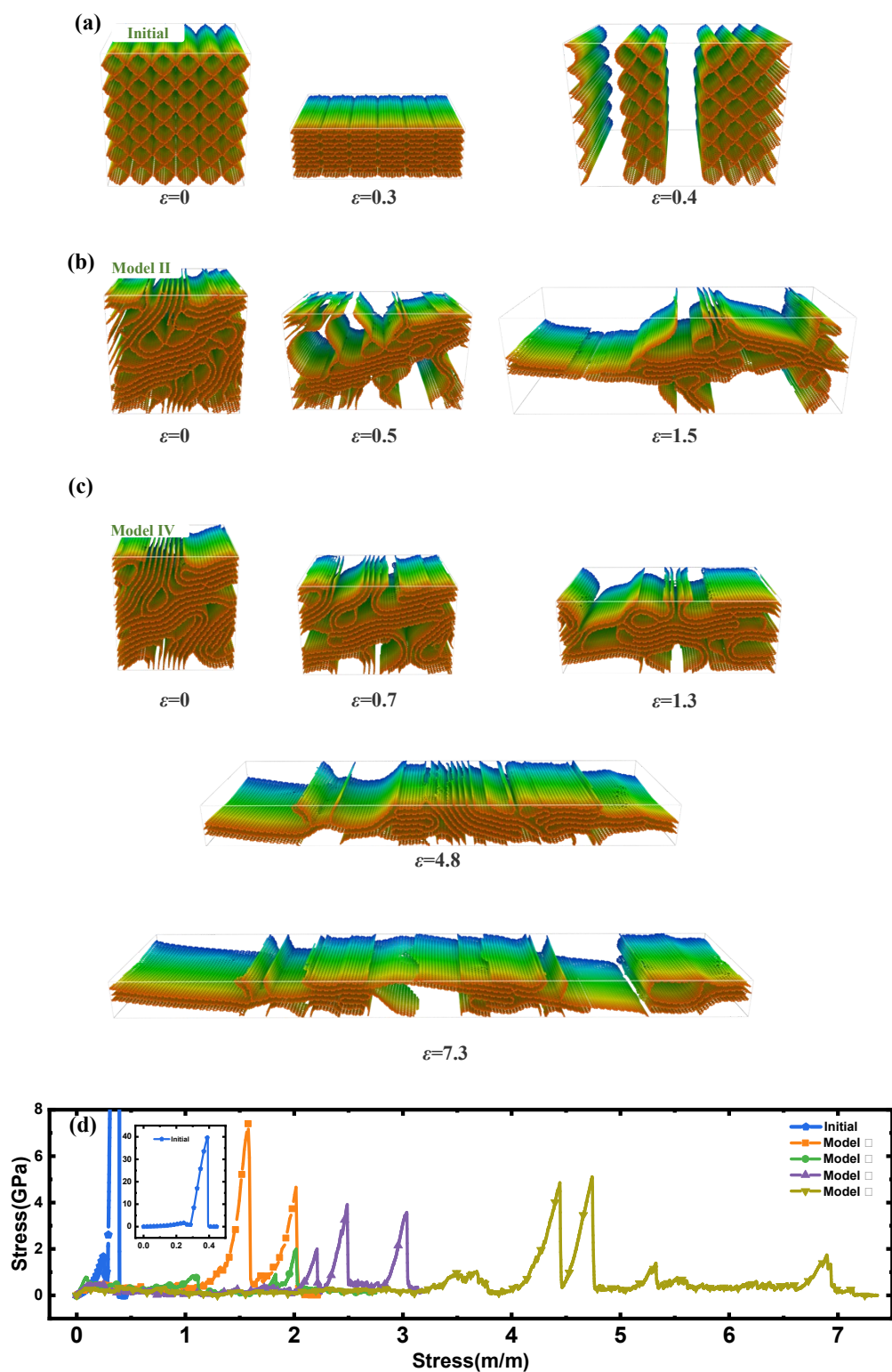
Figure S2. (a)-(c) Snapshots of others CNT array under compression loading. (d) The tensile stress-strain curves of all the Models.
