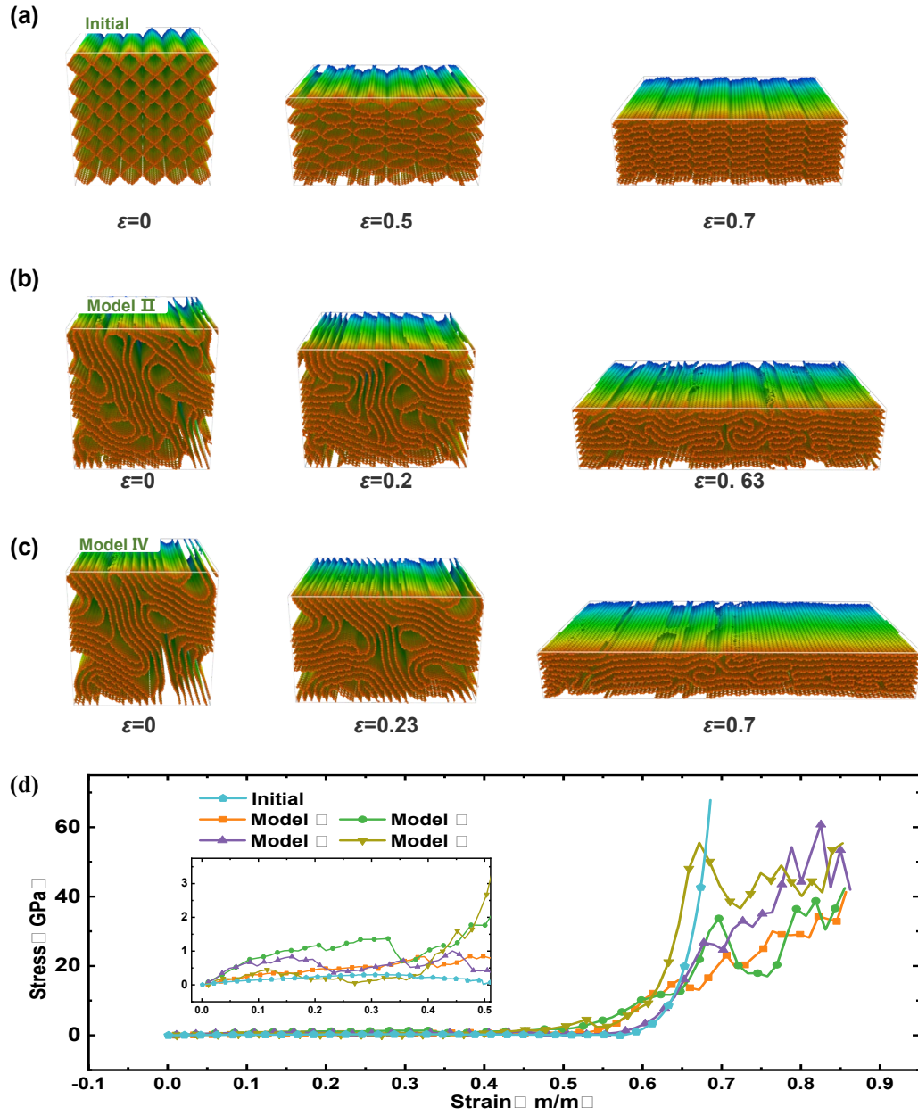
Figure S1. (a)-(c) Snapshots of others CNT array under compression loading. (d) The tensile stress-strain curves of all the Models.
