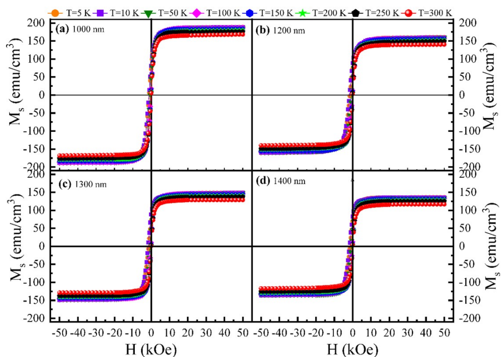
Fig. S2. M - H curves of the Fe nanocluster-assembled films with different thickness measured at different temperature: (a) 1000 nm, (b) 1200 nm, (c) 1300 nm, (d) 1400 nm.
