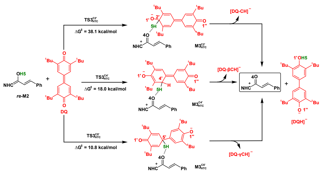
Scheme S2 The other possible HTC pathways for the oxidation process (energies in kcal/mol).
