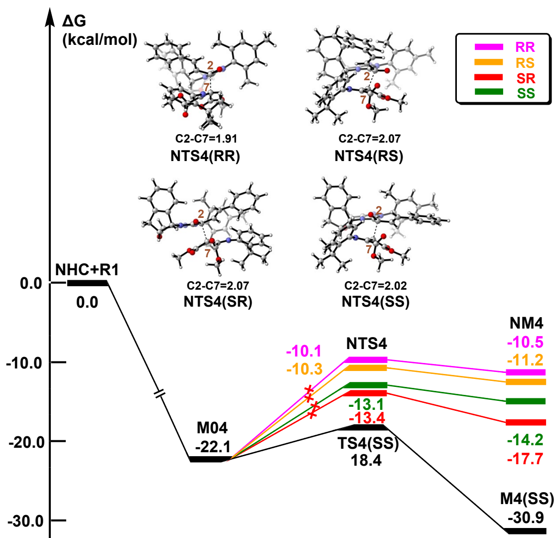
Fig. S8 Free energy profile for the C2-C7 bond formation pathway in the R2 and M3 addition reaction (distance in Å and energies in kcal/mol).
