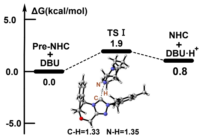
Fig. S1 The deprotonation of Pre-NHC by base (DBU) generating NHC (distance in Å and energies in kcal/mol).
