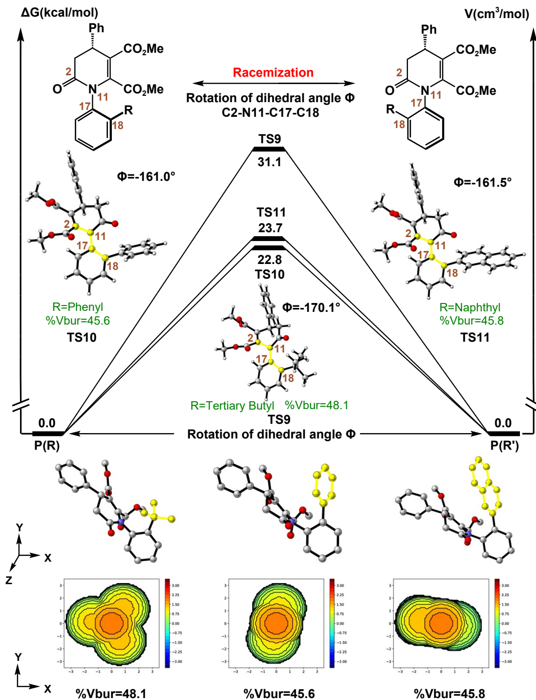
Fig. S10 Energy profiles and buried volume plot models involved in the racemization process.
