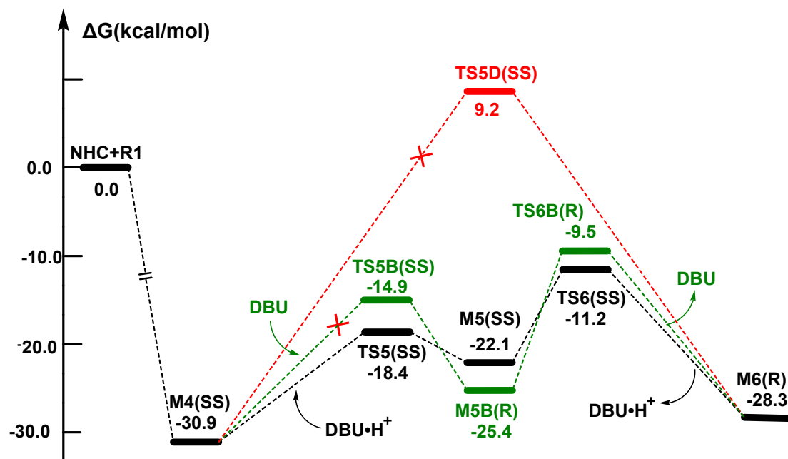
Fig. S7 Free energy profiles of possible mechanisms for M4 → M6 conversion (energies in kcal/mol).
