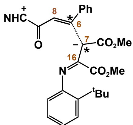
Fig. S5 Conformational search for TS4.
