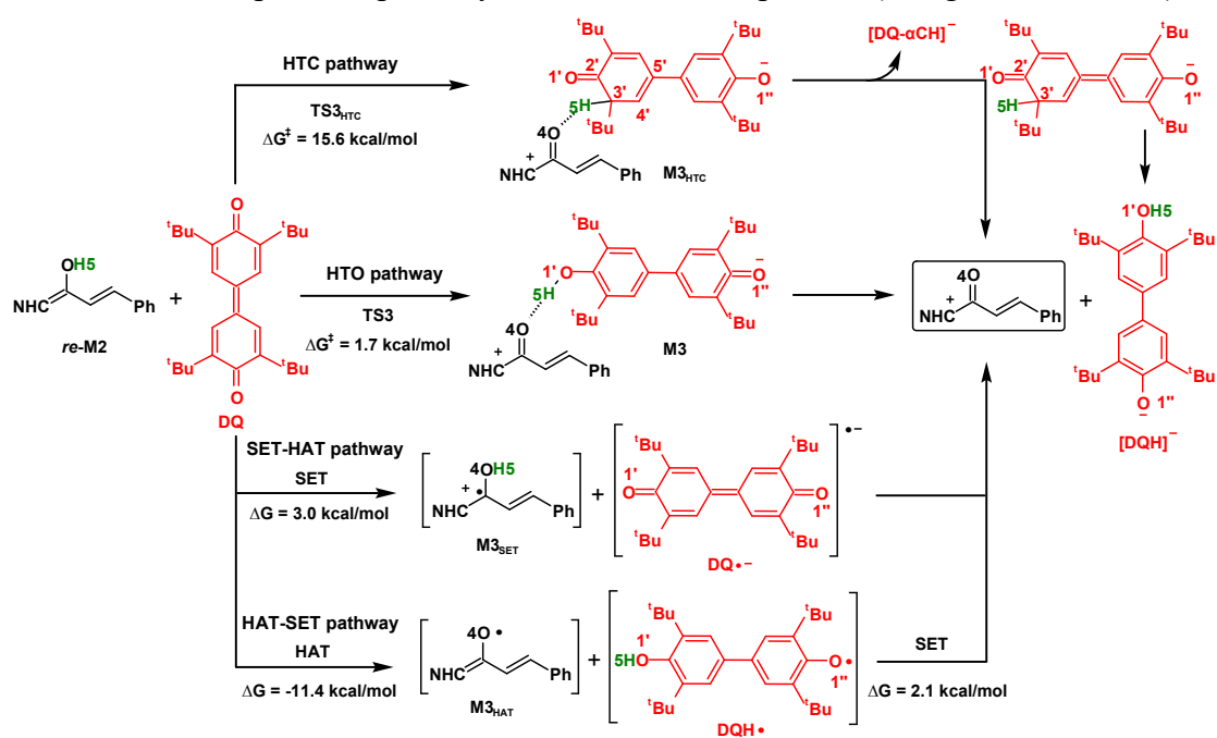
Scheme S1 Four possible pathways for the oxidation process (energies in kcal/mol).
