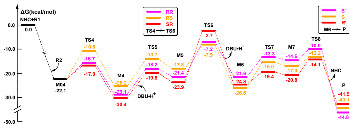
Fig. S6 Free energy profiles for transformation from intermediate M04 to product P (energies in kcal/mol).
