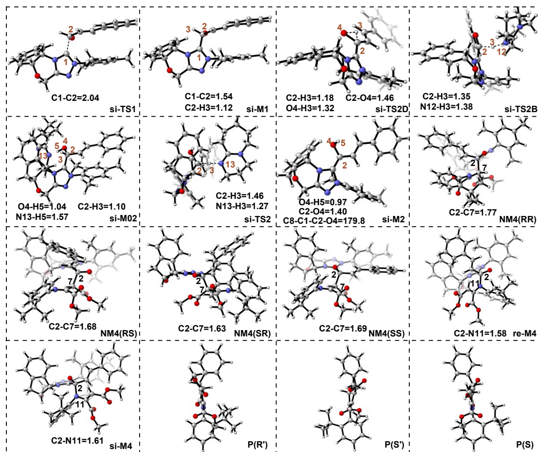
Fig. S3 Optimized geometries of transition states and intermediates (distance in Å).
