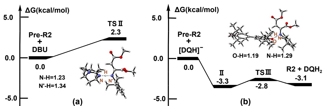
Fig. S2 The deprotonation of Pre-R2 by base generating R2 (distance in Å and energies in kcal/mol).
