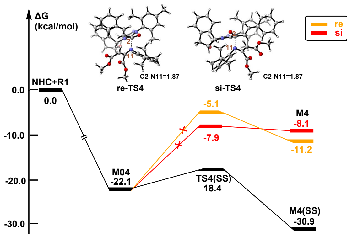
Fig. S9 Free energy profile for the C2-N11 bond formation pathway (distance in Å and energies in kcal/mol).
