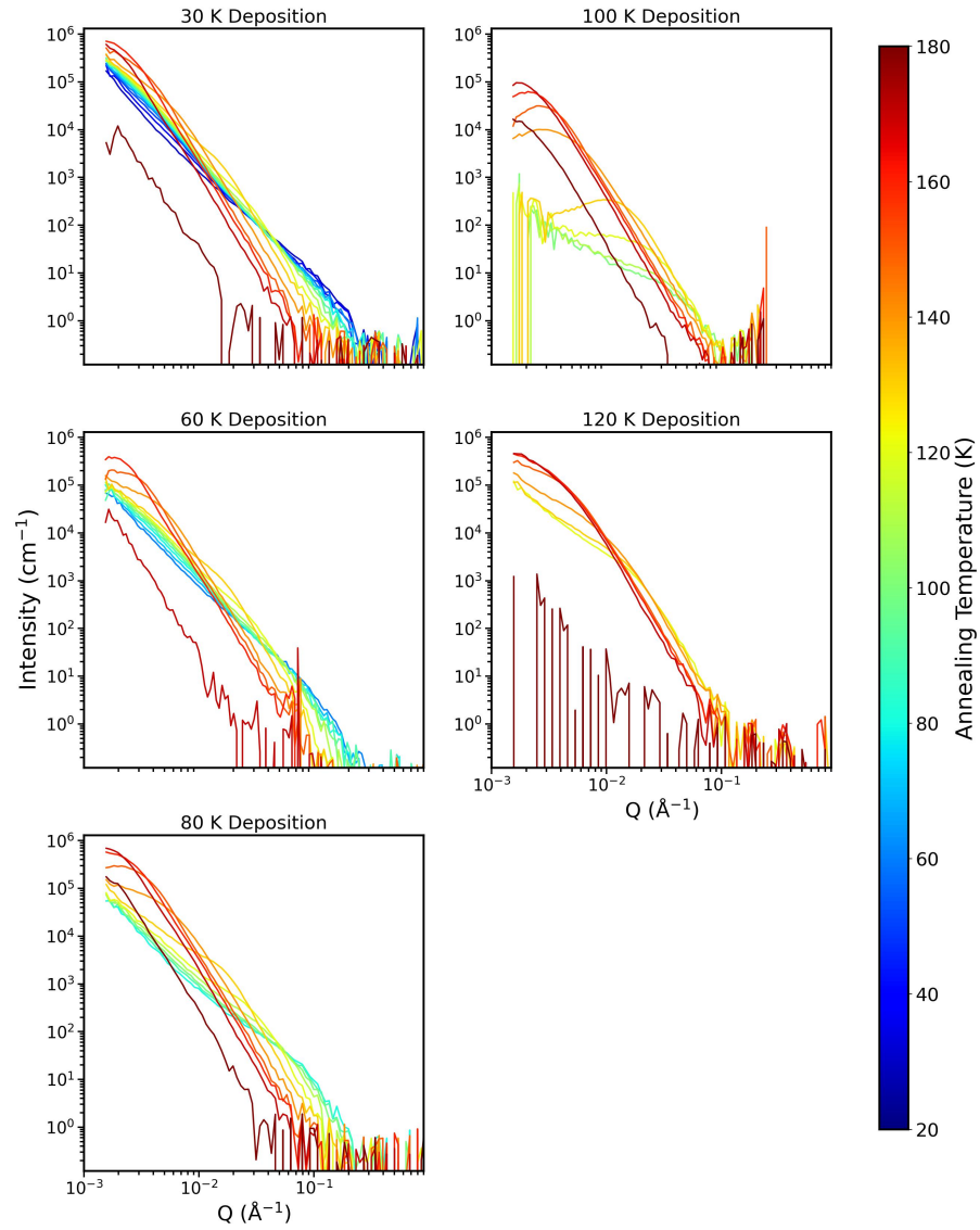
Figure S1: Intensity as a function of Q for the raw SANS2D data of every sample, with the respective deposition temperature written above the plots. Trace colours represent the annealing temperature shown by the colourbar on the right hand side.
