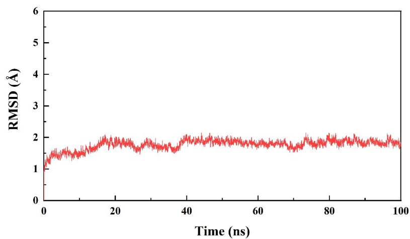
Figure S1. RMSD of completed CYP1B1 structure optimization.
