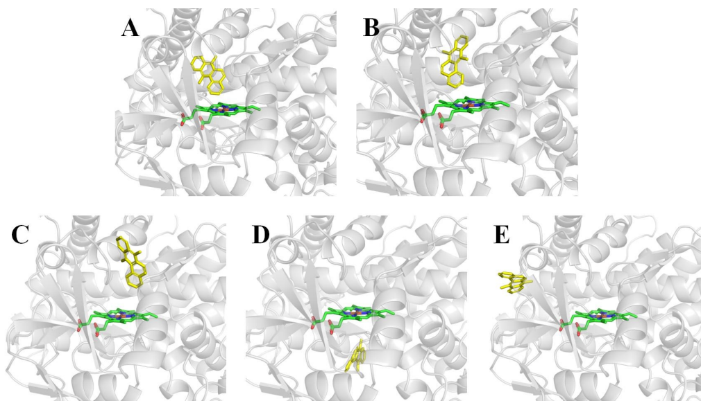
Figure S3. Representative conformations of the five DMBA-CYP1B1 docking poses
