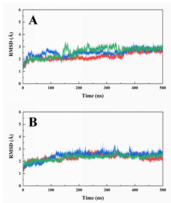
Figure S4. RMSDs of binding mode I (A) and mode II (B).
