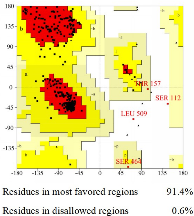
Figure S2. The Ramachandran plot and its detailed information calculated by SAVES.
