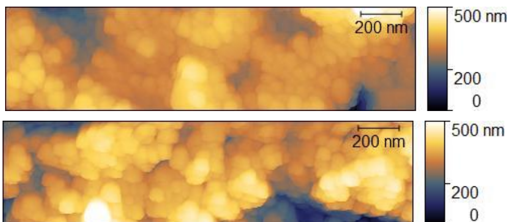
Figure S1- 2D AFM images of photoabsorbers: BTCF:Dy (a) and P25/BTCF:Dy (b).
